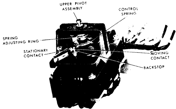
Fig. 19 (8034958) Four-Pole Induction Cylinder Unit Typical Of The Ohm Unit And Starting Unit In The Type GCXG51A Relay.
