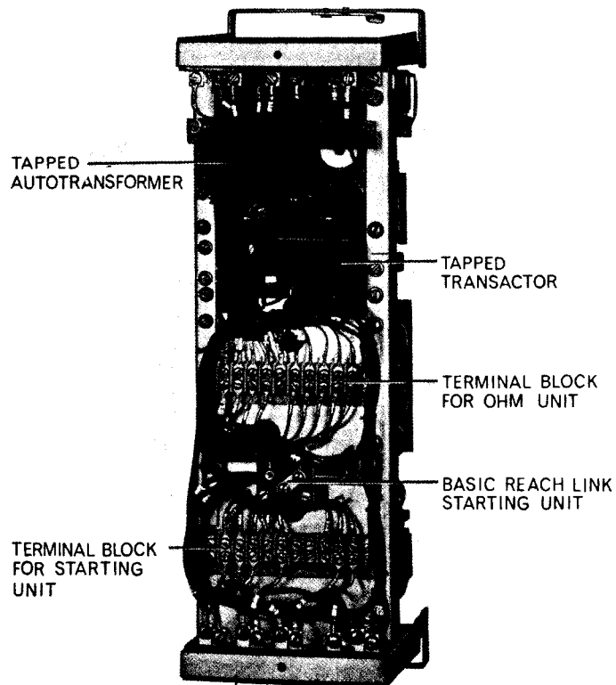
Fig. 2 (8035669) Type GCXG51A Relay Removed From Case. (Rear View)
