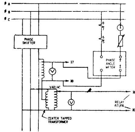
Fig. 14 (0178A9119-3) Test Circuit For The Ohm Unit Of The Type GCXG51A Relay. Using A Phase Shifter.
