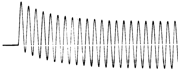
TYPICAL OFFSET FAULT CURRENT WAVE
