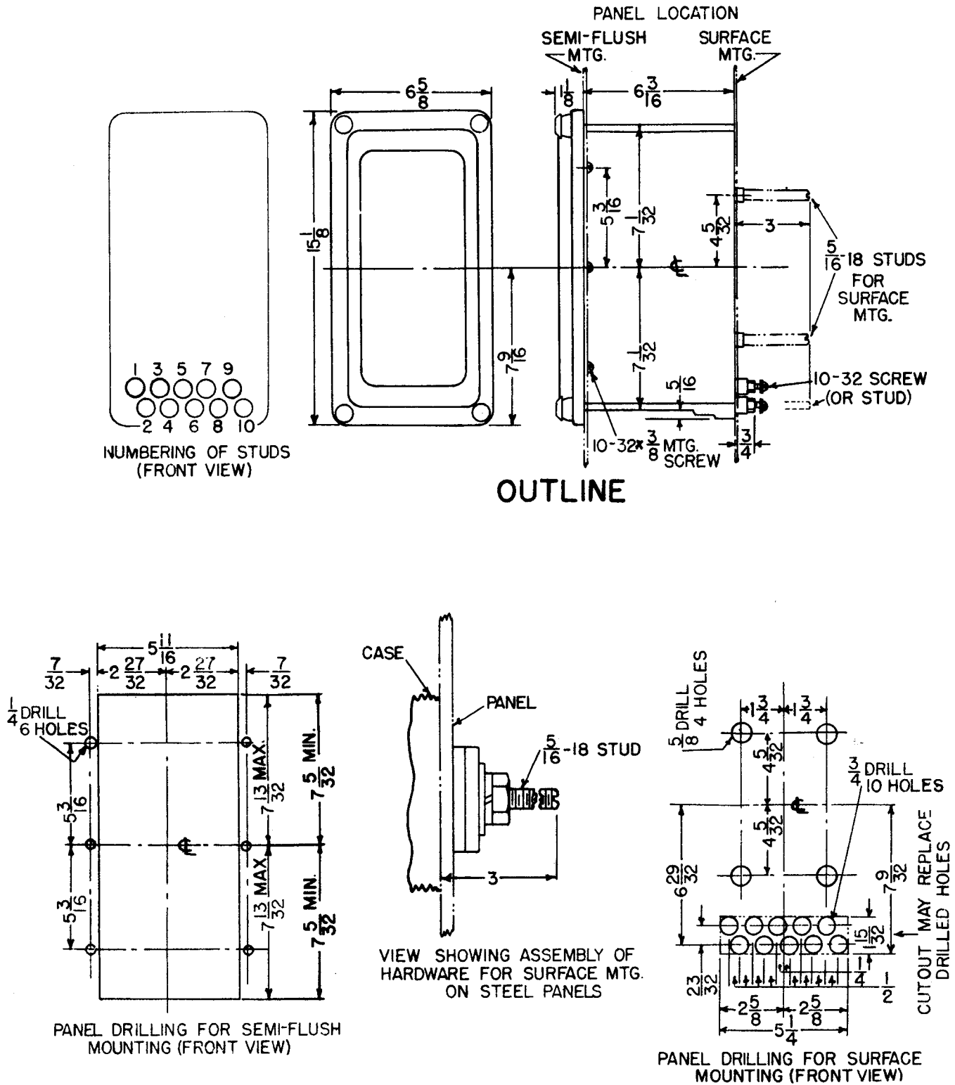
Fig. 12 (6209273-3) Outline And Panel Drilling Dimensions For Type BFC11A Relay.
