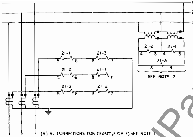
Figure 5 (0108B8983-1) External Connection Diagram for Type CEX57 Relays
