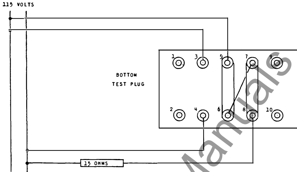
(A) POLARITY CHECK
