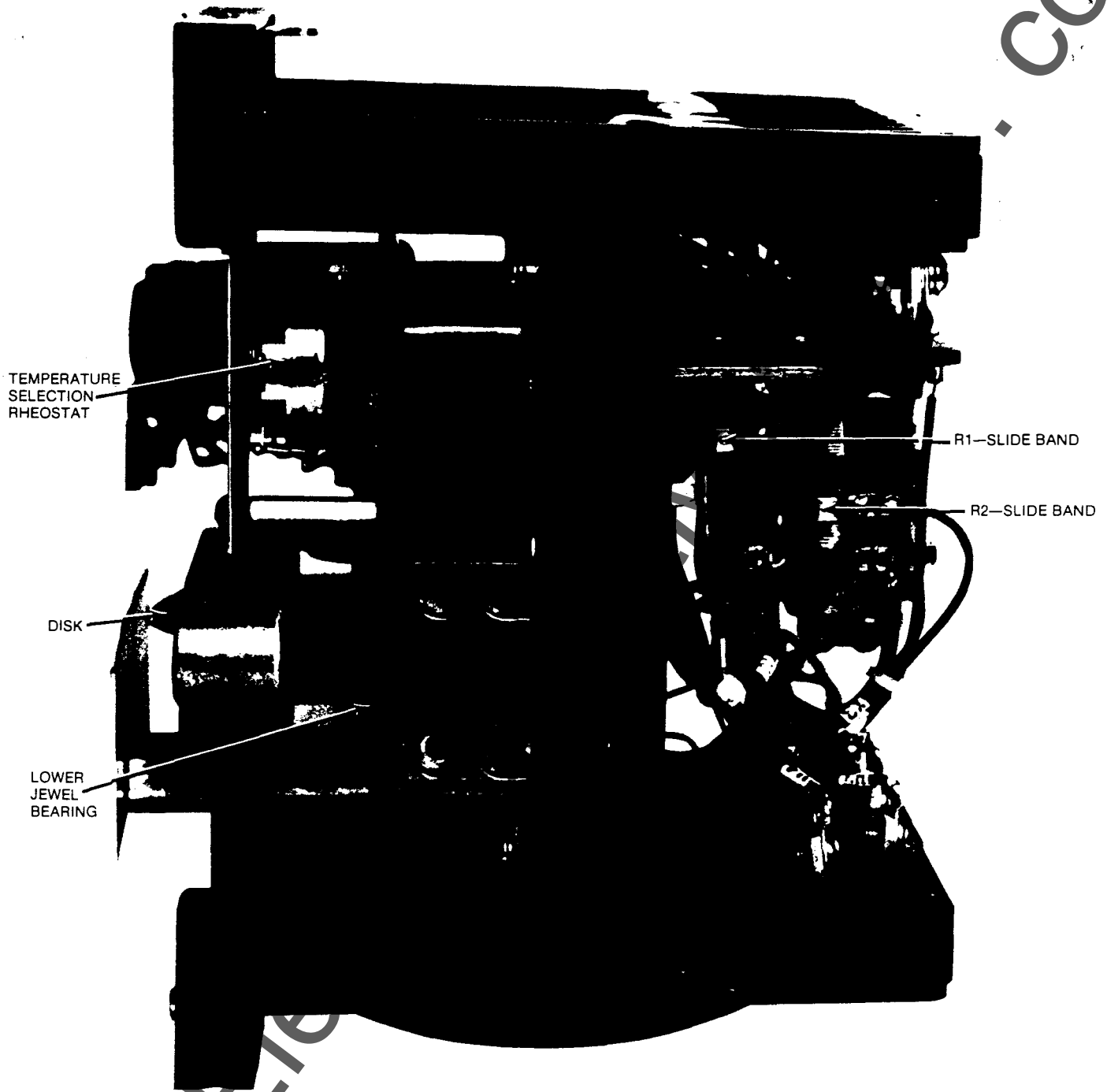
Figure 2 (050283-2) Type IRT51G and IRT51H Relay, Right Side View.
