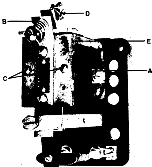
Fig. 3. IC2820-1754D relay
