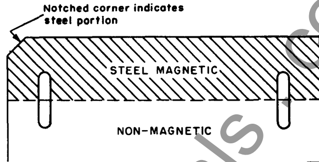
Fig. 4. Bimetal sliding shim used on IC2820-1754D relay
