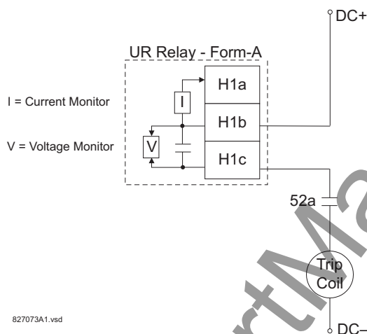
Figure 5-72: TRIP CIRCUIT EXAMPLE 1
