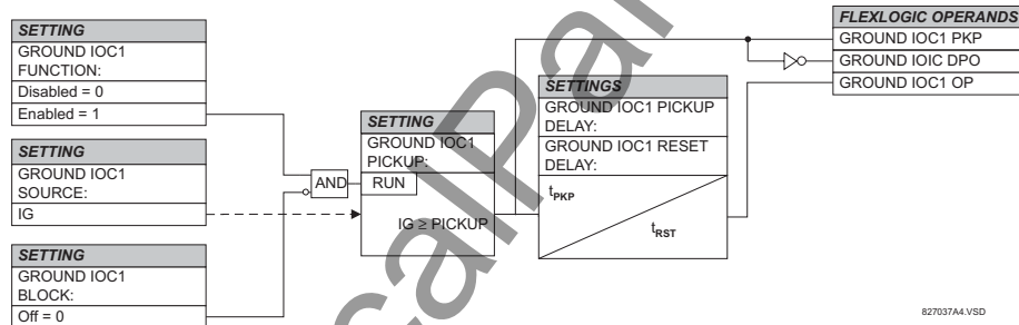
Figure 5-54: GROUND IOC1 SCHEME LOGIC
