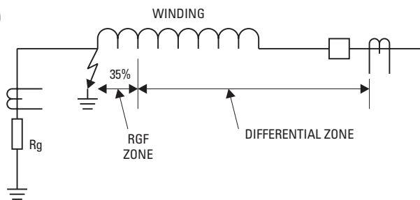
Figure 5-55: RGF AND PERCENT DIFFERENTIAL ZONES OF PROTECTION
