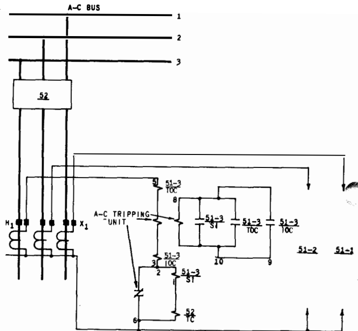
Fig. 6 External Connections of Three Type IAC51 Relays Used for 3-Phase Circuit Protection
