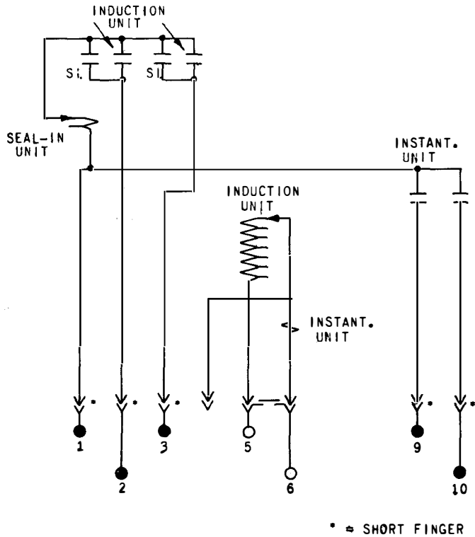
Fig. 17 Internal Connections for the Type IAC52B Relay (Front View)
