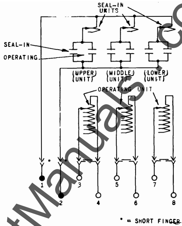
Fig. 14 Internal Connections for the Type IAC51D Relay (Front View)
