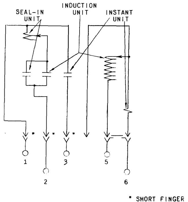
Fig. 12 Internal Connections for the Type IAC51B Relay (Front View)
