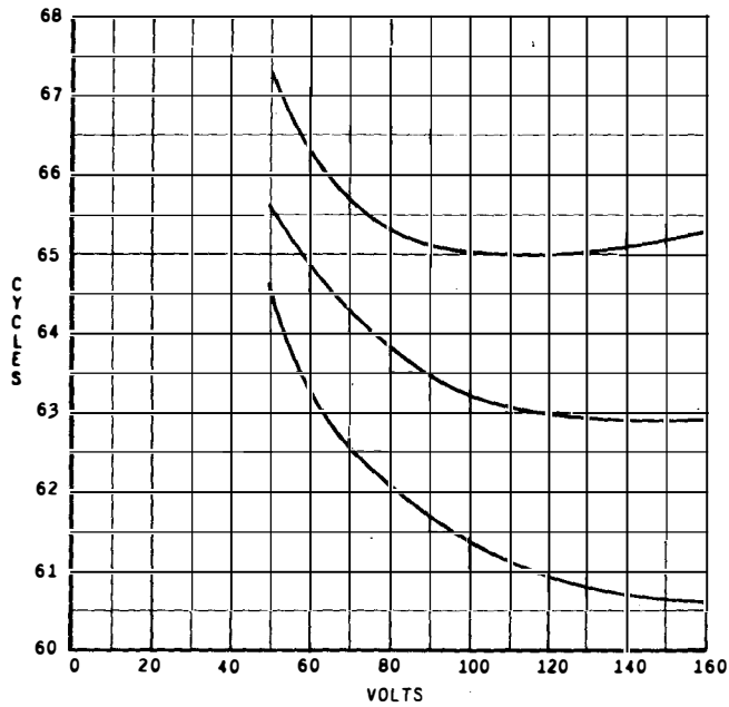
Fig. 3 Type IJF51A Relay, Voltage-Frequency Characteristics
