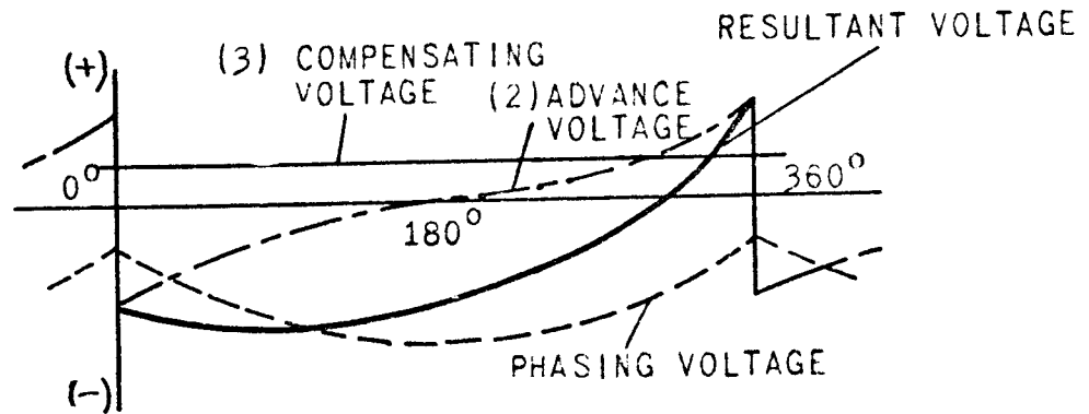
FIG B - COMPONENTS OF VOLTAGE THAT CONTROLS B WHEN VOLTAGES ARE UNBALANCED.
