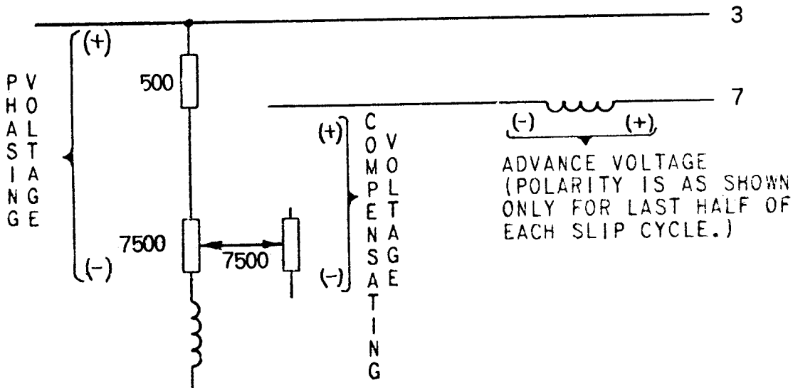
FIG. C - COMPONENTS OF VOLTAGE THAT CONTROLS B RELAY.
