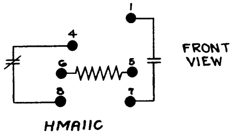
OUTLINE (FRONT & BACK CONNECTED RELAY)
