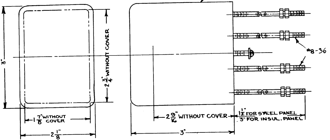
OUTLINE (FRONT & BACK CONNECTED RELAY)
