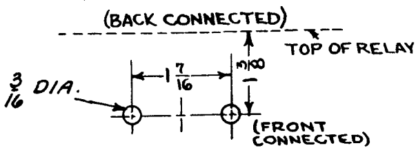
FIG 3 (K-6400440 [5]) OUTLINE, PANEL DRILLING DIMENSIONS AND INTERNAL CONNECTIONS FOR TYPE HMA11C AND HMA11D RELAY
