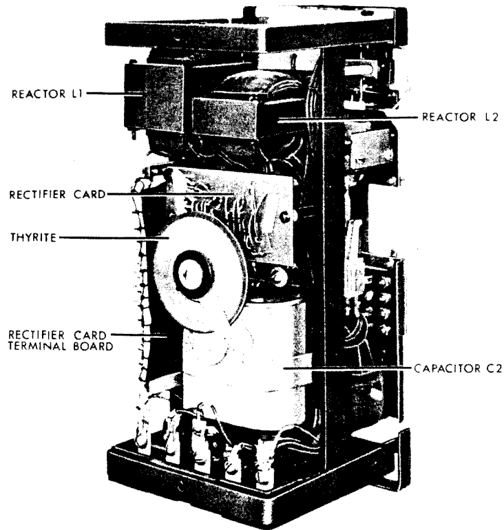
FIG. 4B (8042544) RELAY TYPE STD16C OUT OF CASE, APPROX 3/4 BACK VIEW (RIGHT SIDE)
