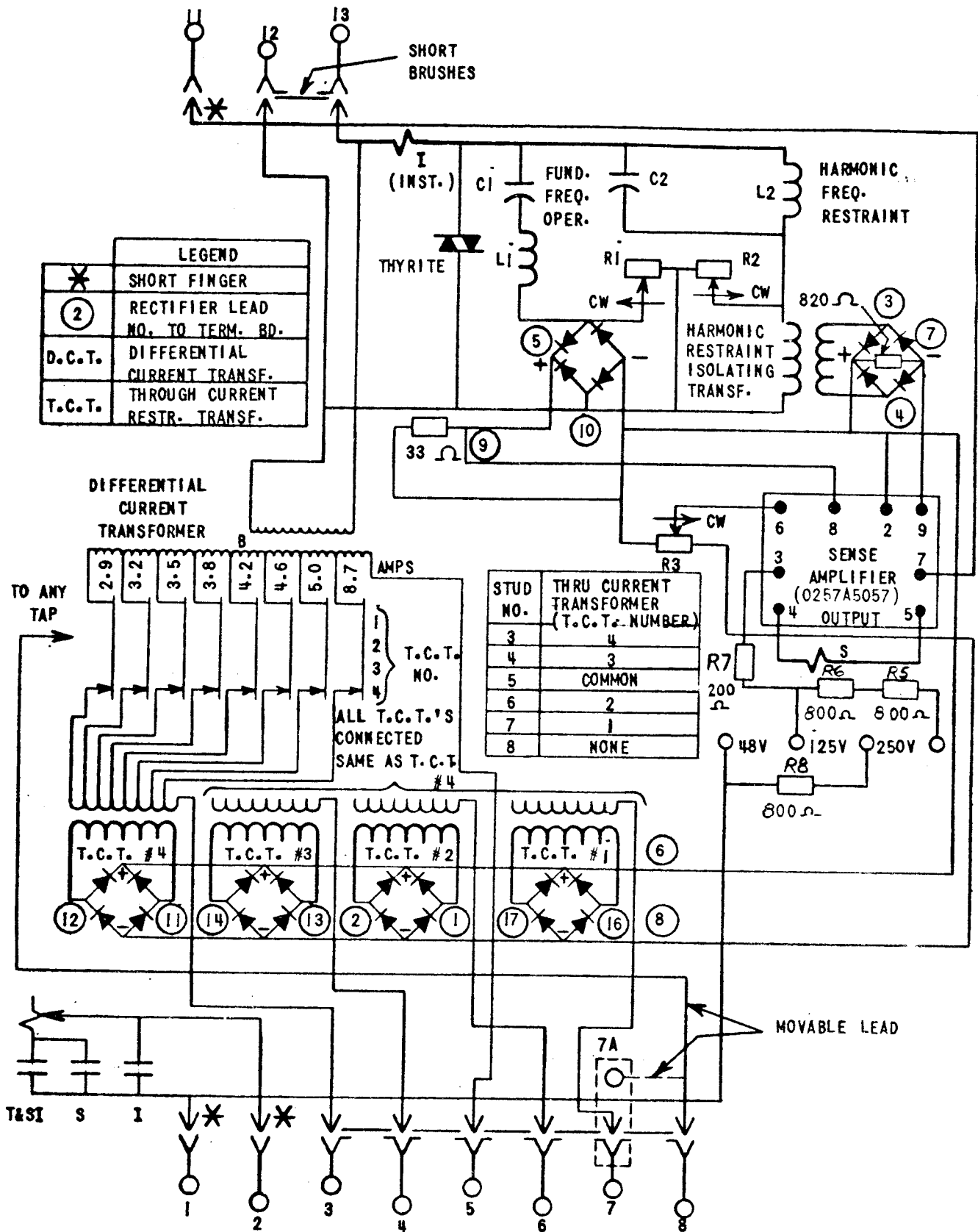
*Figure 1 (0257A5028 [2]) Internal Connections Diagram for the STD17C Relay (Front View)
