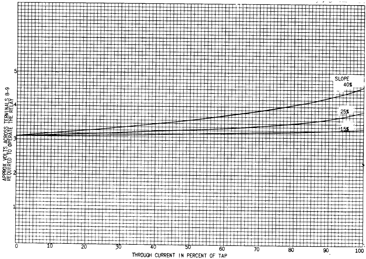
FIG. 16 (0178A8111-0) DIFFERENTIAL VOLTAGE OPERATING CHARACTERISTICS OF TYPE STD RELAY
