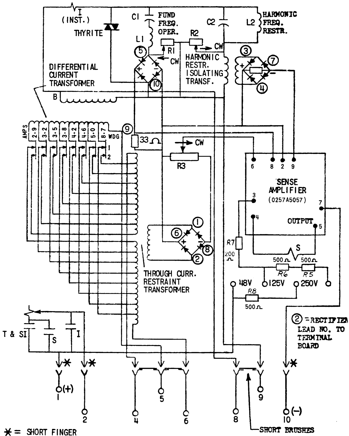
FIG. 10 (0257A502c- INTERNAL CONNECTIONS DIAGRAM FOR RELAY TYPE STD15C
