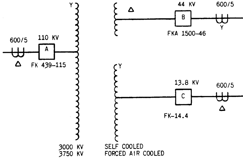
FIG. 17 (0165A7601-0) TRANSFORMER USED IN SAMPLE CALCULATIONS
