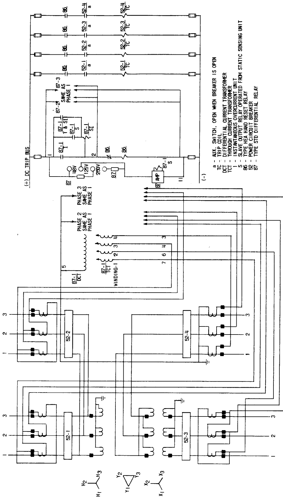
FIG. 2 (0165B2441-0) External Connections Diagram For The STD17C Relay
