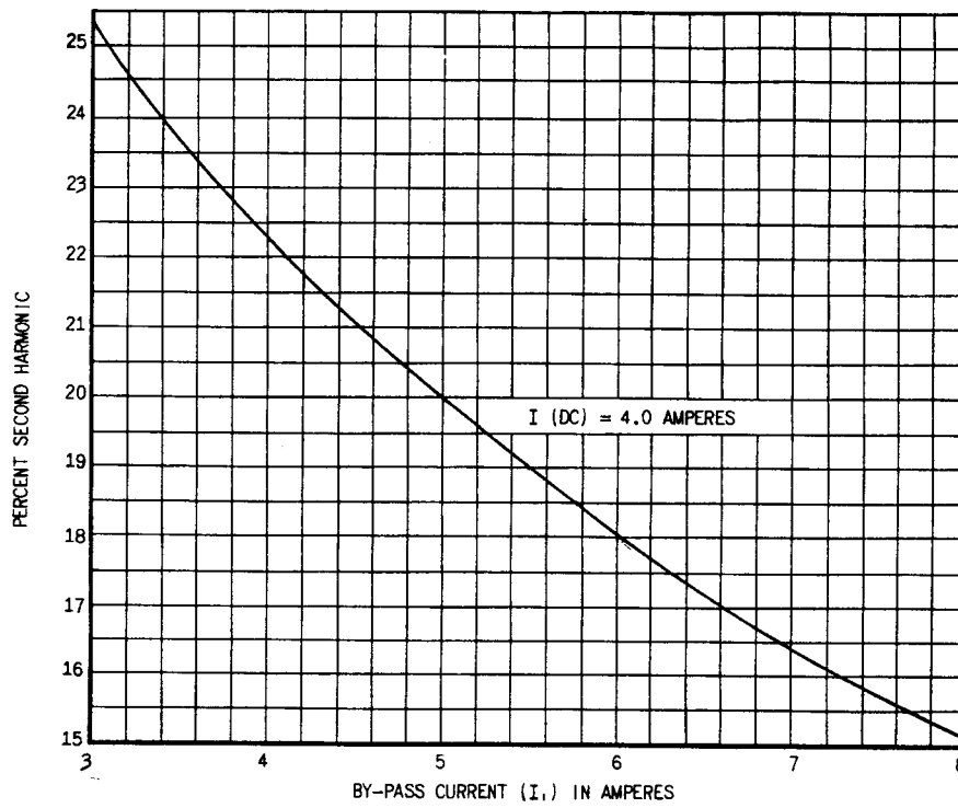
FIG. 15 (418A786-0) RELATIONSHIP BETWEEN PERCENT SECOND HARMONIC AND BY-PASS CURRENT WITH I(DC) SET AT 4.0 AMPERES
