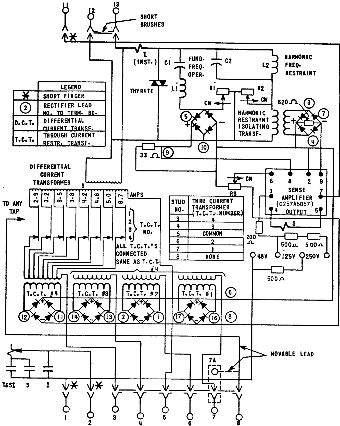
FIG. 1 (0257A5028-0) Internal Connections Diagram For The STD17C Relay (Front View)
