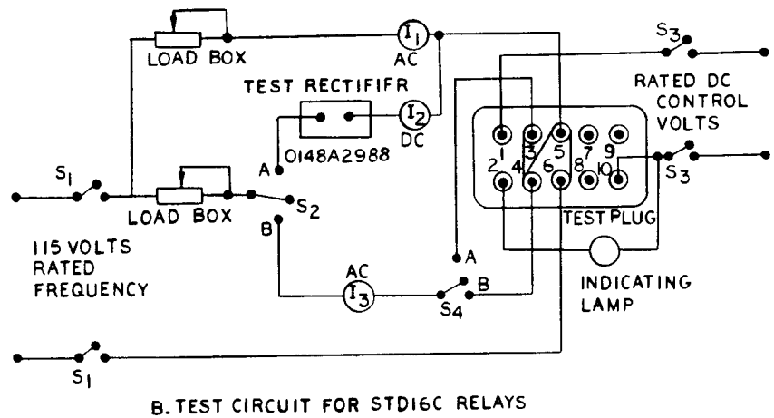
FIG. 14 (0257A5054-0 SH. 1) FIELD TEST CONNECTIONS, IN CASE, USING TYPE XLA TEST PLUG
