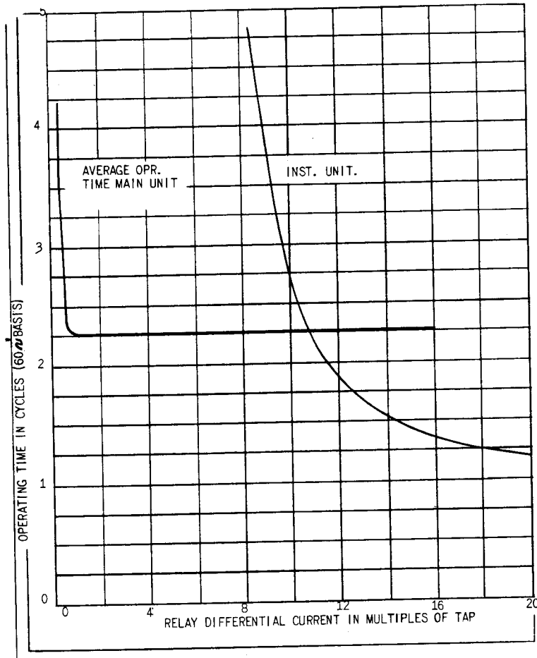
FIG. 2 (0227A2503-0) OPERATING SPEED CHARACTERISTICS OF THE STD RELAY
