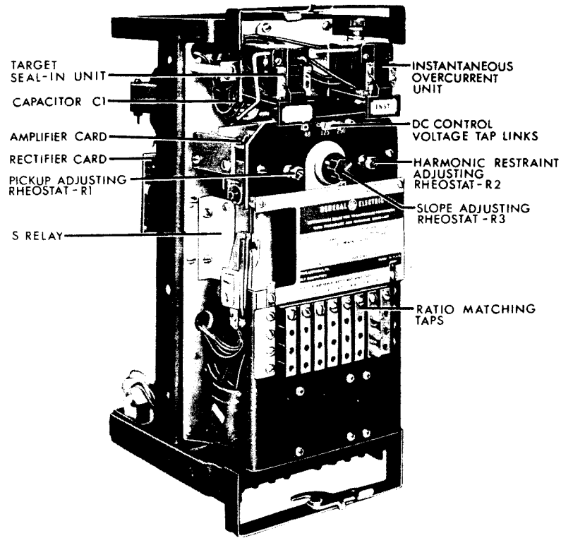
FIG. 4A (8042539) RELAY TYPE STD16C OUT OF CASE, APPROX 3/4 FRONT VIEW (LEFT SIDE)
