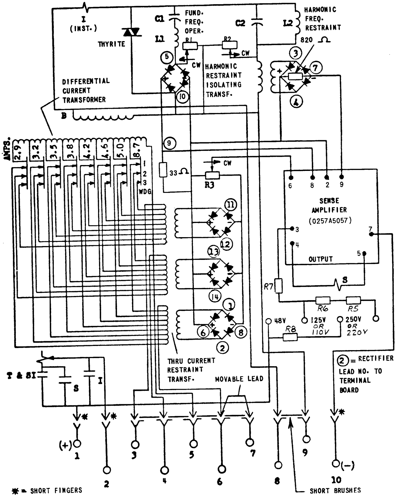
FIG. 11 (0257A5027-0) INTERNAL CONNECTIONS DIAGRAM FOR RELAY TYPE STD16C
