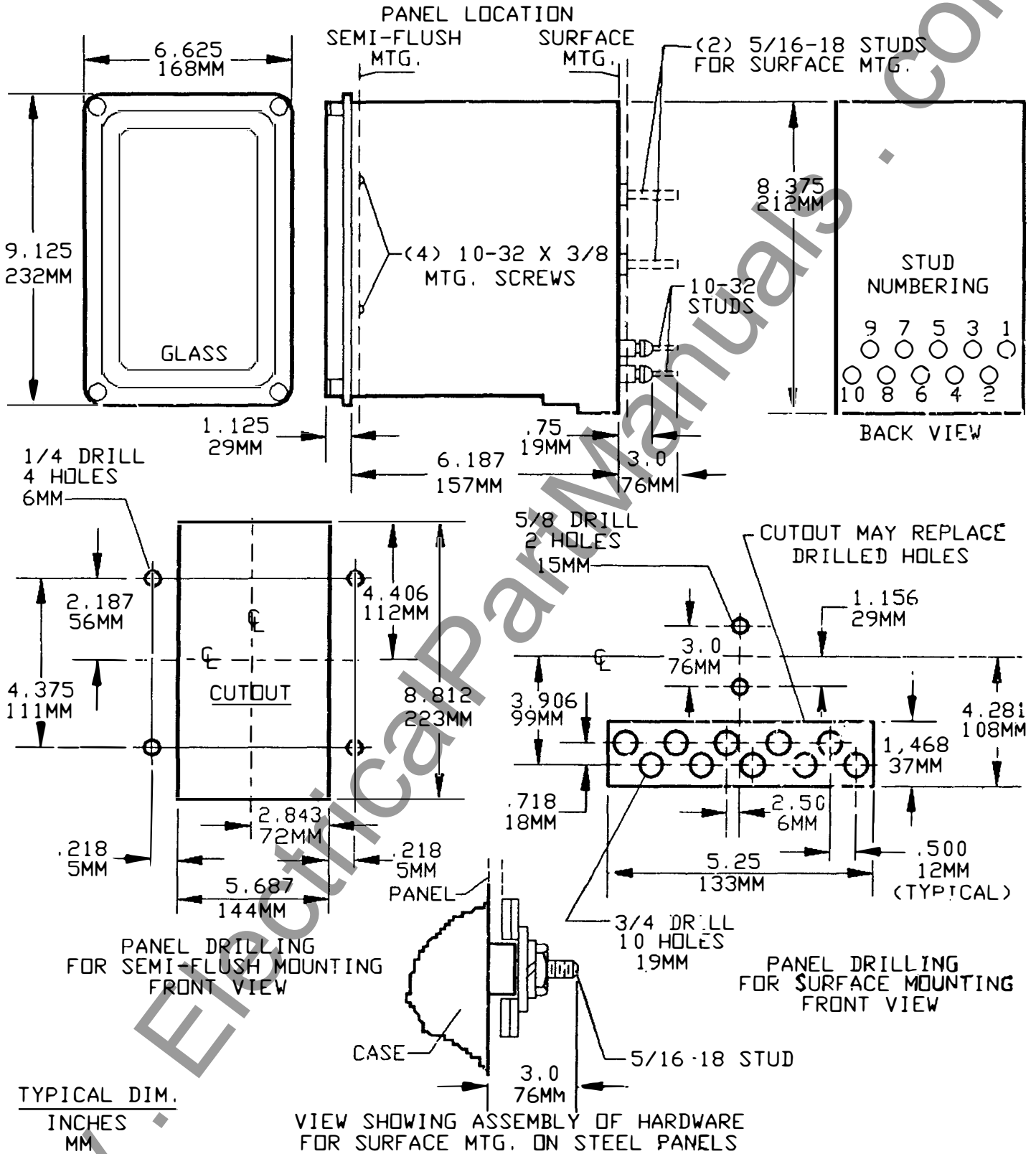
* FIG. 15 (K6209271-8) OUTLINE AND PANEL DRILLING FOR RELAY TYPES IAV51K AND IAV52K
