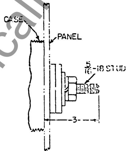
VIEW SHOWING ASSEMBLY OF HARDWARE FOR SURFACE MTG. ON STEEL PANELS
