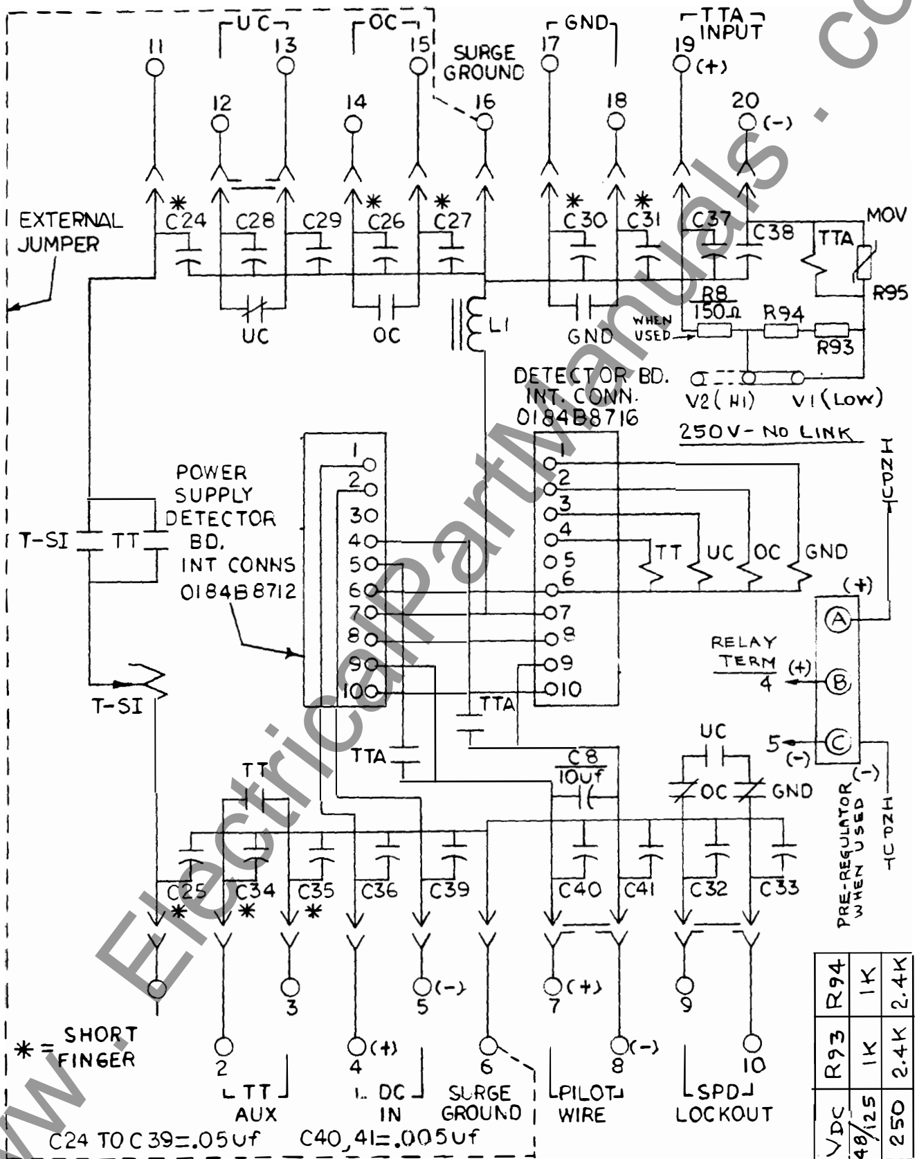
Figure 2 (0275A3241-3) Internal Connections Diagram for Type SPA11B Relay
