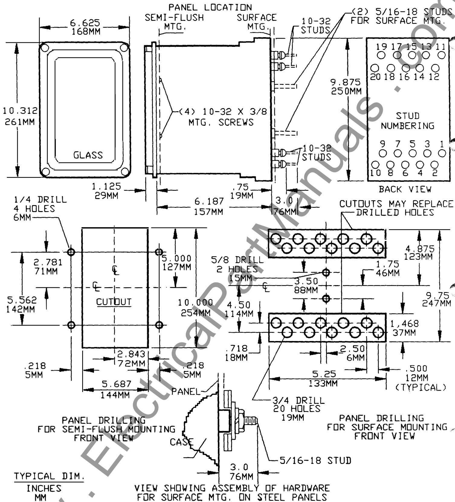
Figure 11 (006209272 [7]) Outline and Panel Drilling
