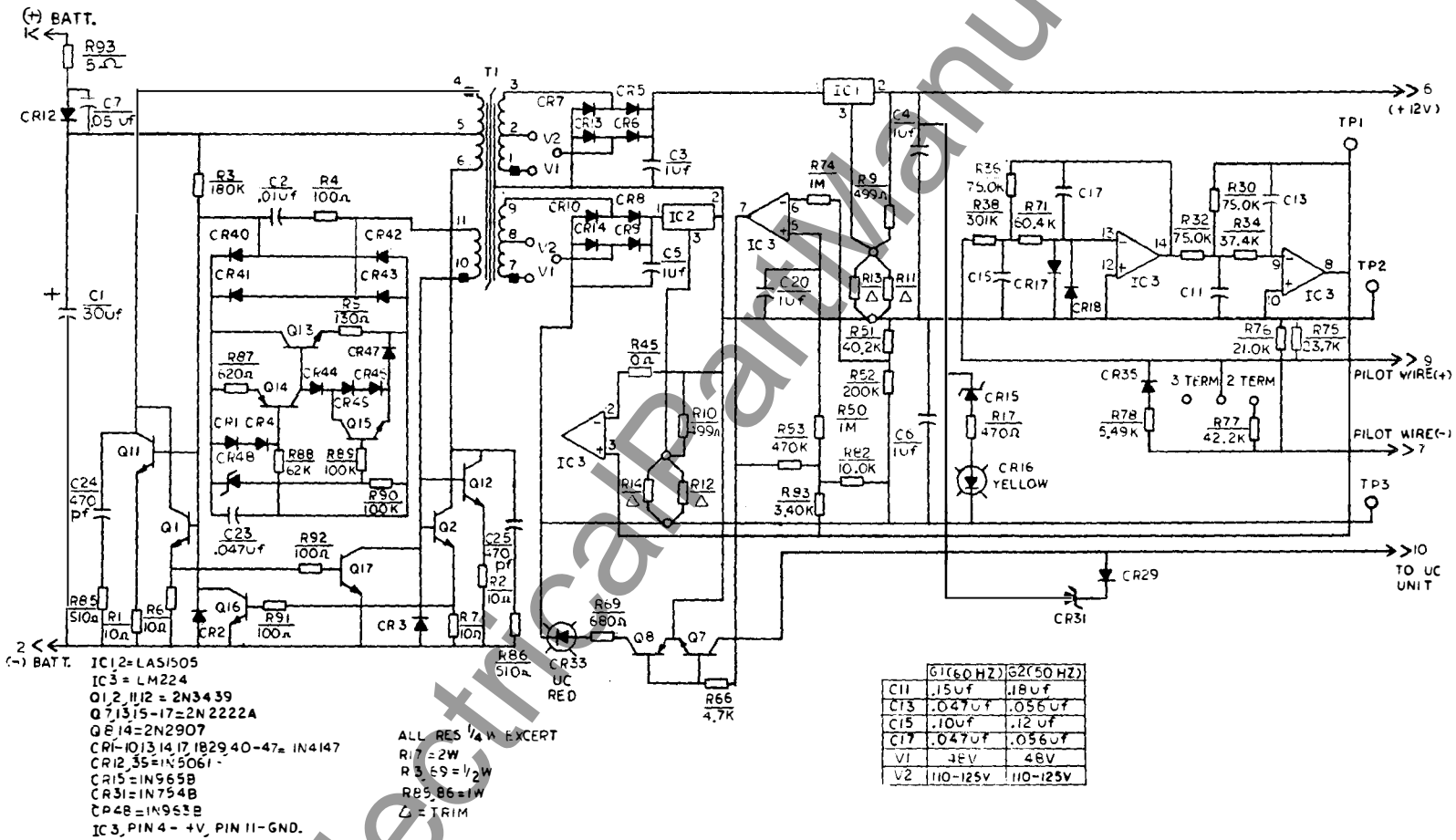
Figure 9a (0184B8715-4) Internal Connections for Printed Circuit Board in Position PCB-1 in SPA12A (No rev. letter) Board Identity: 0184B8615 G-
