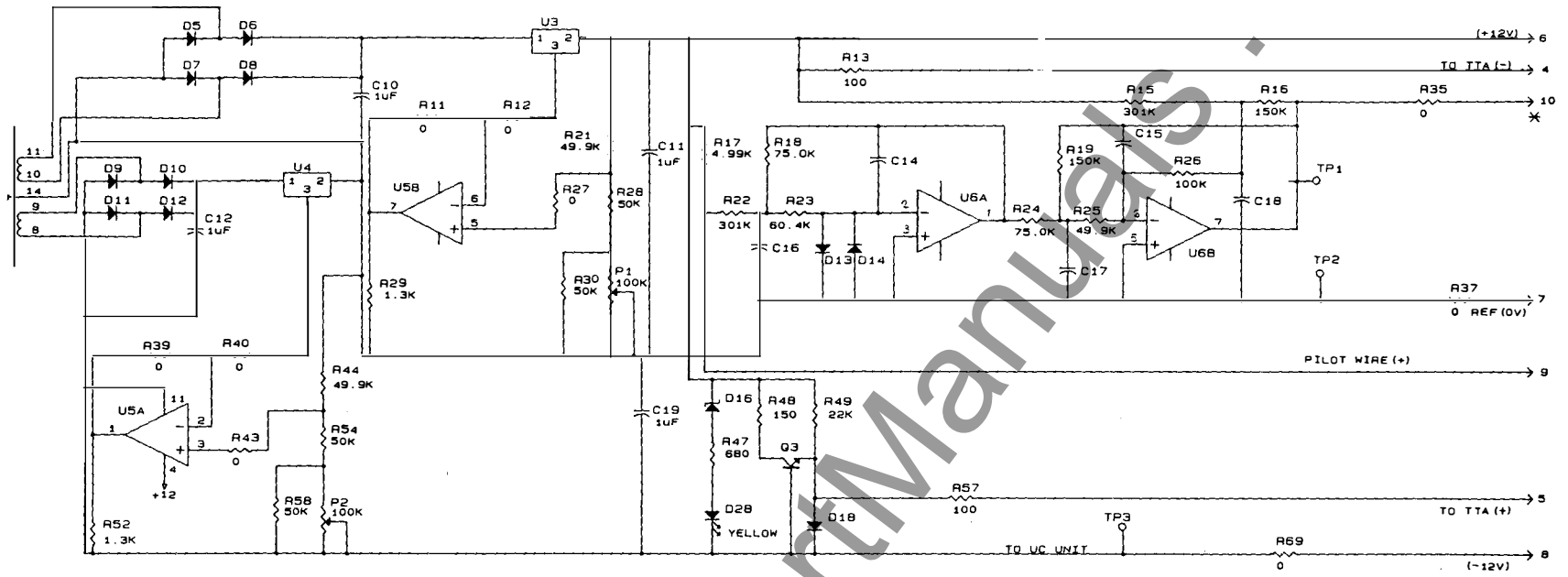
Figure 7b (0153D7689) Internal Connections for Printed Circuit Board in Position PCB-1 in SPA11B (Rev.A) Board Identity: 0184B8730 G-
