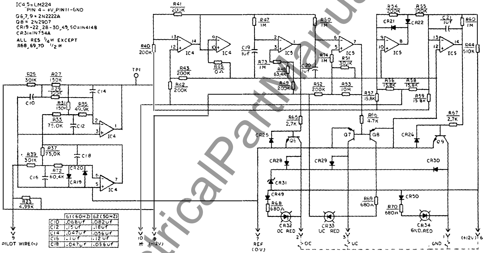
Figure 6 (0184B8717-1) Internal Connections for Printed Circuit Board in Position PCB-2 in SPA11A (both no Rev.letter and Rev.A) Board Identity: 0184B8617 G-
