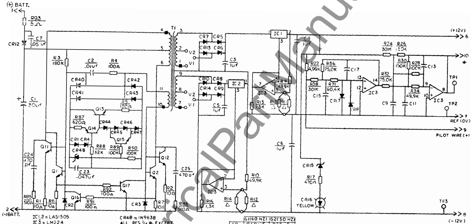
Figure 5a (0184B8714-4) Internal Connections for Printed Circuit Board in Position PCB-1 in SPA11A (No rev. letter) Board Identity: : 0184B8614-G-
