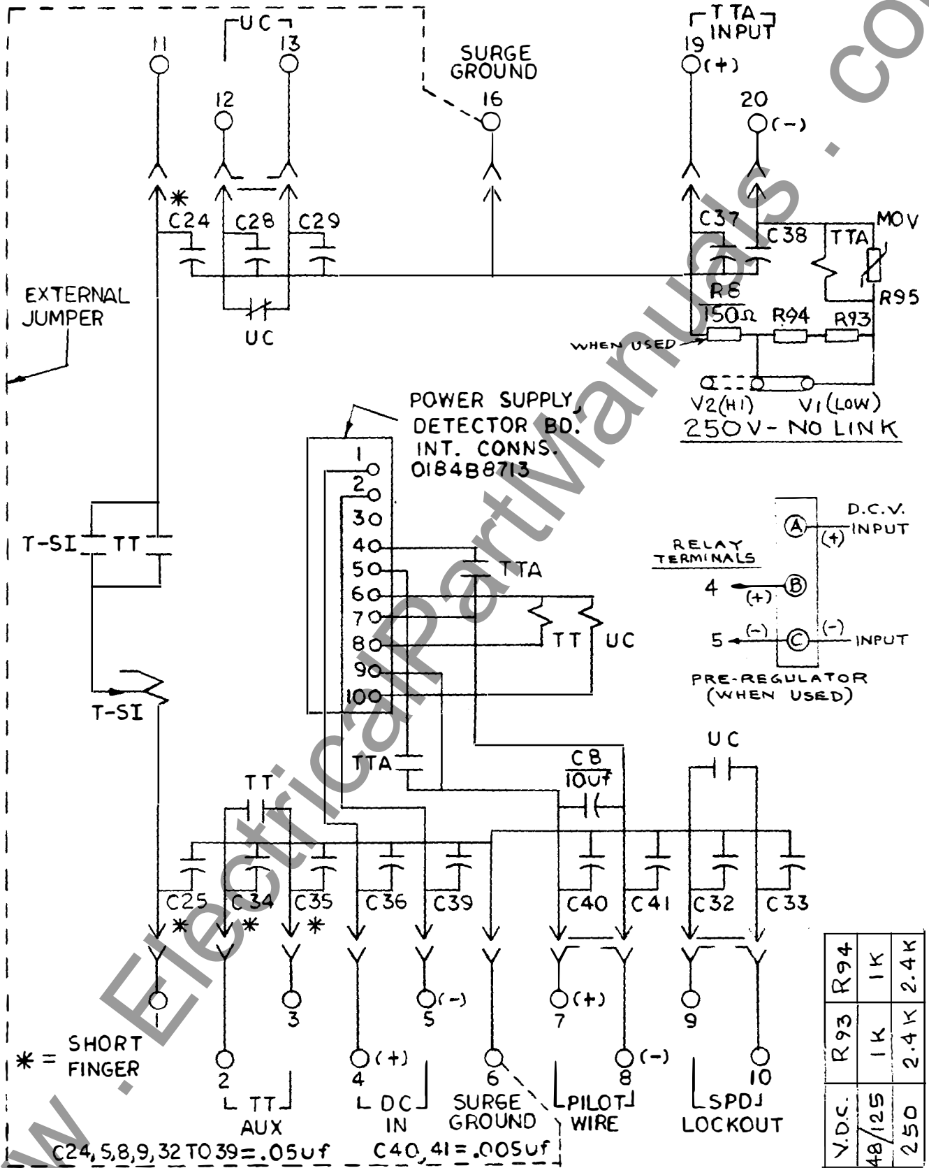
Figure 4 (0275A3243-3) Internal Connections Diagram for Type SPA12B Relay
