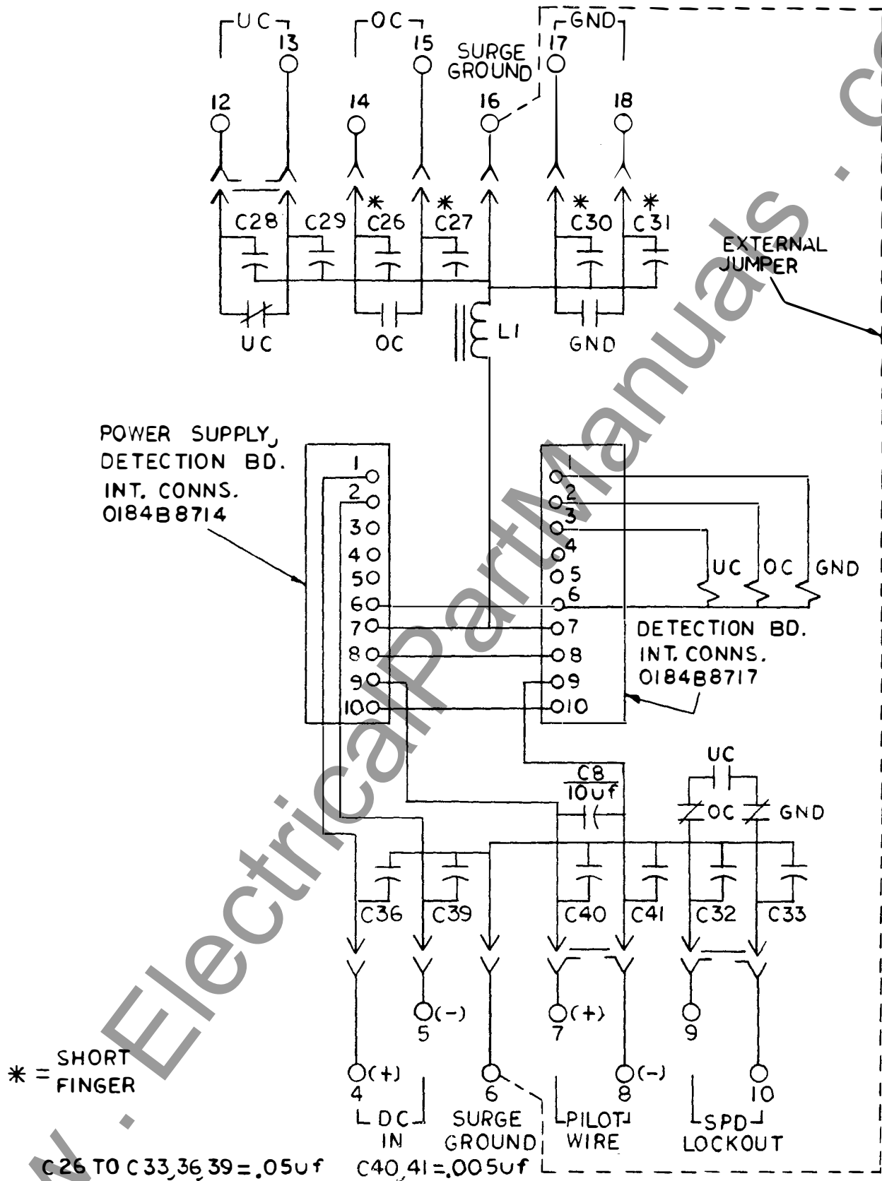
Figure 1 (0275A3240-0) Internal Connections Diagram for Type SPA11A Relay
