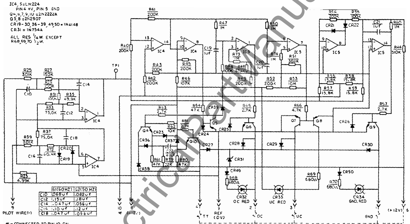
Figure 8 (0184B8716-1) Internal Connections for Printed Circuit Board in Position PCB-2 in SPA11B (both no rev. letter and Rev.A) Board Identity: 0184B8616 G-
