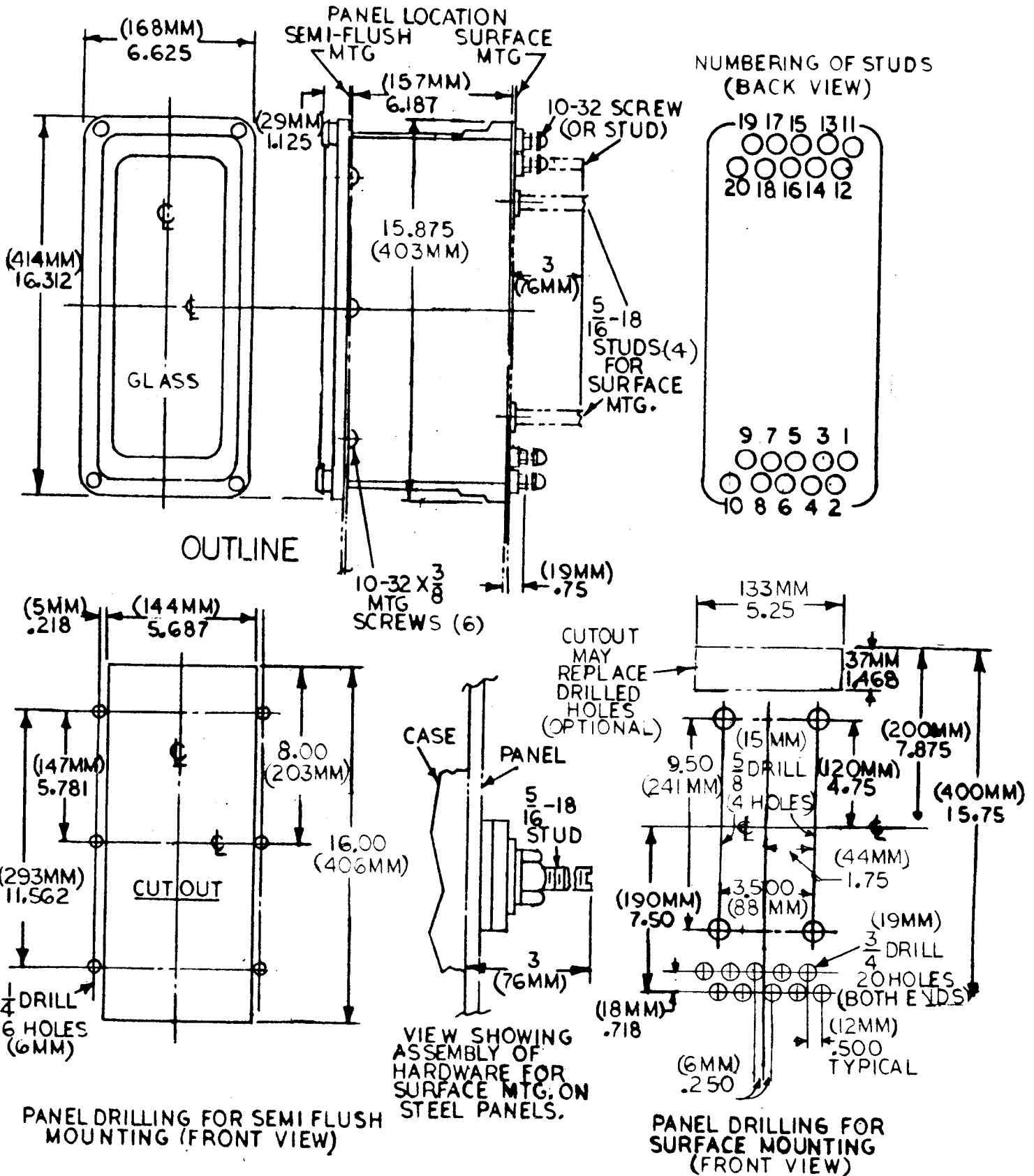
* Figure 11 (K620974-4) Outline and Panel-Drilling Dimensions for Drawout Relays, Size M2
