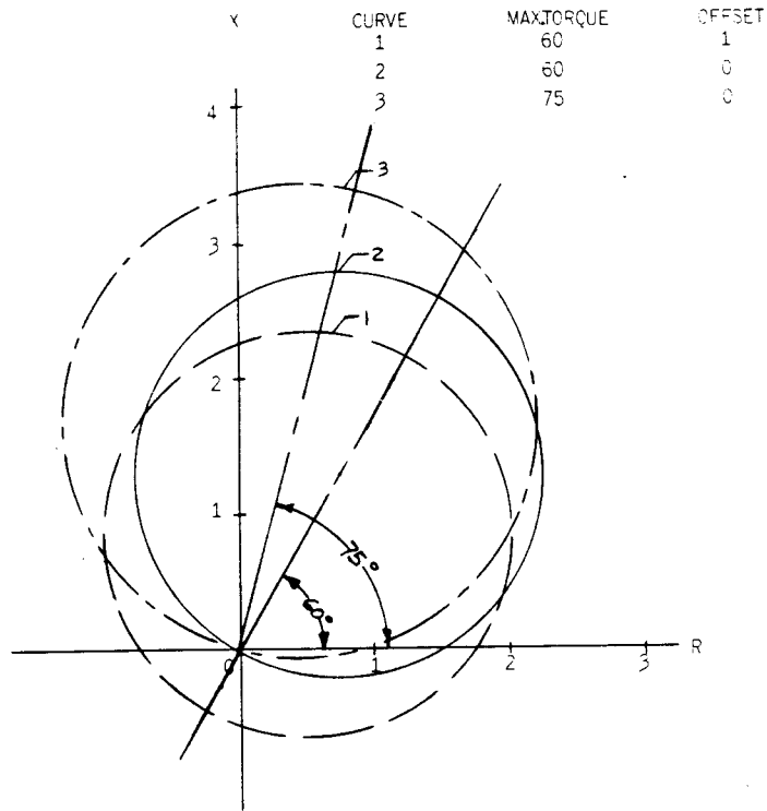
* Figure 2 (0208A3584-1) Typical Characteristics of the CEB51A Relay
