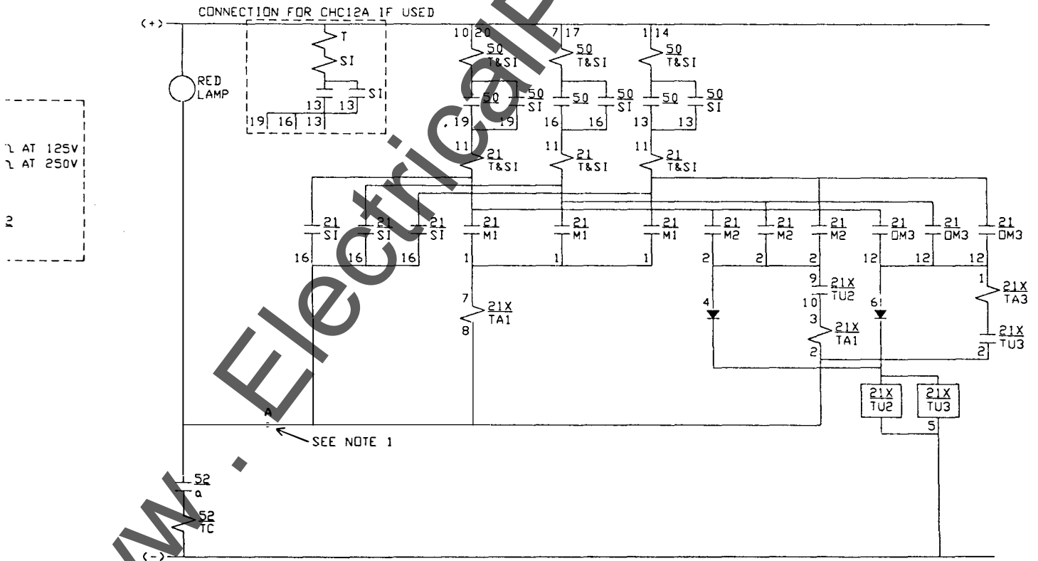
Figure 43 (0153D7812 [1]) SAM206 Used in Three-Zone Step Distance Scheme
