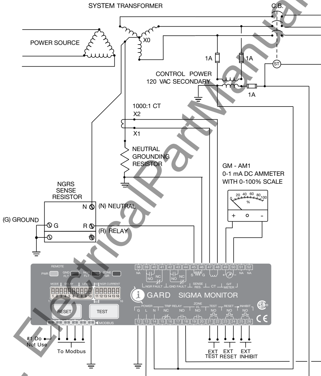
Figure 1 Sigma Monitor Relay Typical Installation Detail
