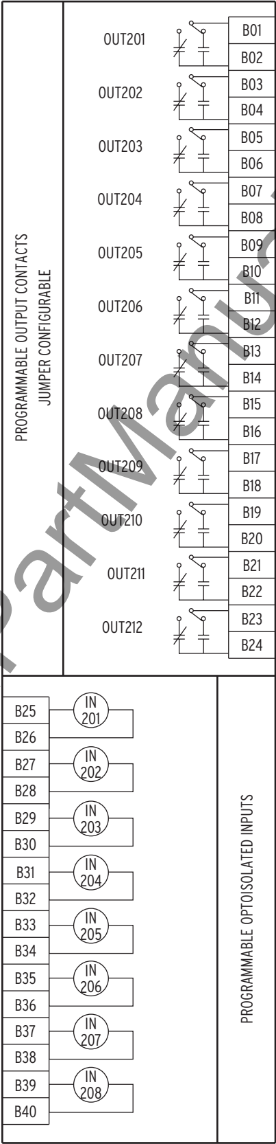
Figure 1.4 Extra I/O Board (Model 0351Sx1, Screw-Terminal Block Version; Main Board Shown in Figure 1.2 )
