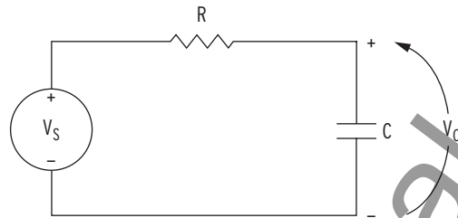
Figure 8.12 Voltage V_S Applied to Series RC Circuit
