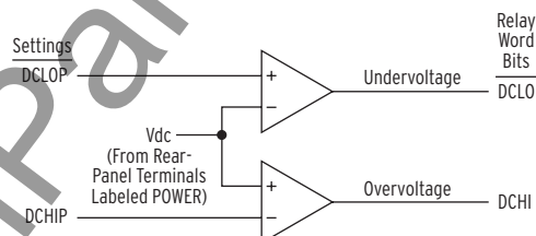
Figure 8.9 DC Under- and Overvoltage Elements
