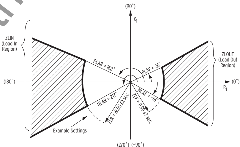
Figure 4.2 Load-Encroachment Logic
