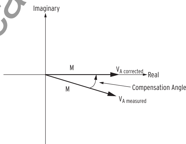
Figure L.3 Correction of Measured Phase Angle
