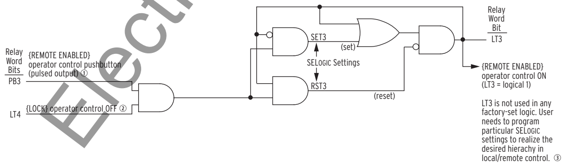
Figure 11.16 {REMOTE ENABLED} Operator Control Logic
