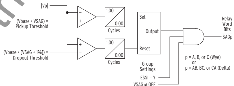
Figure 3.32 Voltage Sag Elements
