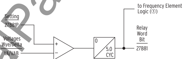
Figure 3.29 Undervoltage Block for Frequency Elements (Group Setting VNOM ≠ OFF)
