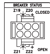
Connectorized Rear-Panel Breaker Status Labeling
