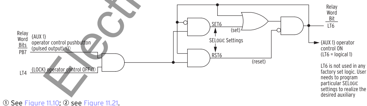
Figure 11.18 {AUX 1} Operator Control Logic
