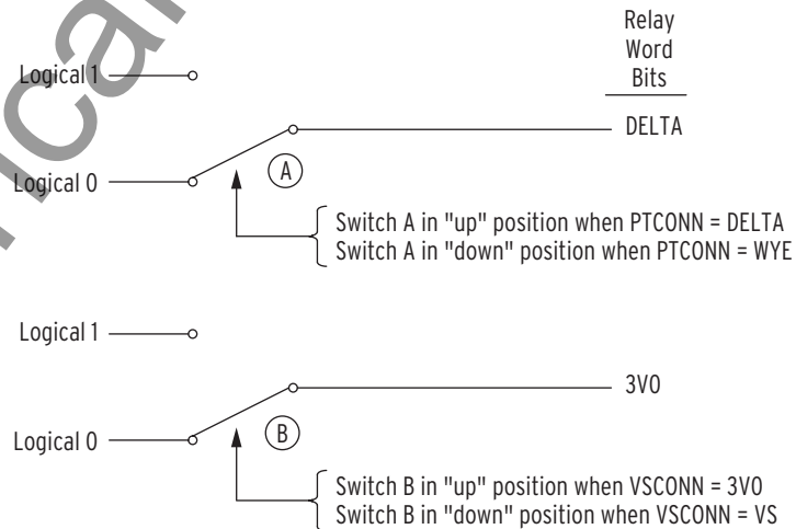
Figure 9.21 Operation of DELTA and 3V0 Relay Word Bits
