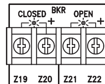
Rear-Panel Breaker Labeling With Conventional Terminal Blocks
