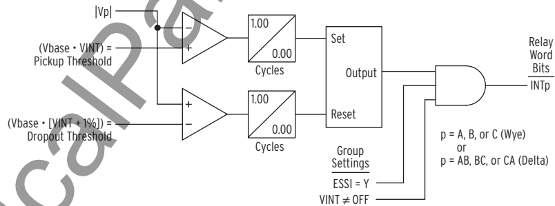
Figure 3.34 Voltage Interruption Elements
