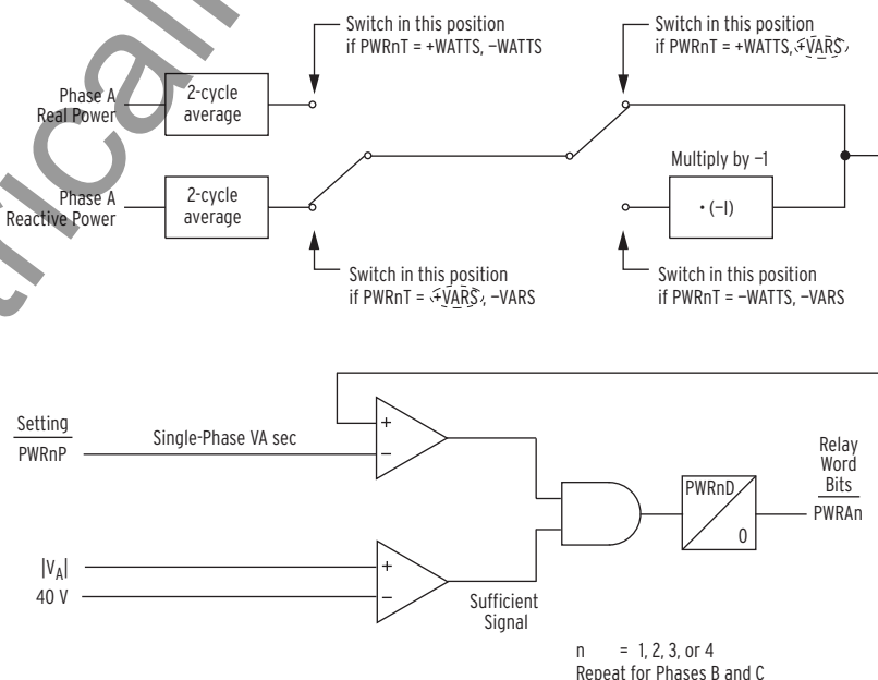
Figure 3.36 Single-Phase Power Elements Logic (+VARS Example Shown)
