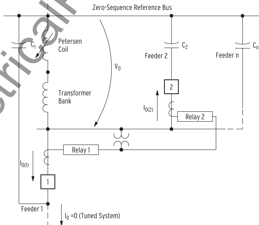
Figure 4.27 Zero-Sequence Impedance Network for Ground Fault on Feeder 1
