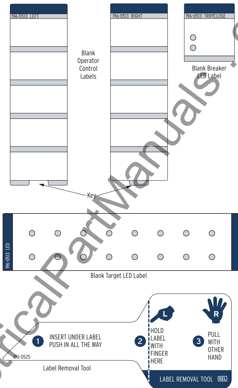
Figure 2.8 SEL-351S (Horizontal) Blank Slide-In Label Set and Label Removal Tool
