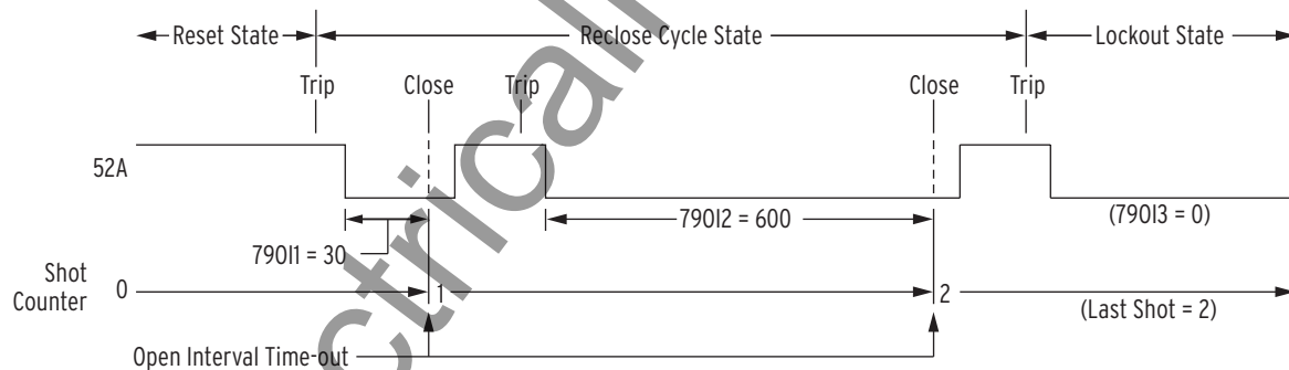
Figure 6.9 Example Reclosing Sequence From Reset to Lockout
