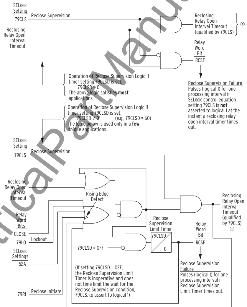
Figure 6.5 Reclose Supervision Logic (Following Open-interval Time-Out)
