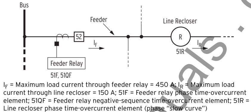
Figure F.2 Distribution Feeder Protective Devices
