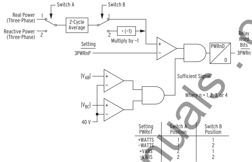
Figure 3.37 Three-Phase Power Elements Logic
