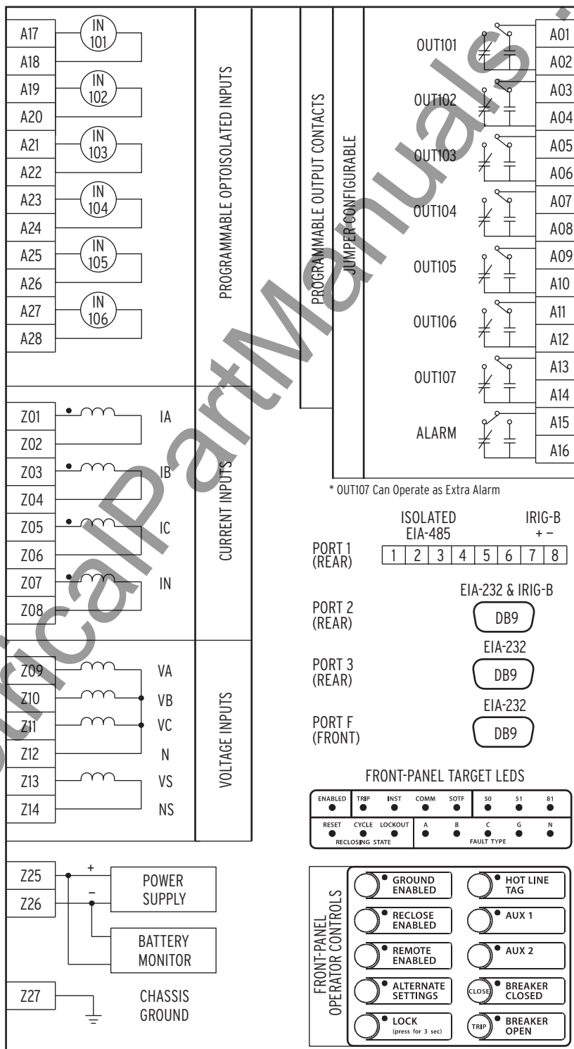
Figure 1.2 Inputs, Outputs, and Communications Ports (Extra I/O Boards in Figure 1.3 and Figure 1.4)
