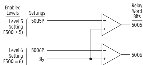
Figure 3.13 Levels 5-6 Negative-Sequence Instantaneous Overcurrent Elements
