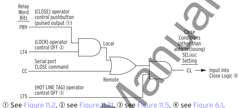
Figure 6.2 Close Conditions—Other Than Auto-Reclosing
