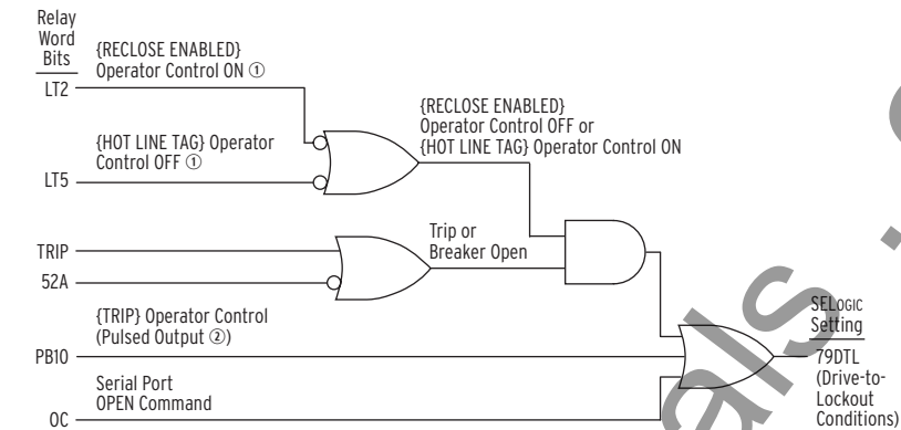
Figure 6.10 Factory-Default Drive-to-Lockout Logic
