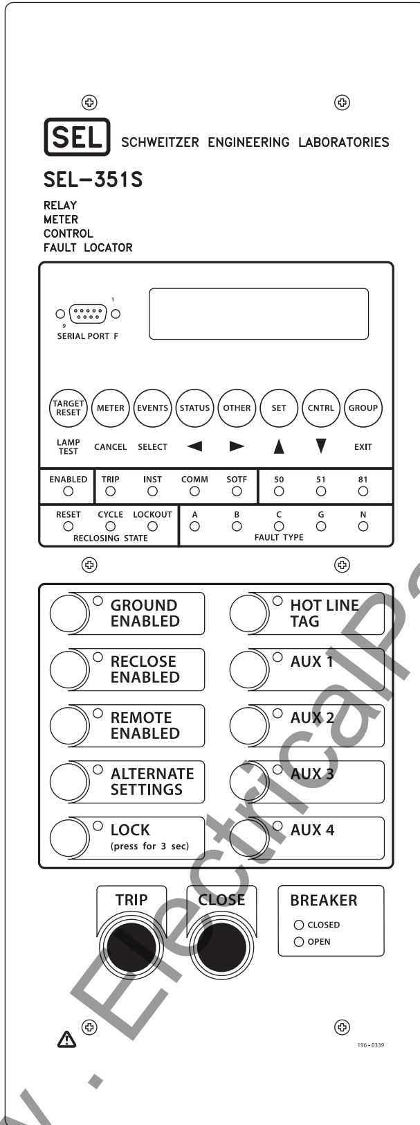
Figure 2.5 SEL-351S with Auxiliary {TRIP}/{CLOSE} Pushbuttons (Model 0351Sx145xxx6x); Vertical Panel-Mount Example, (Conventional Terminal Blocks, With Additional I/O Board)
