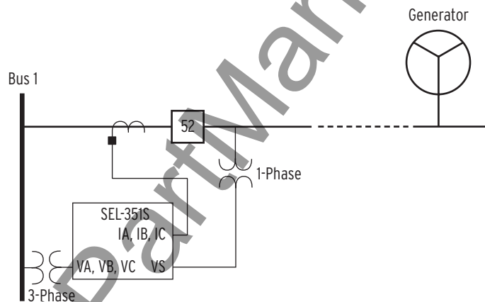
Figure 6.11 Reclose Blocking for Islanded Generator
