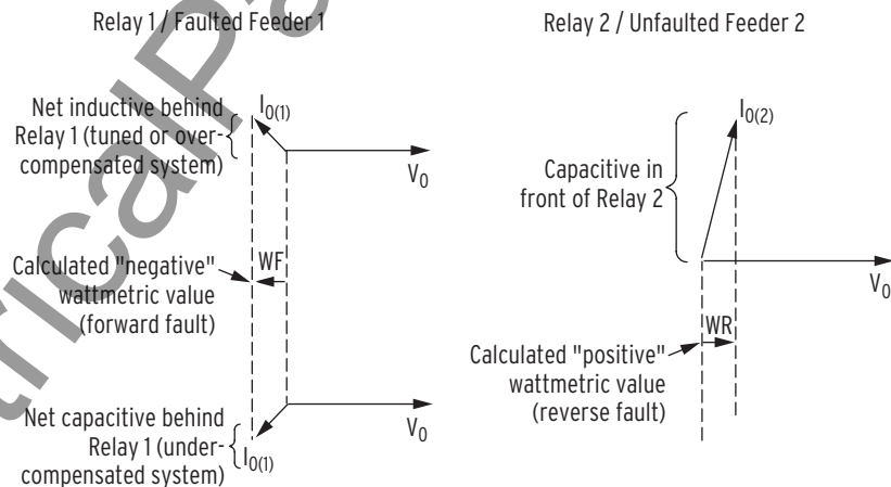
Figure 4.28 Wattmetric Element Operation for Ground Fault on Feeder 1
