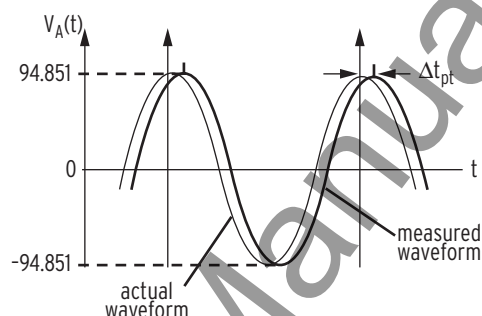
Figure L.2 Waveform at Relay Terminals May Have Phase Shift
