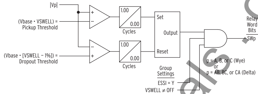
Figure 3.33 Voltage Swell Elements
