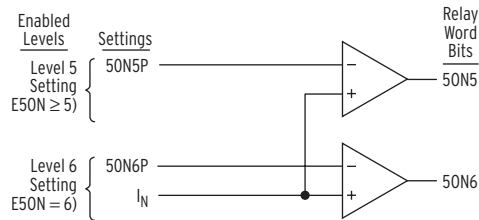
Figure 3.9 Levels 5-6 Neutral Ground Instantaneous Overcurrent Elements
