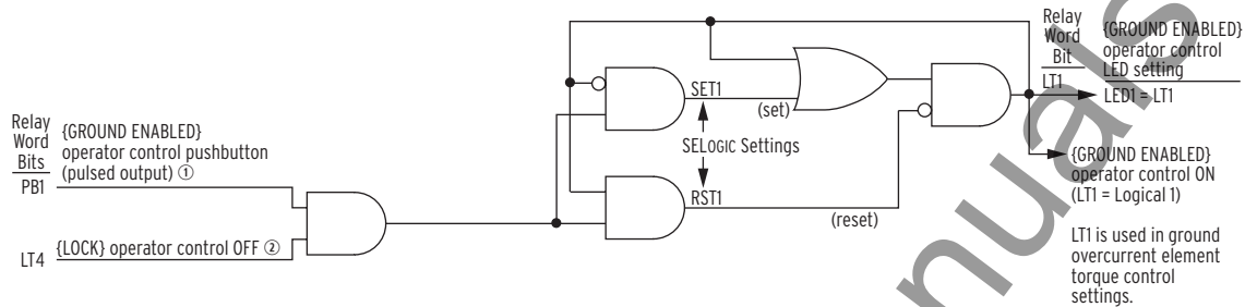
Figure 11.14 {GROUND ENABLED} Operator Control LED and Logic
