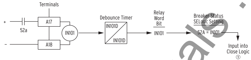
Figure 6.4 Breaker Status Determination
