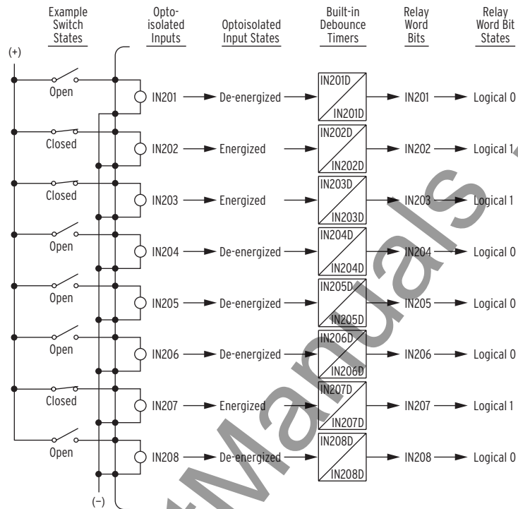
Figure 7.2 Example Operation of Optoisolated Inputs IN201-IN208-Extra I/O Board
