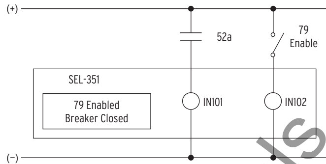
Figure 7.30 Rotating Default Display Replaces Traditional Panel Light Installations
