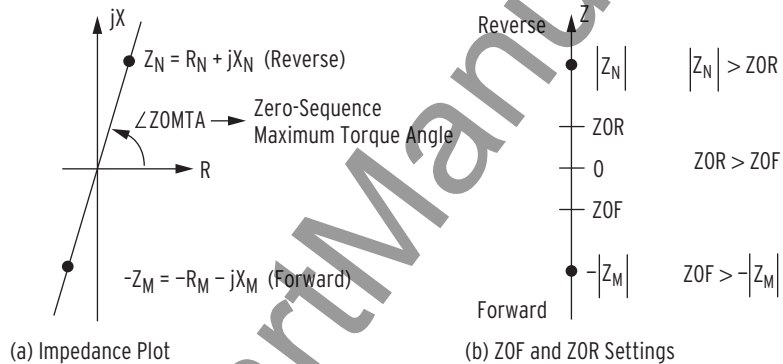
Figure 4.26 Zero-Sequence Impedance Plot for Solidly-Grounded, Mostly Inductive System
