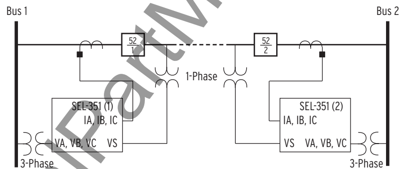
Figure 6.7 SEL-351S Relays Installed at Both Ends of a Transmission Line in a High-Speed Reclose Scheme
