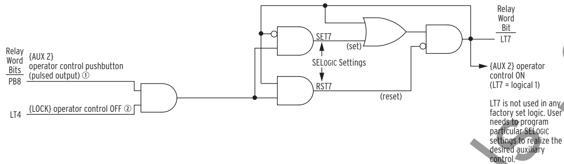
Figure 11.19 {AUX 2} Operator Control Logic
