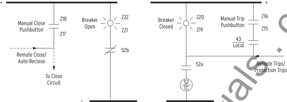
Figure 2.31 SEL-351S Example Wiring Diagram Using the Auxiliary {TRIP}/{CLOSE} Pushbuttons for 0351Sxxx5/6/A/B Models
