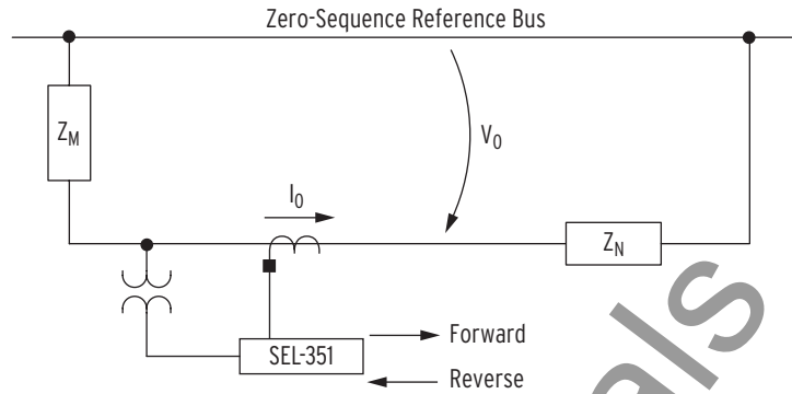
Figure 4.25 Zero-Sequence Impedance Network and Relay Polarity
