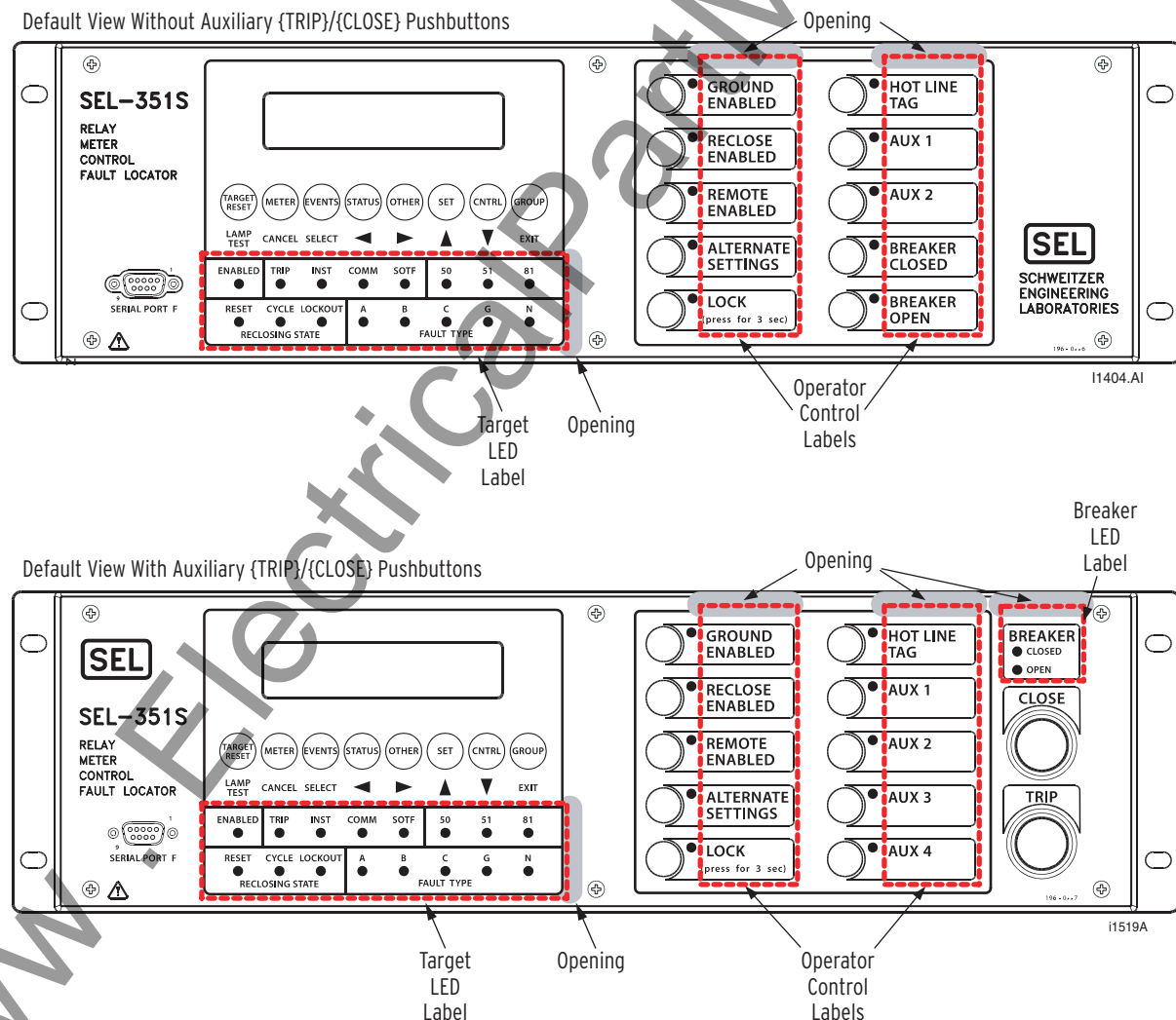
Figure 2.7 SEL-351S (Horizontal) With User-Configurable Default Labels
