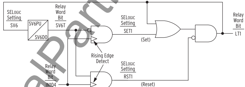
Figure 7.17 Latch Control Switch (With Time Delay Feedback) Controlled by a Single Input to Enable/Disable Reclosing
