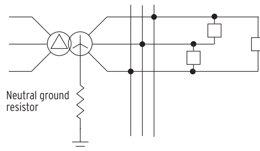
Figure 9.22 Hybrid Power System With Neutral Ground Resistor
