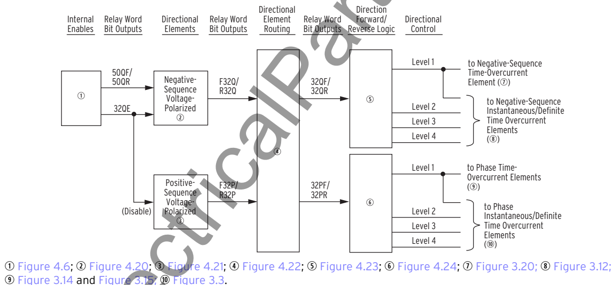
Figure 4.19 General Logic Flow of Directional Control for Negative-Sequence and Phase Overcurrent Elements
