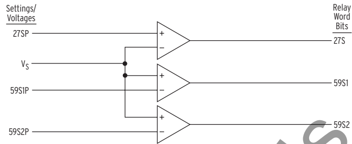
Figure 3.25 Channel VS Voltage Elements (Wye- or Delta-Connected PTs)
