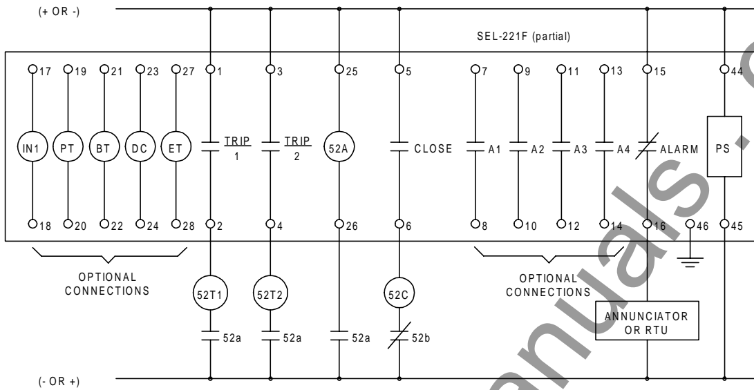
Figure 8: SEL-221F Relay Typical DC Connections
