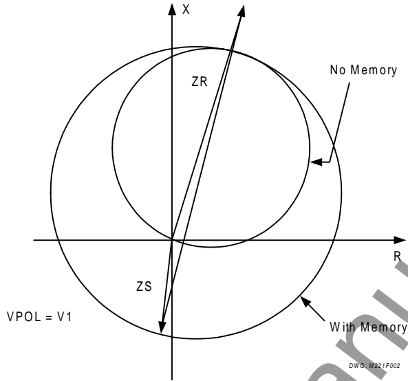
Figure 2: Phase-to-Phase Element Response for a Three-Phase Forward Fault
