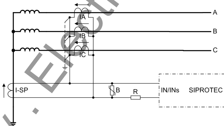
Figure 2-23 Connection diagram of the ground fault differential protection according to the high-impedance principle
