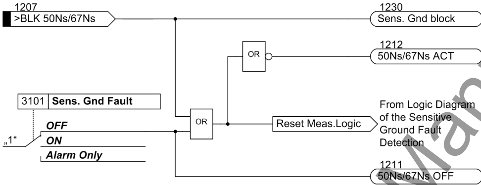
Figure 2-49 Activation of the sensitive ground current protection
