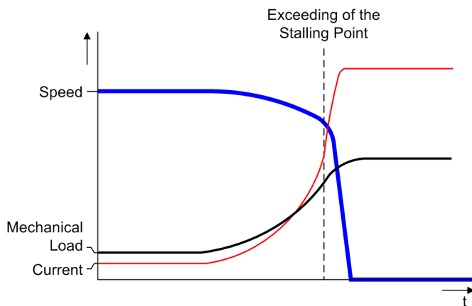
Figure 2-37 Example of the time characteristic for mechanical rotor blocking
