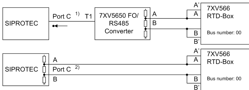
Figure A-16 Simplex operation with one RTD-Box, above: optical design (1 FO); below: design with RS 485
