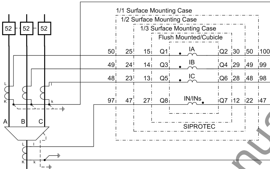
Figure A-11 Current connections to three current transformers, ground current from additional summation CT, normal circuit layout
