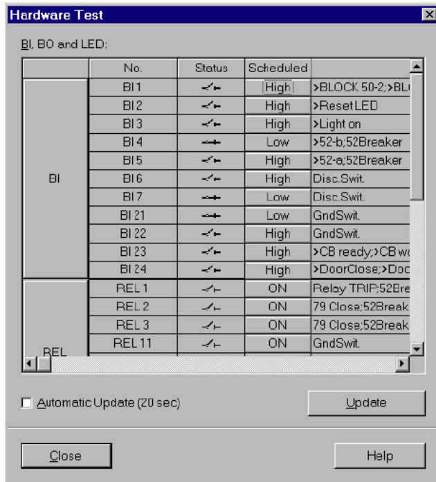
Figure 3-20 Test of the binary inputs/outputs — example
