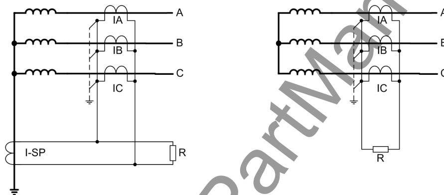
Figure 2-21 Ground fault protection according to the high-impedance principle
