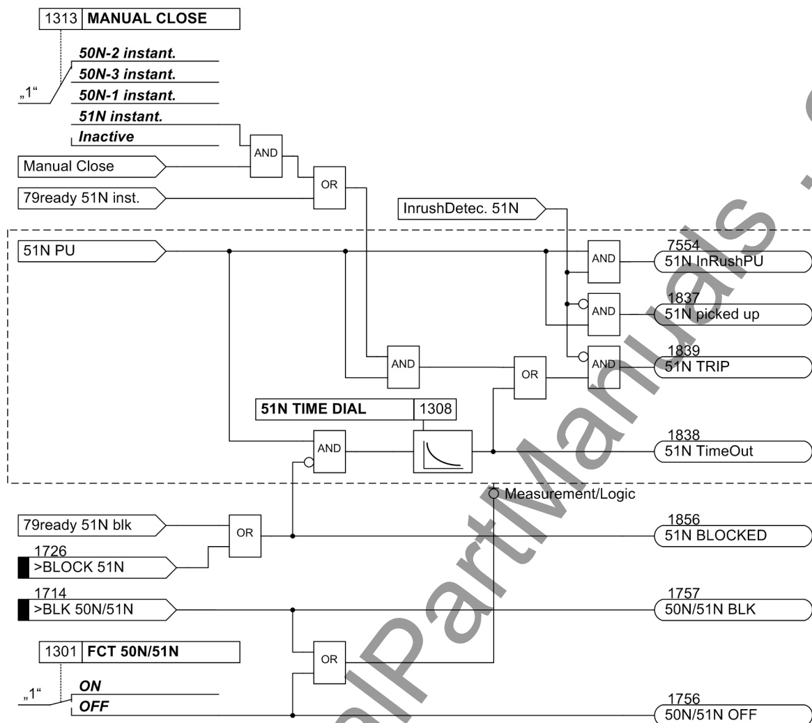
Figure 2-11 Logic diagram of the inverse-time overcurrent protection element for ground
