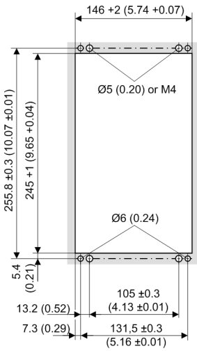
Panel Cut-Out
