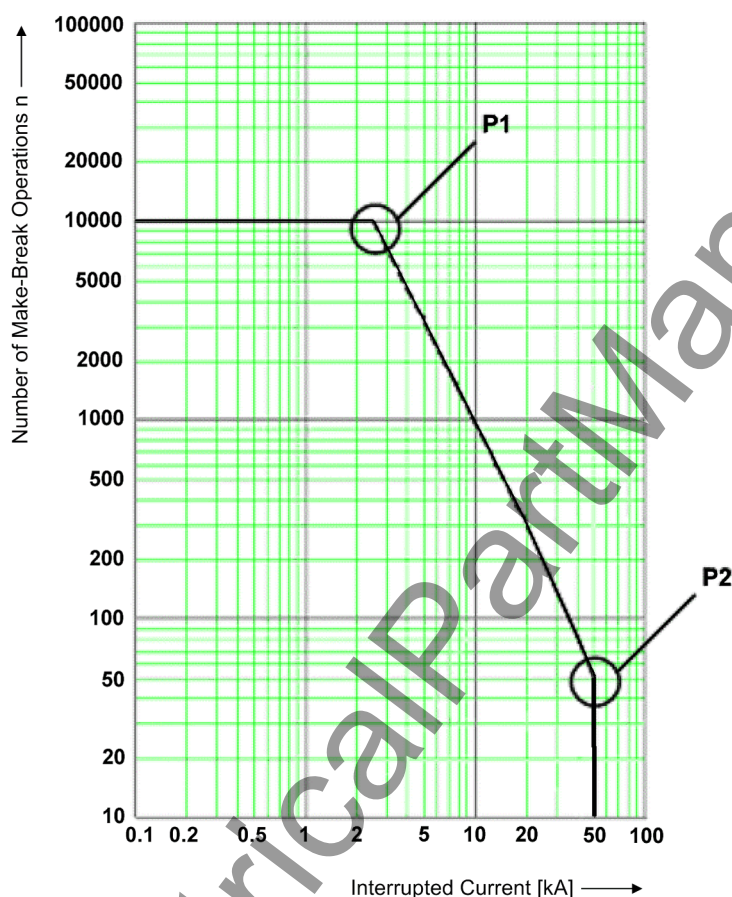
Figure 2-74 Diagram of operating cycles for the 2P procedure
