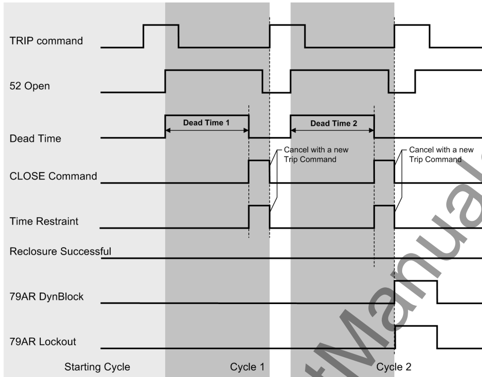
Figure 2-57 Timing diagram showing two unsuccessful reclosing shots
