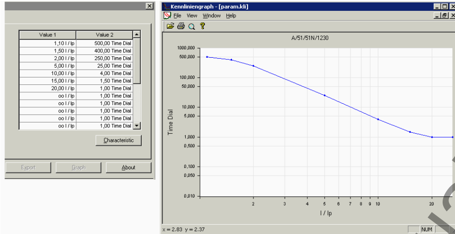
Figure 2-15 Entry and visualization of a user-defined tripping characteristic in DigiS — example
