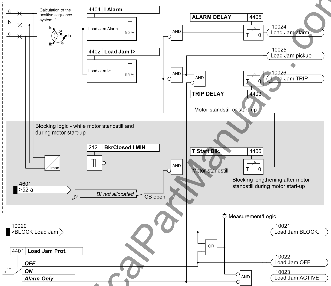
Figure 2-38 Logic diagram of the load jam protection
