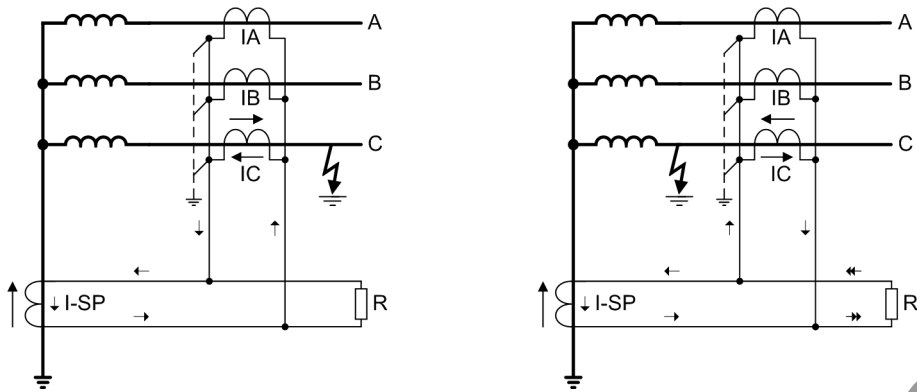
Figure 2-22 Principle of ground fault protection according to the high-impedance principle
