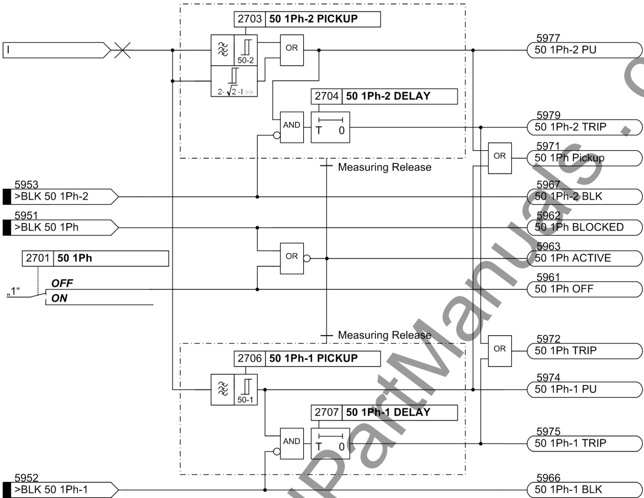
Figure 2-20 Logic diagram of the single-phase time overcurrent protection
