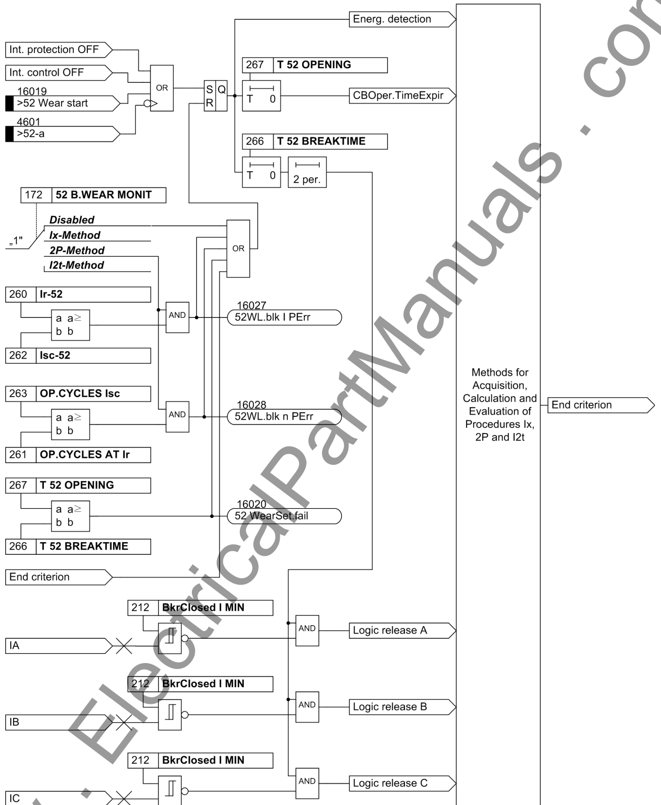
Figure 2-73 Logic of the start and end criterion
