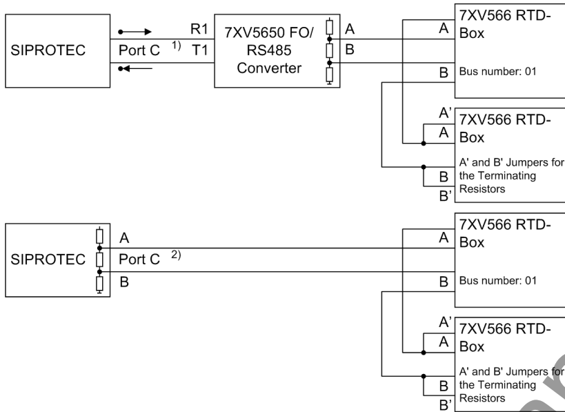
Figure A-18 Half-duplex operation with two RTD-Boxes, above: optical design (2 FOs); below: design with RS 485 1) for 7SJ64 port D 2) for 7SJ64 optionally port C or port D
