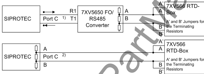
Figure A-17 Half-duplex operation with one RTD-Box, above: optical design (2 FOs); below: design with RS 485
