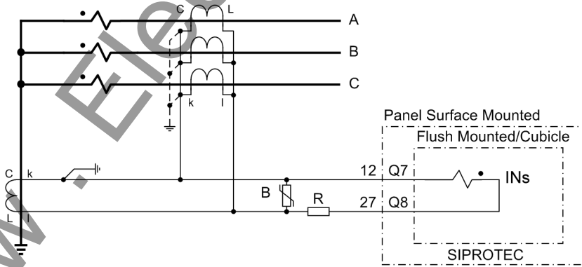
Figure A-15 High-impedance differential protection for a grounded transformer winding ( showing the partial connection for the high-impedance differential protection)
