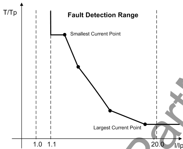
Figure 2-53 Use of a user-defined characteristic
