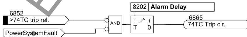
Figure 2-47 Logic diagram of trip circuit supervision with one binary input
