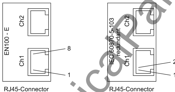
Figure 3-18 RJ45 sockets
