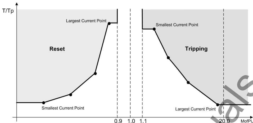
Figure 2-14 Using a user-defined curve
