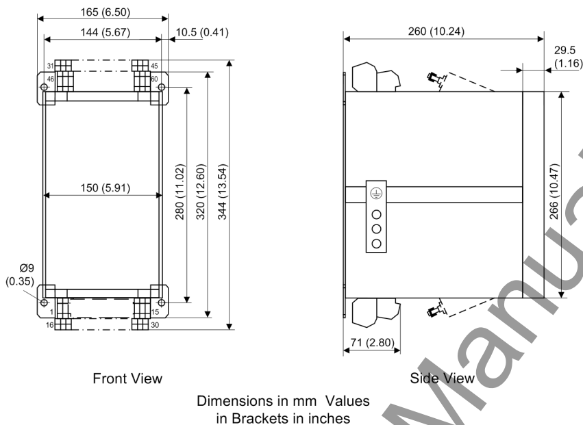
Figure 4-14 Dimensional drawing of a 7SJ61 for panel flush mounting (housing size 1/3)
