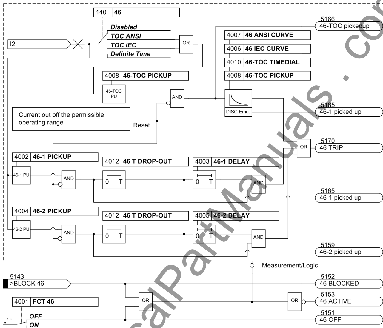
Figure 2-29 Logic diagram of the unbalanced load protection
