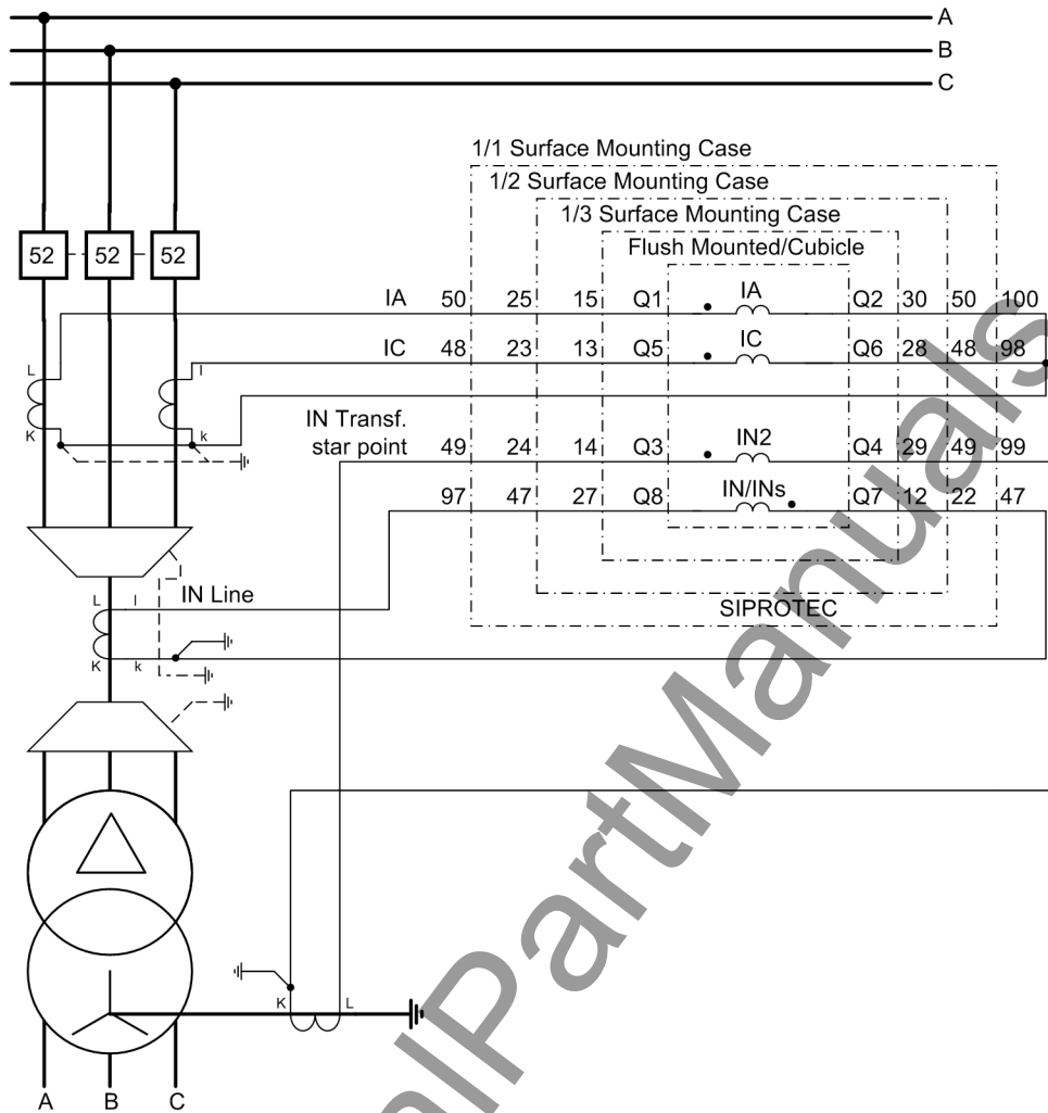
Figure 2-3 Measurement of two ground currents, example
