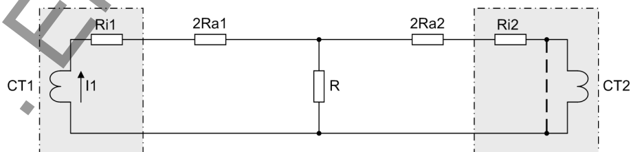
Figure 2-25 Simplified equivalent circuit of a circulating current system for high-impedance protection
