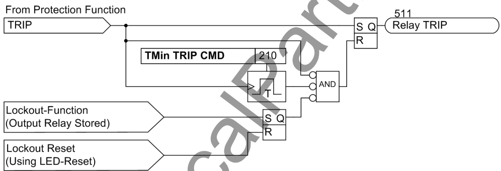
Figure 2-70 Terminating the Trip Signal
