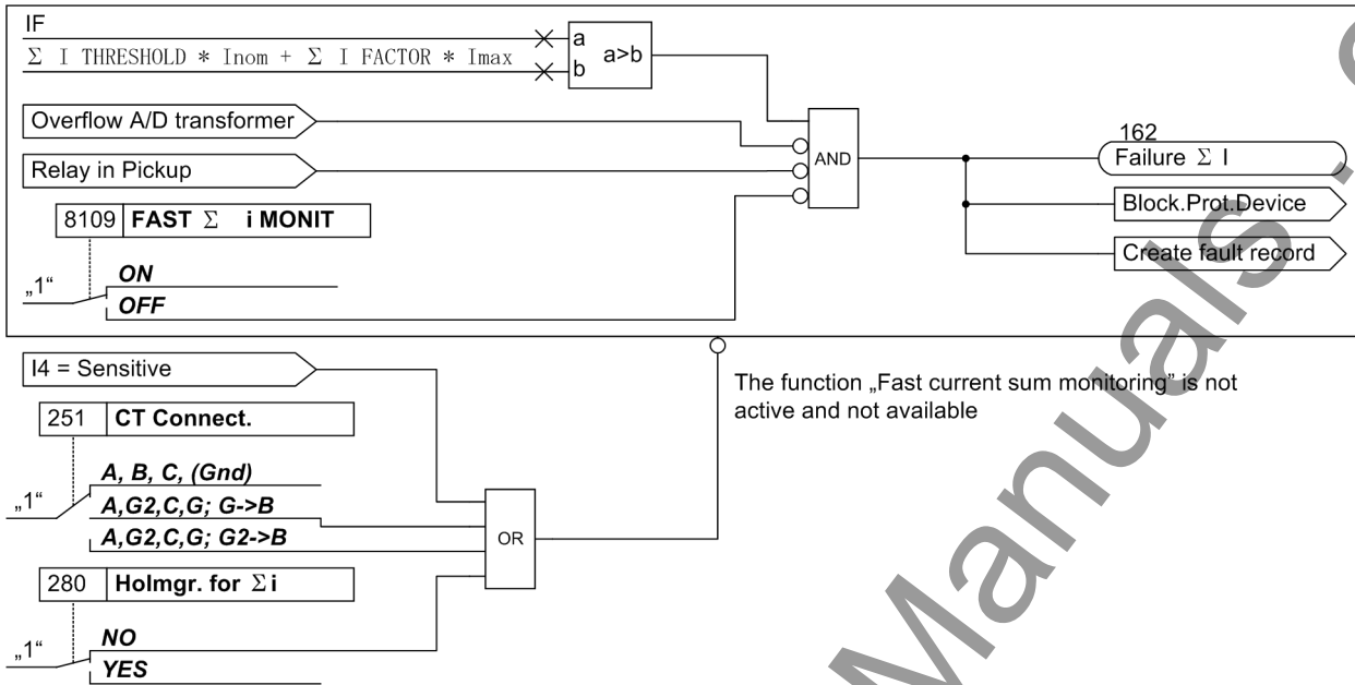
Figure 2-42 Logic Diagram of the fast current sum monitoring
