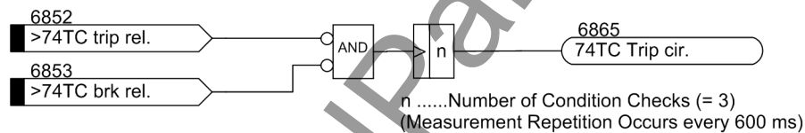
Figure 2-45 Logic diagram of the trip circuit supervision with two binary inputs
