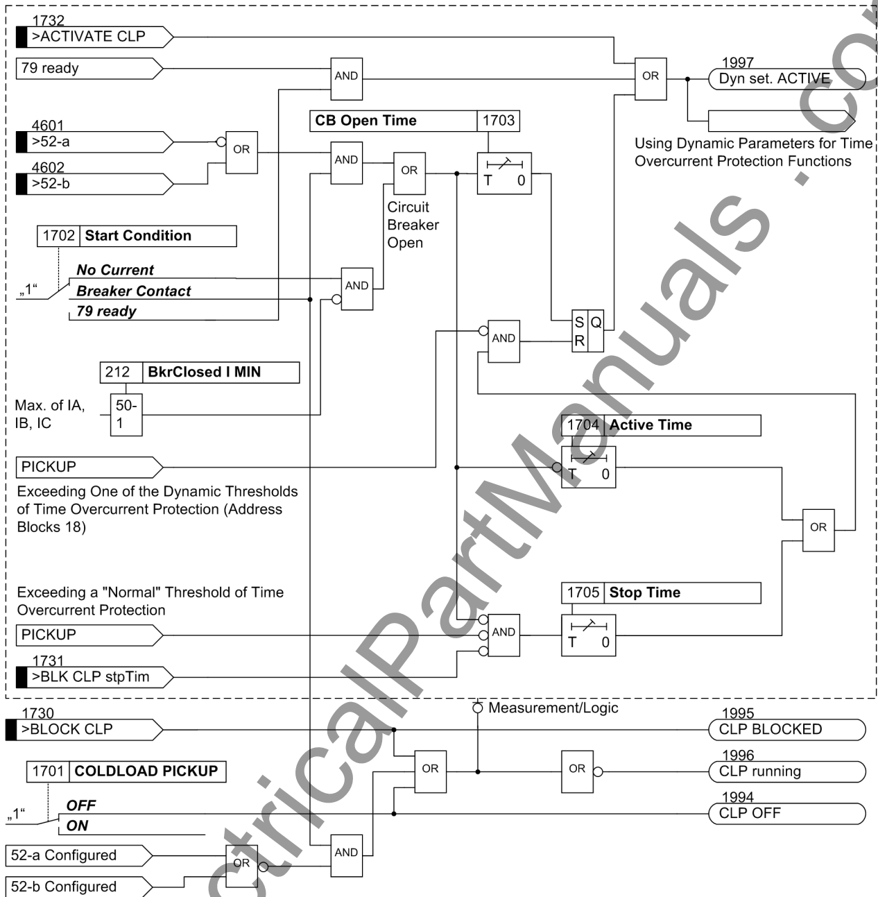
Figure 2-18 Logic diagram of the dynamic cold load pickup function (50c, 50Nc, 51c, 51Nc, 67c, 67Nc)
