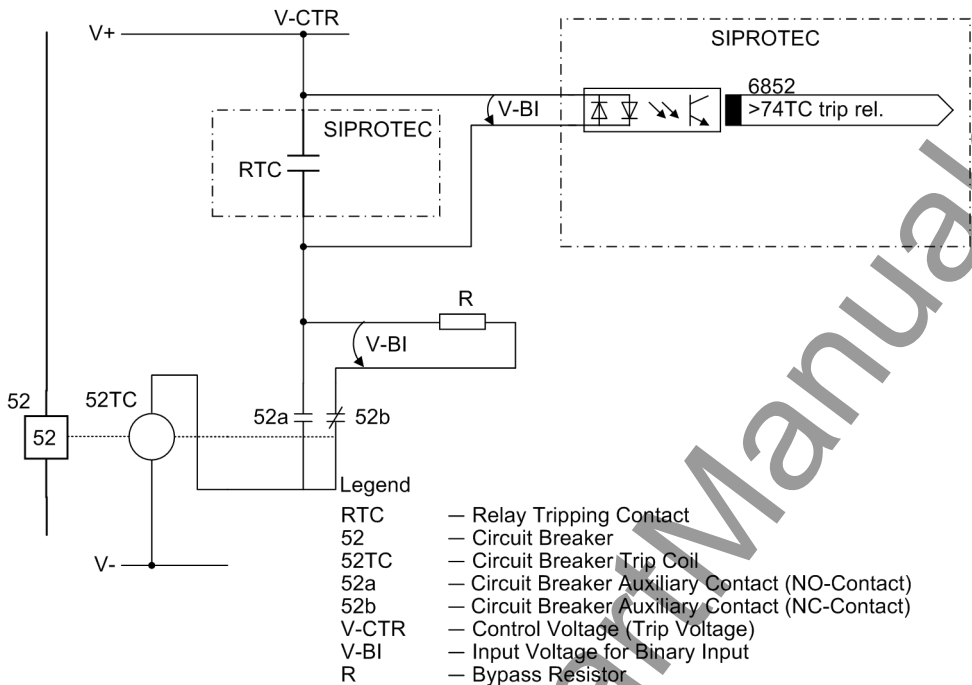
Figure 2-46 Trip circuit supervision with one binary input
