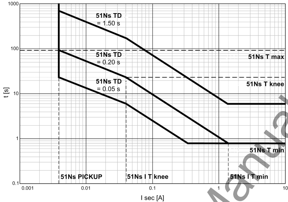
Figure 2-52 Trip-time characteristics of the inverse-time ground fault protection 51Ns with logarithmic inverse characteristic with knee point (example for 51Ns = 0.004 A)
