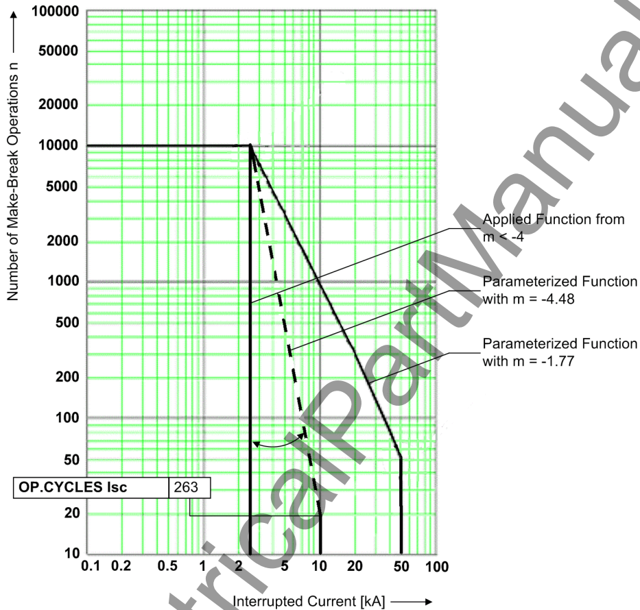
Figure 2-75 Value limitation of directional coefficient
