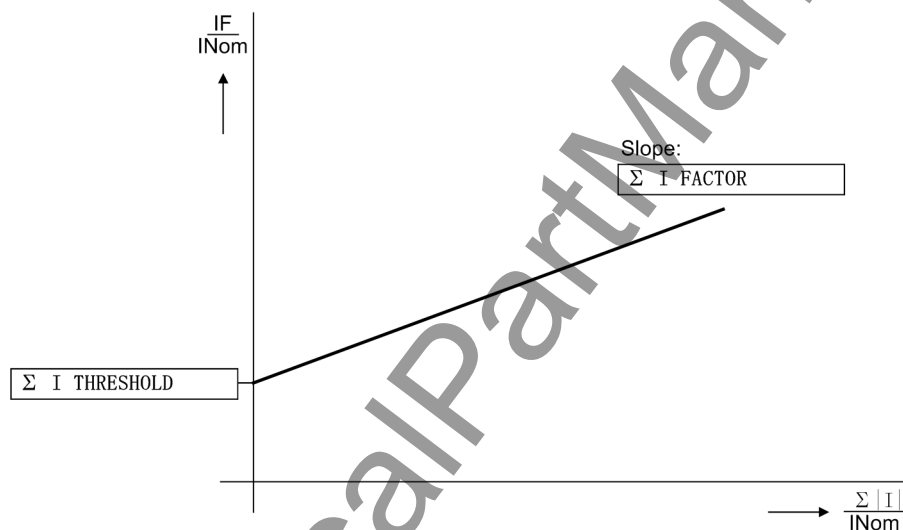
Figure 2-41 Current Sum Monitoring
