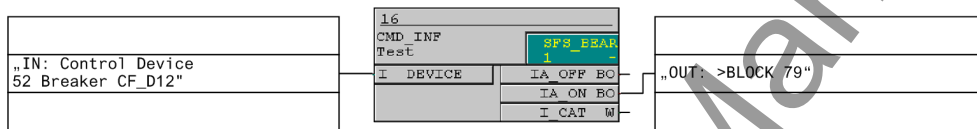
Figure 2-61 Blocking of the automatic reclose function using the internal control function
