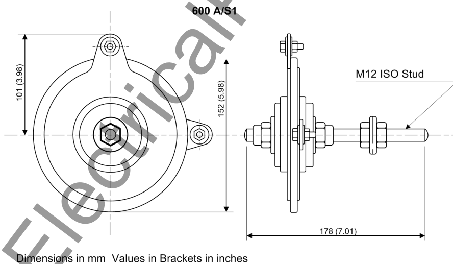
Figure 4-15 Dimensional drawing of the varistor for voltage limiting in high-impedance differential protection
