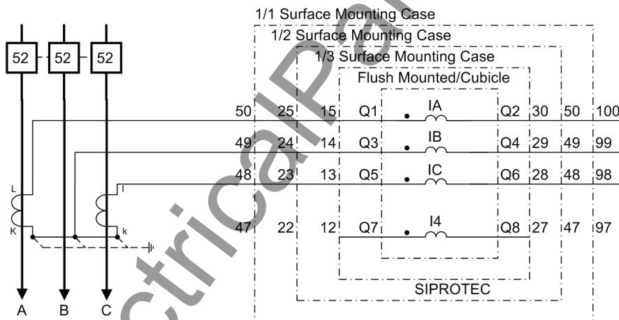
Figure A-10 Current connections to two current transformers - only for ungrounded or compensated networks
