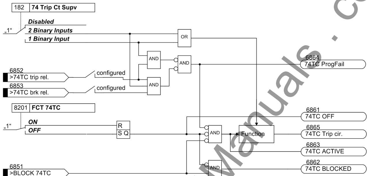
Figure 2-48 Message logic for trip circuit supervision
