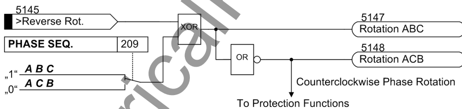
Figure 2-69 Message logic of the phase rotation reversal
