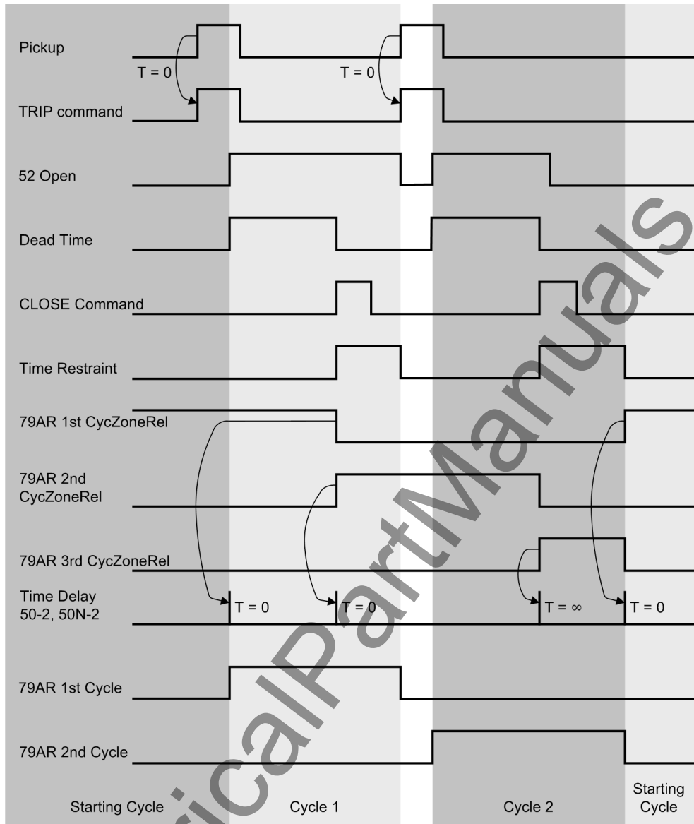
Figure 2-58 Control of protection elements for two-fold, successful auto-reclosure
