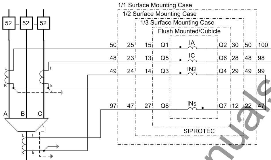
Figure A-13 Current transformer connections to two phase-current transformers and a ground-current transformer; the ground current is taken via the highly sensitive and sensitive ground input.
