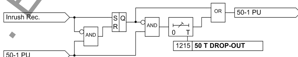
Figure 2-7 Logic diagram of the dropout delay for 50-1
