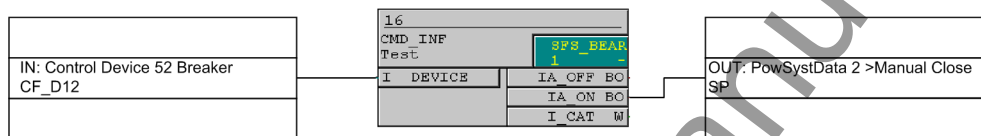
Figure 2-16 Example for the generation of a manual close signal using the internal control function
