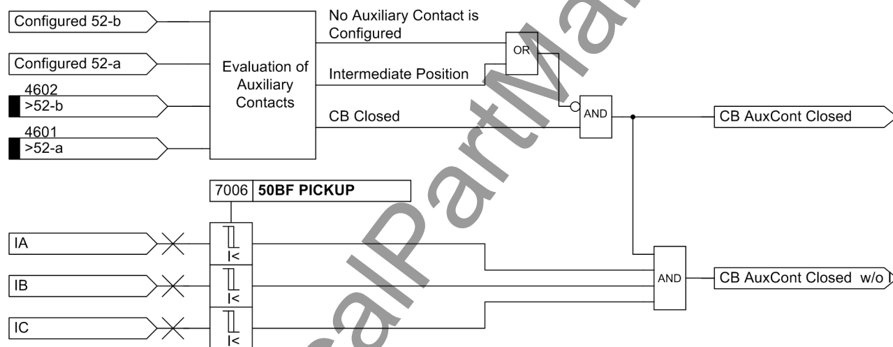
Figure 2-64 Logic diagram for breaker failure protection, monitoring of the circuit-breaker auxiliary contacts
