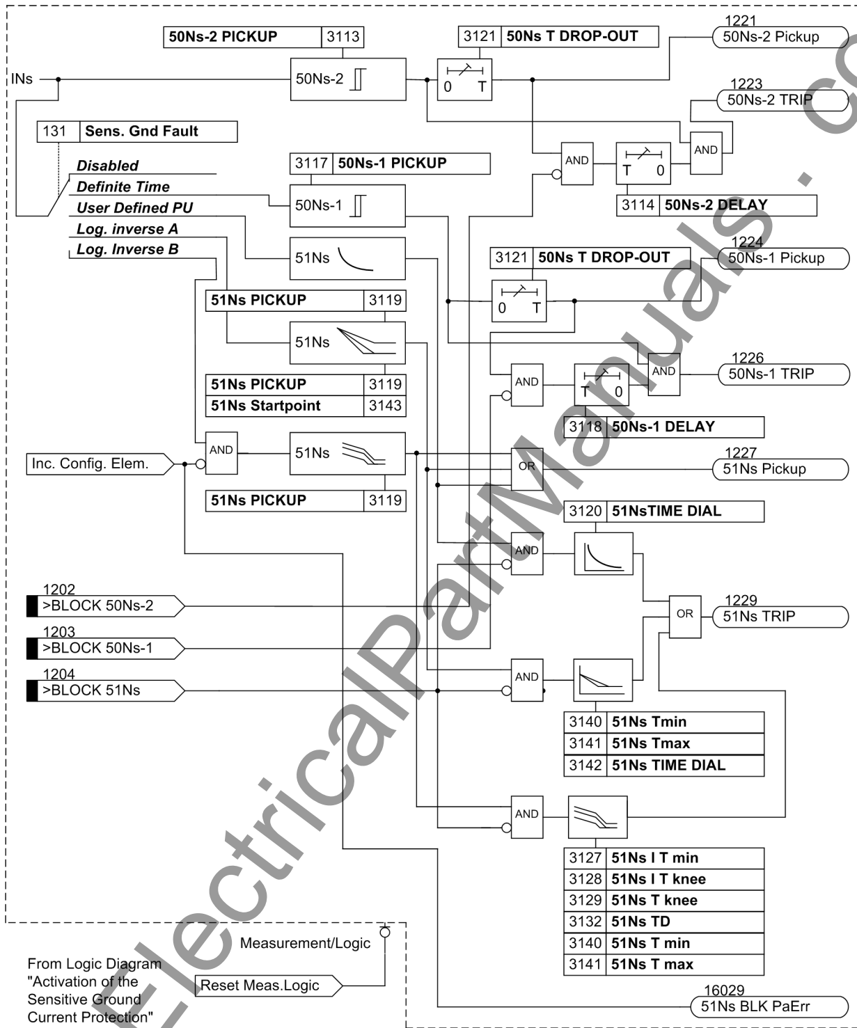
Figure 2-50 Logic diagram of the sensitive ground fault protection
