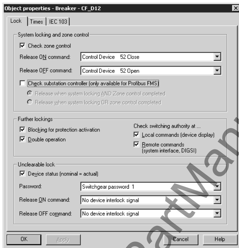
Figure 2-84 DIGSI dialog box for setting the interlocking conditions
