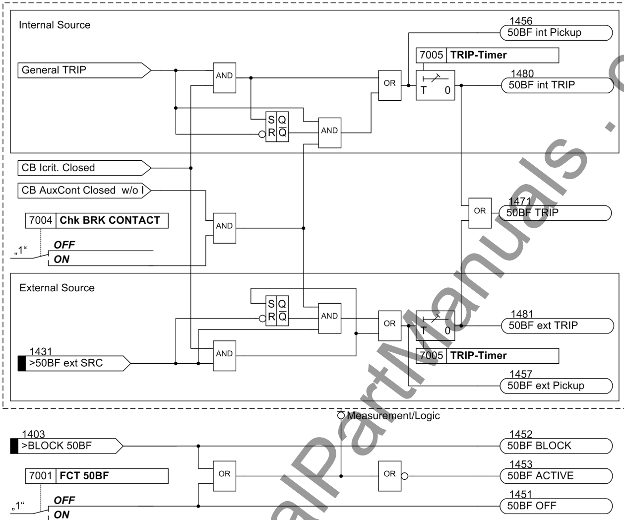
Figure 2-65 Logic diagram of the breaker failure protection
