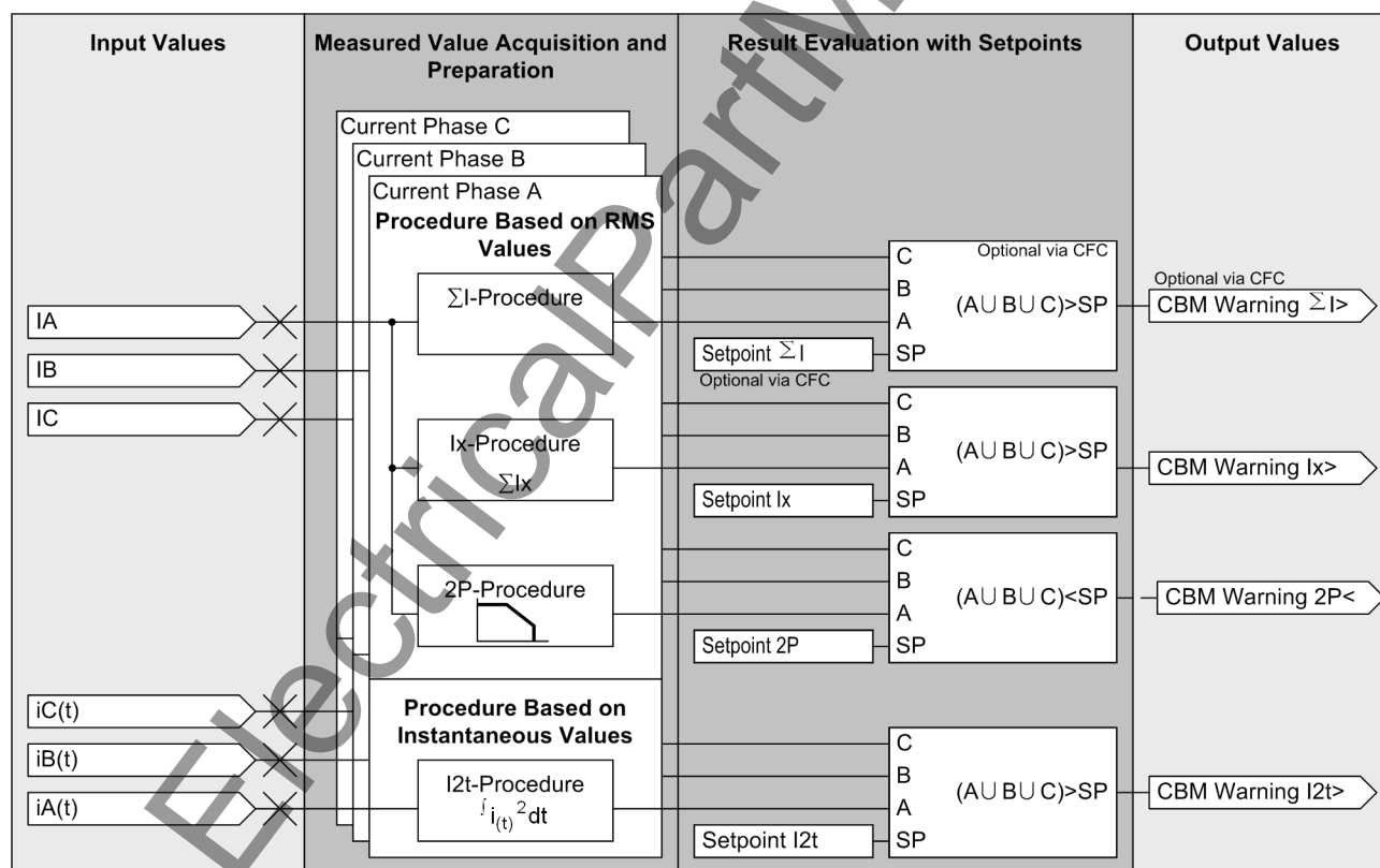
Figure 2-72 Diagram of CB maintenance procedures
