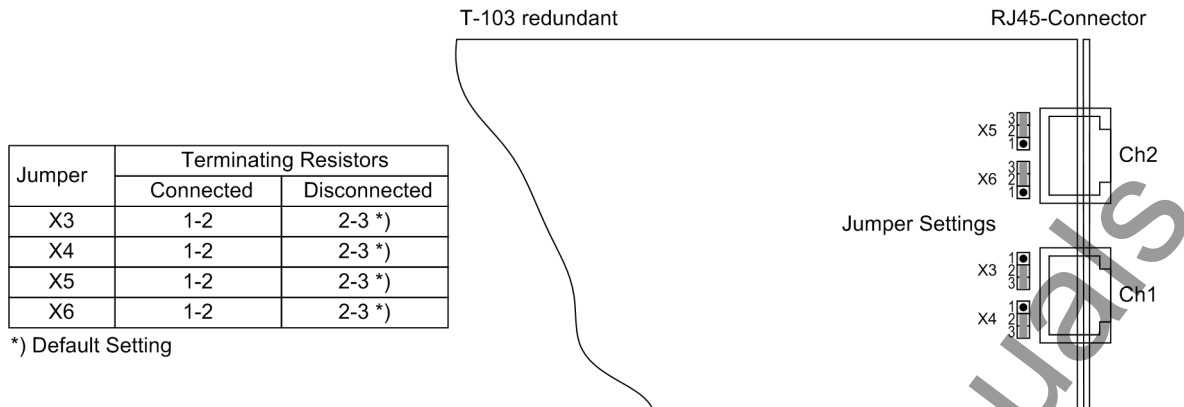
Figure 3-13 Location of the jumpers for configuration of the terminating resistors
