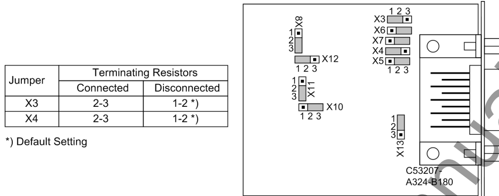
Figure 3-11 Position of terminating resistors and the plug-in jumpers for configuration of the RS485 interface
