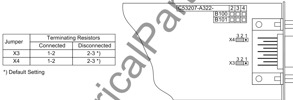
Figure 3-12 Position of the plug-in jumpers for the configuration of the terminating resistors at the Profibus (FMS and DP), DNP 3.0 and Modbus interfaces.
