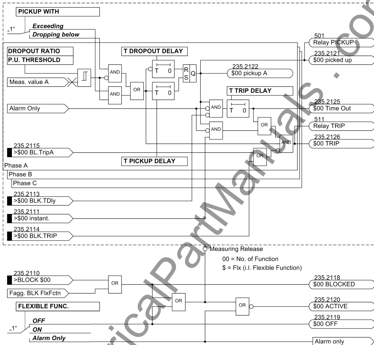
Figure 2-67 Logic diagram of flexible protection functions
