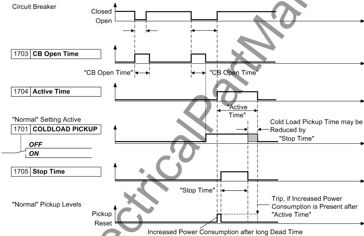
Figure 2-17 Timing charts of the dynamic cold load pickup function
