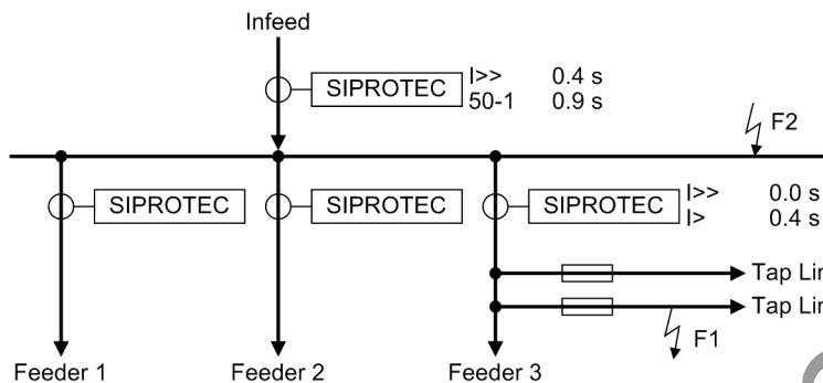
Figure 2-59 Zone sequencing with a fault occurring at Tap Line #5 and the busbar
