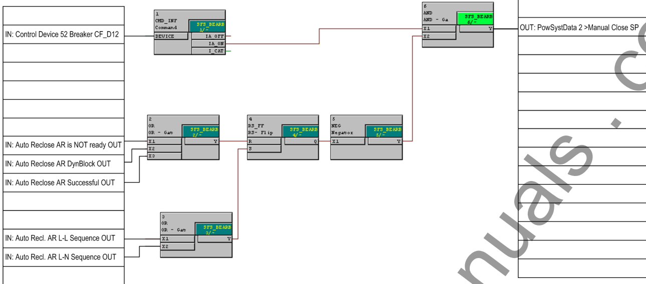
Figure 2-60 CFC logic for Manual Close with automatic reclosing via control
