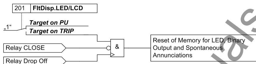
Figure 2-122 Logic diagram of the no-trip-no-flag feature (trip-dependent alarms)
