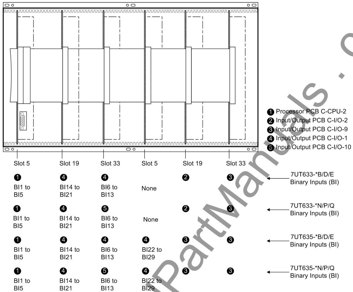
Figure 3-4 Front view with housing size 1/1 after removal of the front panel (simplified and scaled down)
