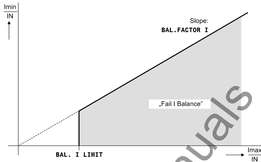
Figure 2-114 Current Symmetry Monitoring
