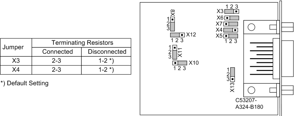
Figure 3-13 Position of terminating resistors and the plug-in jumpers for configuration of the RS485 interface
