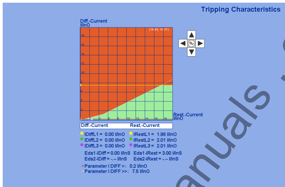
Figure 3-28 Differential and Restraint Currents - Example of Plausible Measurements
