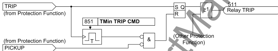
Figure 2-121 Storage and termination of the trip command (simplified)
