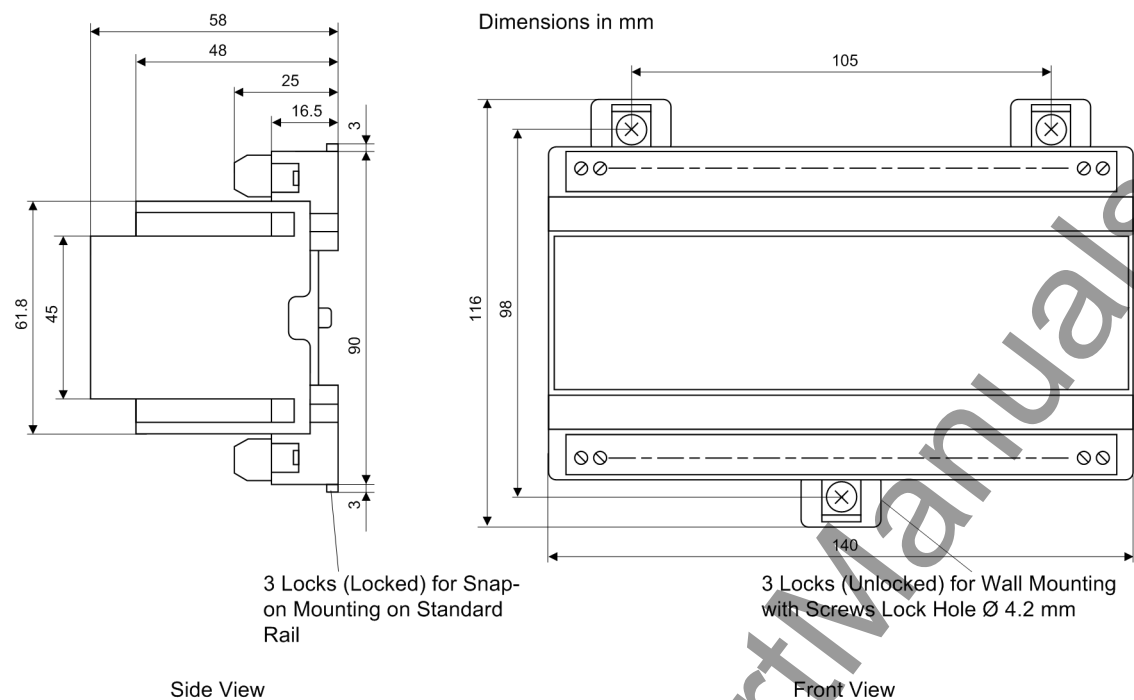
Figure 4-24 Dimensions of the Remote Temperature Detection Unit 7XV5662-*AD10-0000
