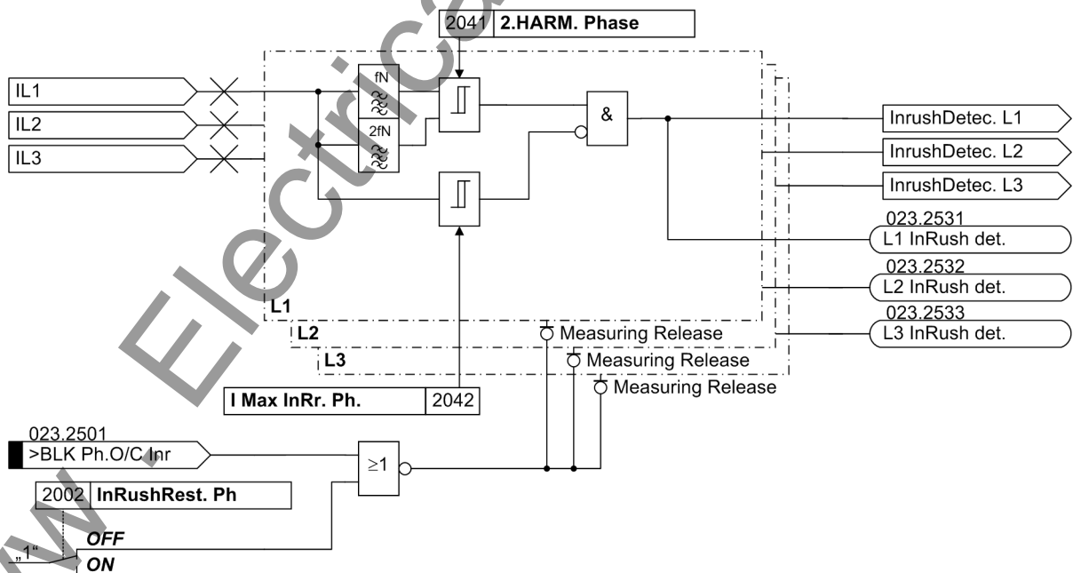
Figure 2-72 Logic diagram of the inrush restraint feature — example for phase currents (simplified)
