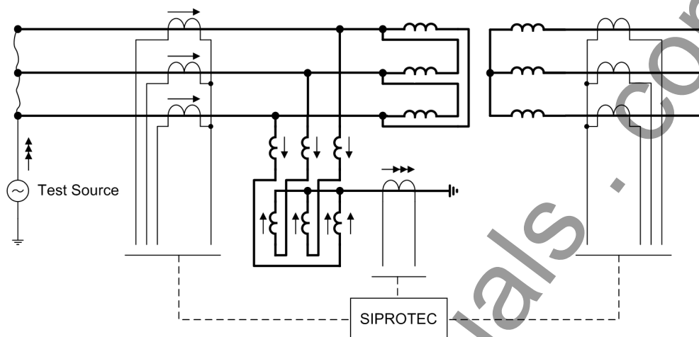
Figure 3-34 Zero sequence current measurement on a delta winding with neutral earthing reactor within the protected zone
