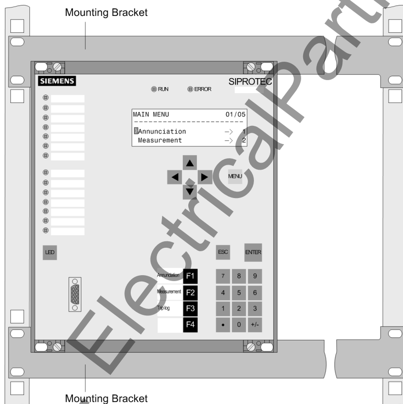
Figure 3-18 Installation of a 7UT613 in a rack or cubicle (housing size 1½) — example
