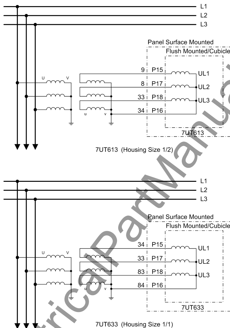
Figure A-27 Voltage connections to three wye-connected voltage transformers (only in 7UT613 and 7UT633)
