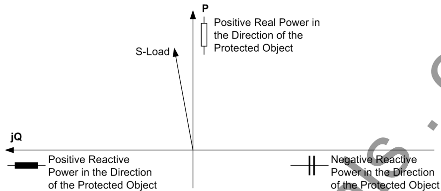
Figure 3-41 Apparent power
