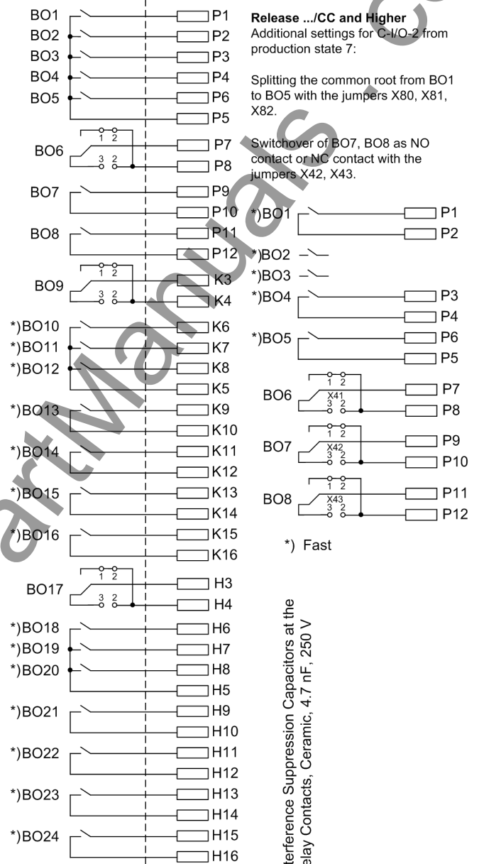
Figure A-2 General diagram 7UT633 (panel flush and cubicle mounting)
