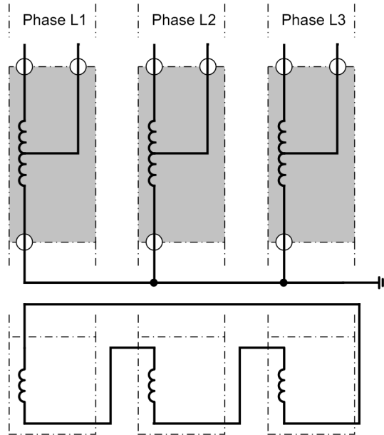
Figure 2-1 Transformer bank, consisting of 3 single-phase auto-transformers with current comparison via each single phase
