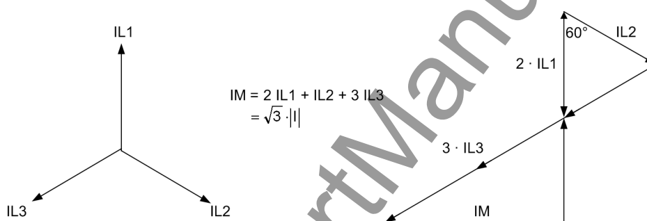
Figure 2-47 Summation of the currents in the summation transformer on connection L1-L2-L3
