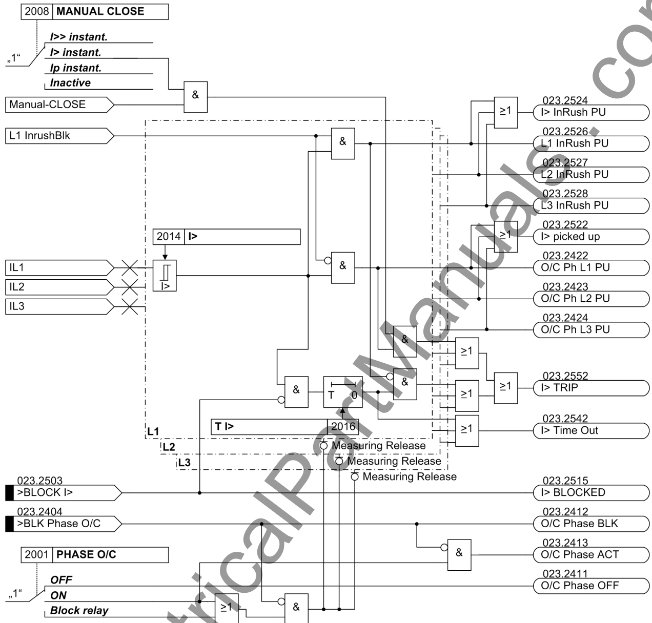
Figure 2-67 Logic diagram of the overcurrent stage I&gt; for phase currents (simplified)
