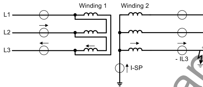
Figure 2-29 Example for an earth fault outside a transformer with current distribution
