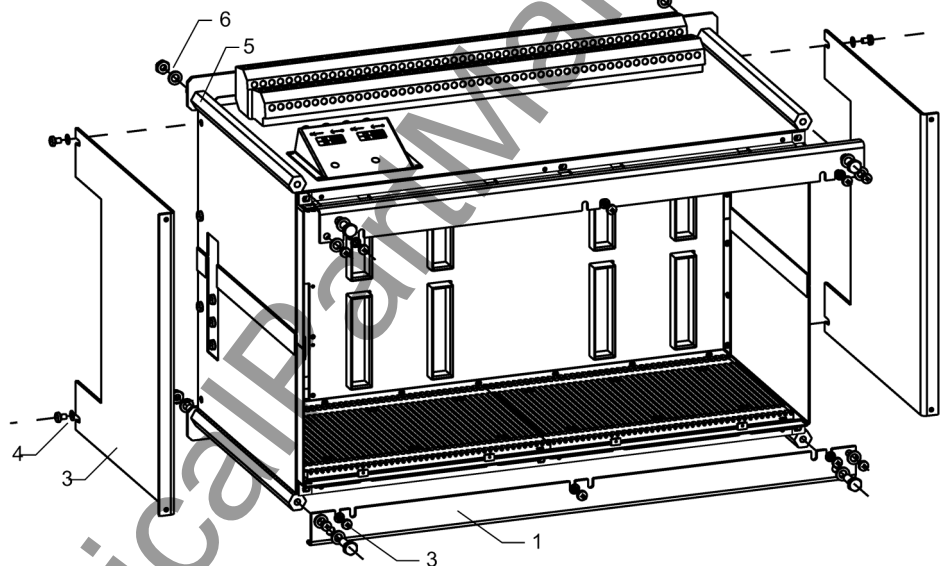
Figure 3-20 View of a housing with transport protection (without front cover nor boards)
