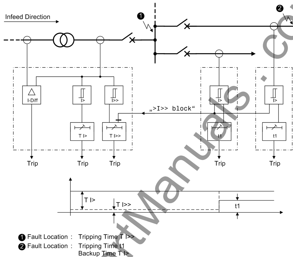
Figure 2-74 Fast busbar protection using reverse interlock — principle
