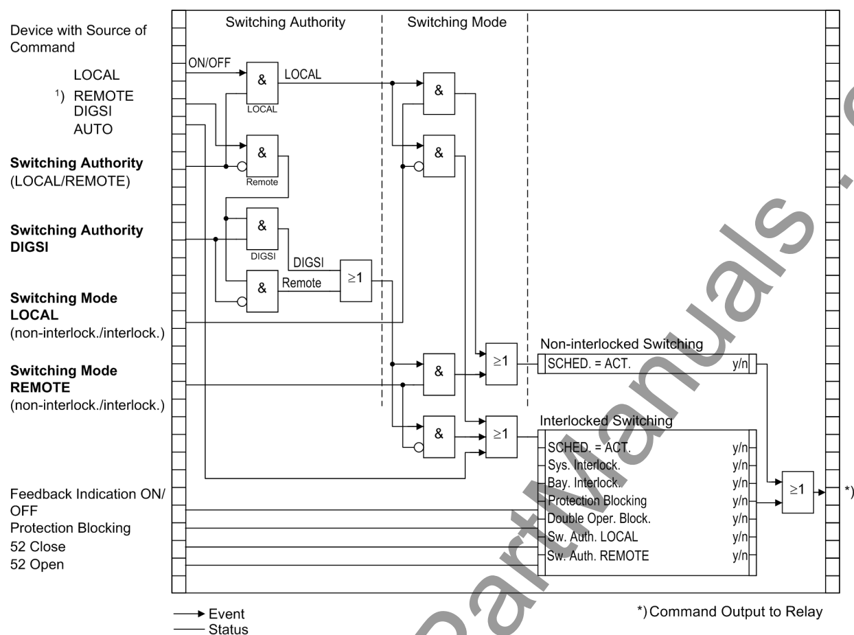
Figure 2-127 Standard interlockings
