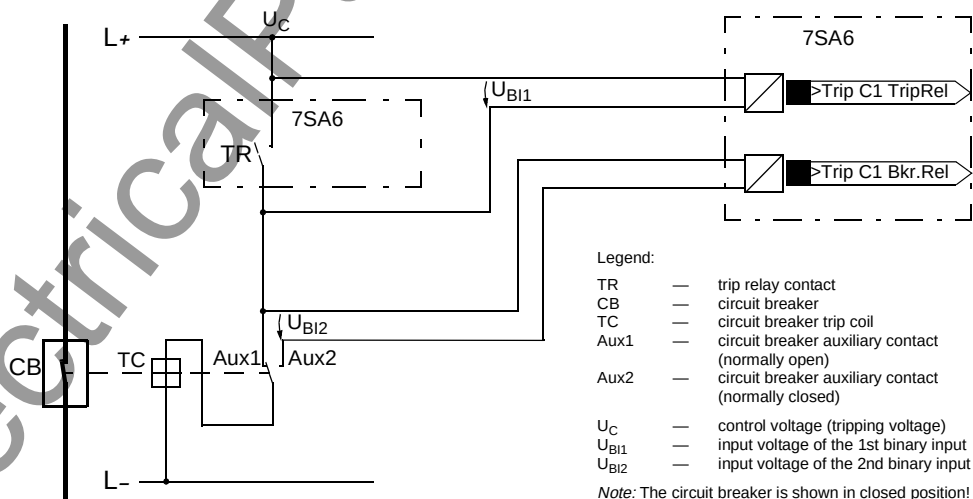
Figure 6-134 Trip circuit supervision operating principle with two binary inputs
