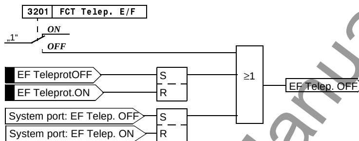
Figure 6-70 Switching on and off of the signal transmission logic
