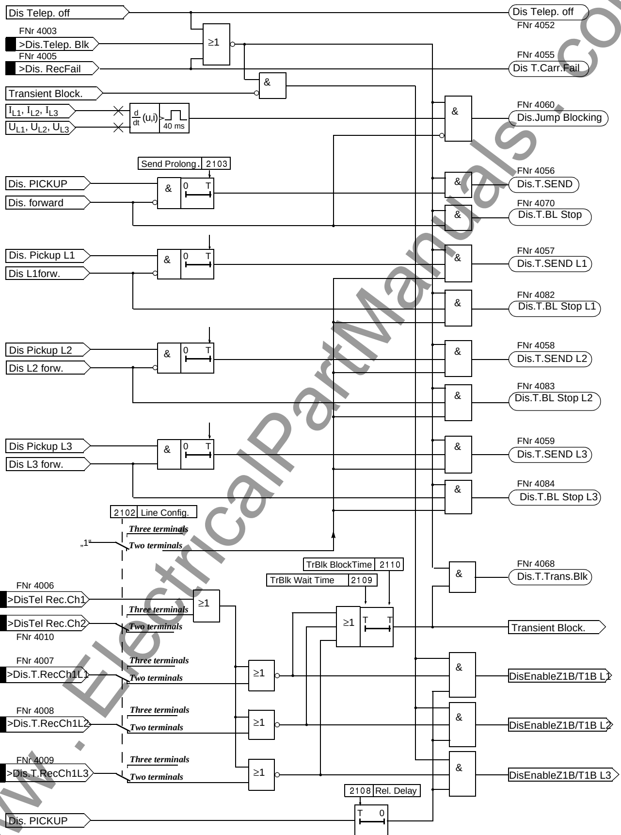
Figure 6-55 Logic diagram of the blocking scheme (one line end)
