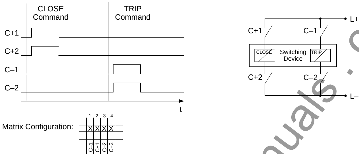
Figure 5-9 Double command with double contacts (with 4 relays)
