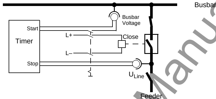
Figure 8-28 Measuring the circuit breaker closing time
