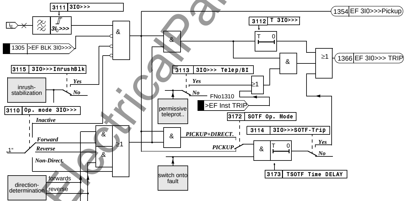
Figure 6-61 Logic diagram of the 3I_0>>> -stage
