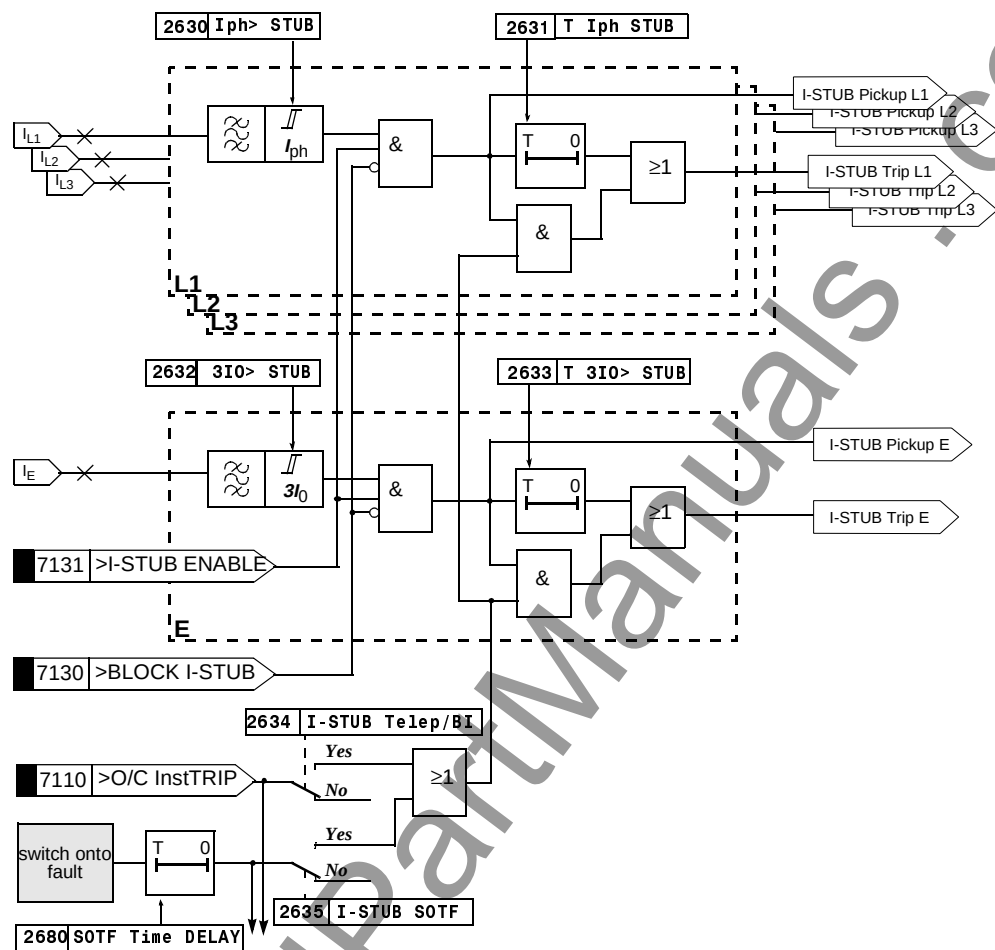
Figure 6-86 Logic diagram of the stub protection
