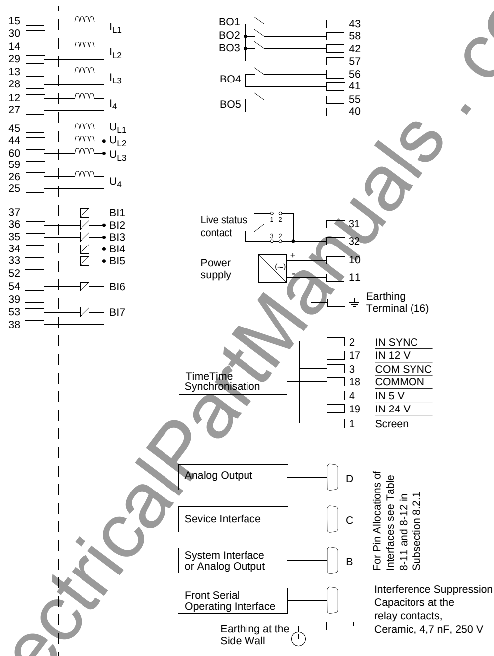
Figure A-9 General Diagram 7SA610*--*F (Panel Surface Mounting)
