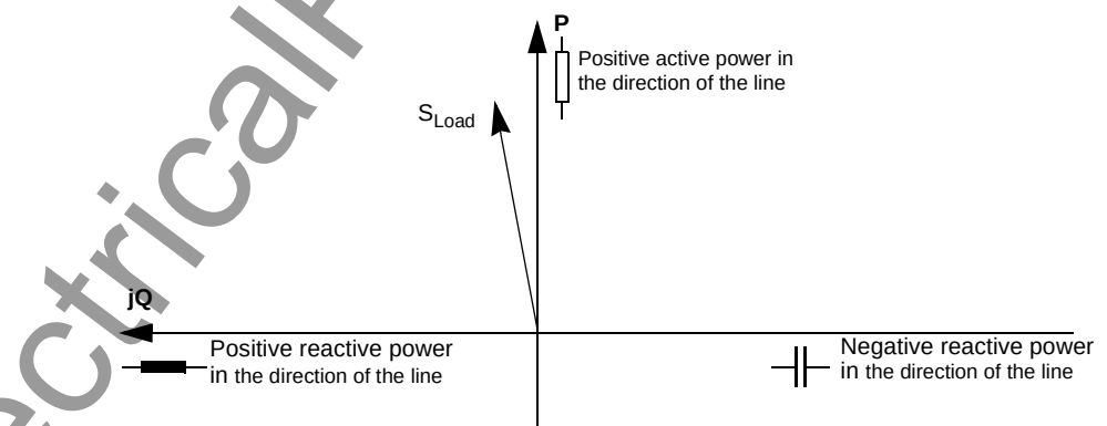
Figure 8-23 Complex (apparent) power
