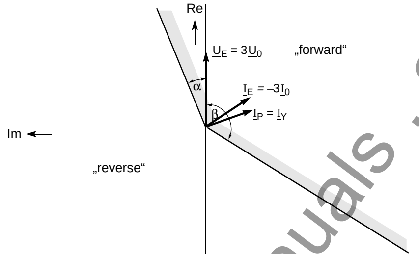
Figure 6-67 Directional characteristic using I_Y as polarization quantity
