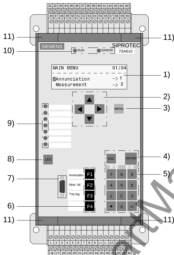
Figure 2-21 Front view of a 7SA61, housing size \frac{1}{3} , for panel surface mounting without
