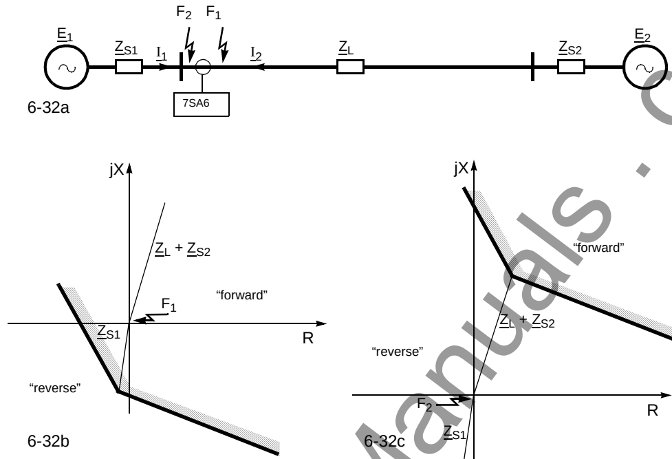
Figure 6-32 Directional characteristic with quadrature or memorized voltages
