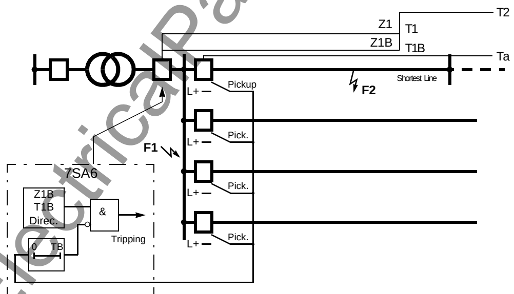
Figure 6-57 Reverse interlocking — functional principle and grading example
