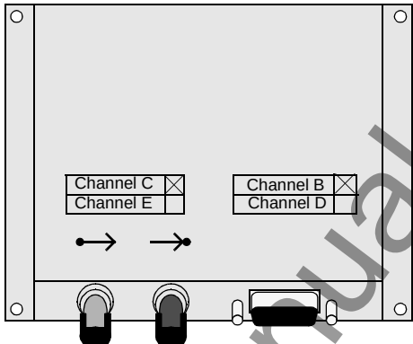
Figure 2-28 Inclined housing with optical communication interface B and DSUB socket for Profibus interface
