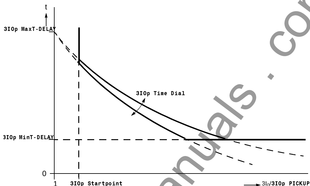
Figure 6-68 Setting parameter characteristics in the logarithmic-inverse curve
