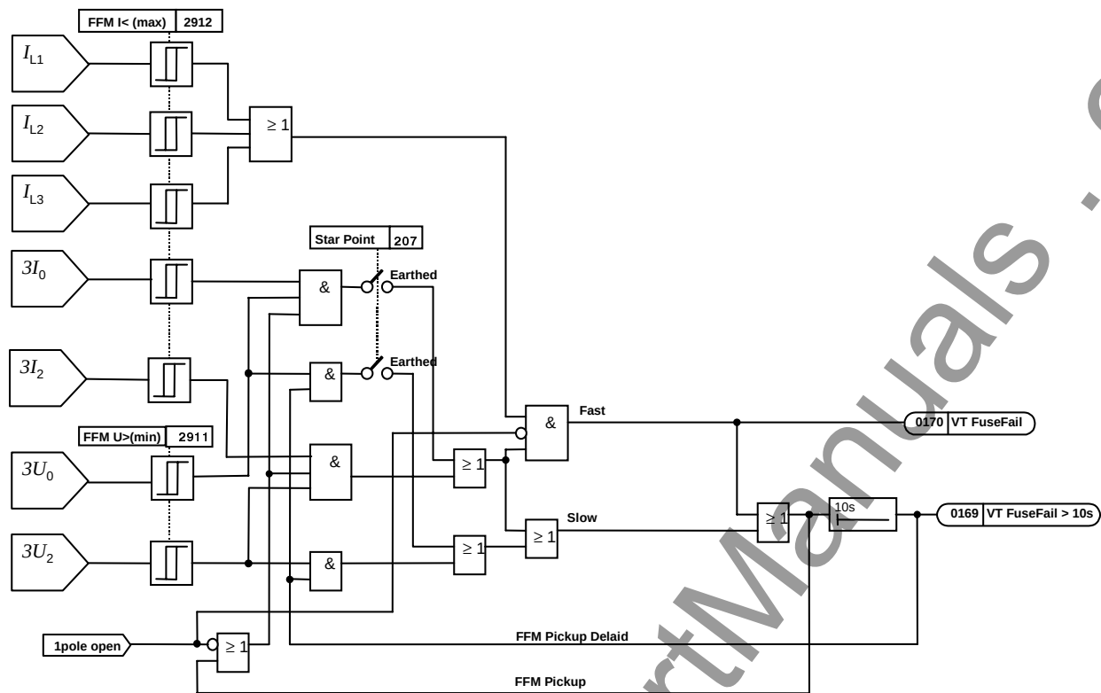
Figure 6-133 Logic diagram of the fuse failure monitor with zero and negative sequence system
