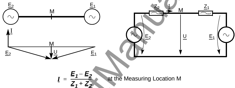
Figure 6-39 Power swing
