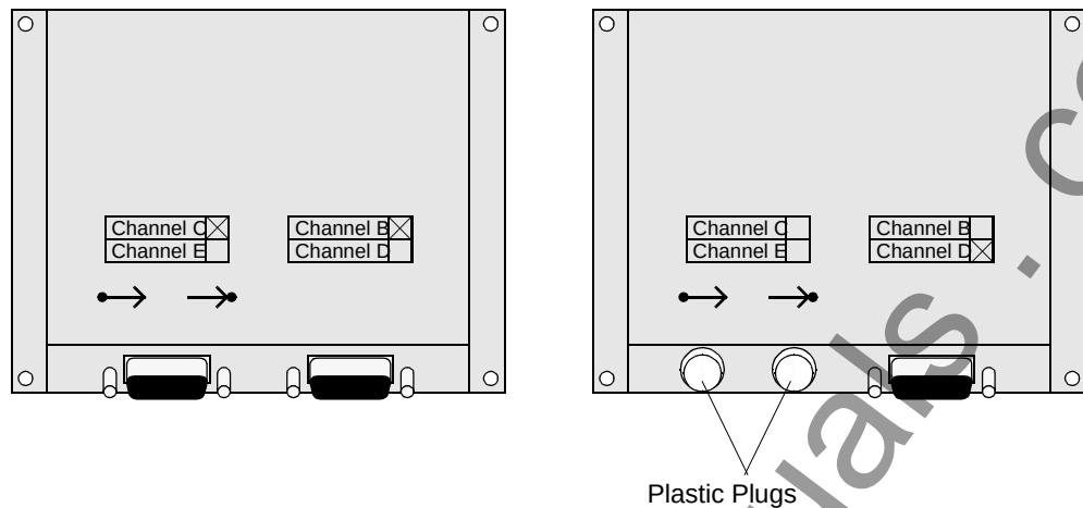
Figure 2-29 Inclined housing with 9-pin DSUB socket
