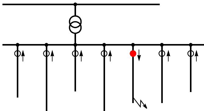
Figure 6-90 Faulted line location in radial network
