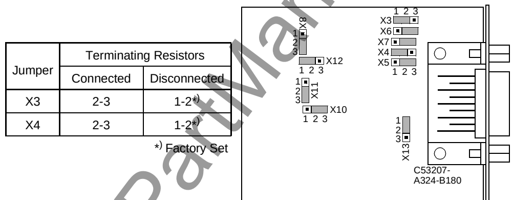
Figure 8-18 Location of the jumpers for the configuration of terminating resistors of the RS 485 interface
