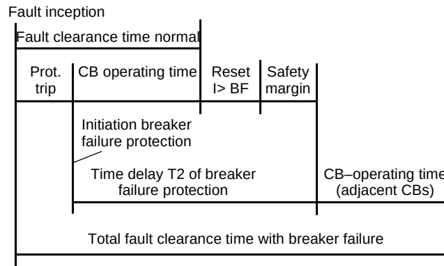
Figure 6-128 Time sequence example for normal clearance of a fault, and with circuit breaker failure, using single-stage breaker failure protection
