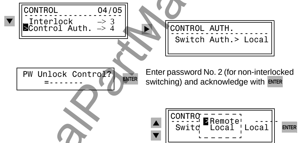
Figure 7-55 Setting Switching Authority with the Operator Control Panel
