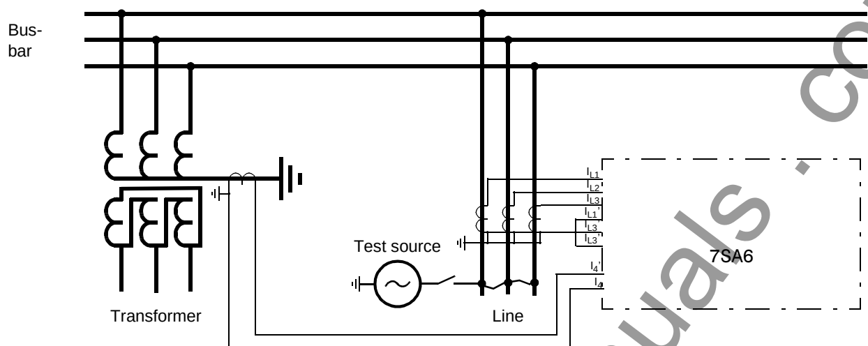
Figure 8-27 Polarity check of I_4 , example with earth current from a power transformer star-point
