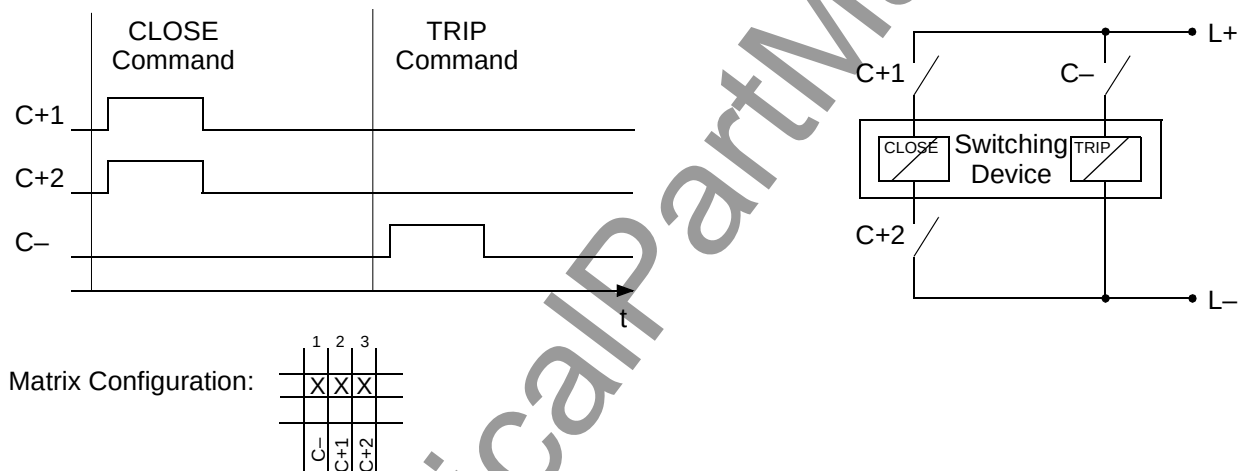
Figure 5-10 Double command with double and single contacts (with 3 relays)
