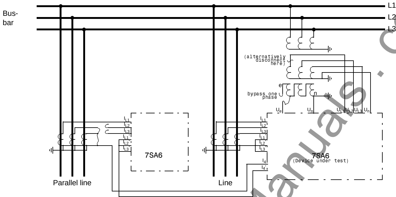
Figure 8-26 Polarity check of I_4 , example with earth current of a parallel line
