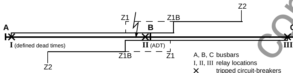
Figure 6-96 Example of adaptive dead time (ADT)
