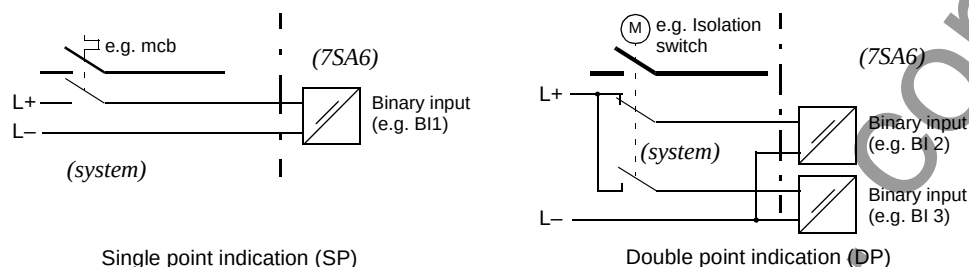
Figure 5-3 Input indications
