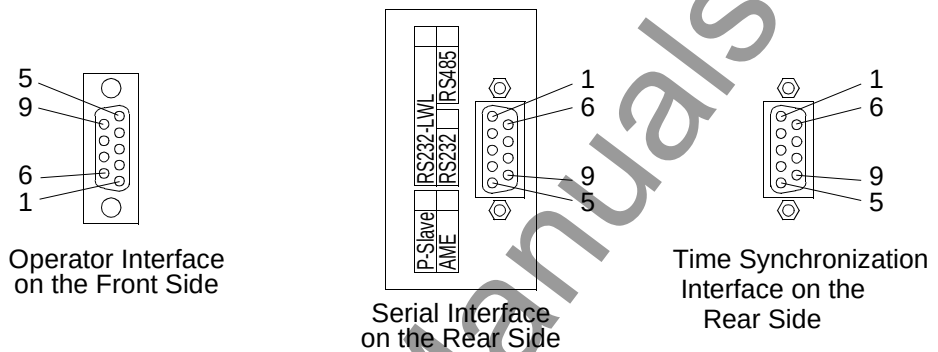
Figure 2-43 9 pin D-subminiature connectors
