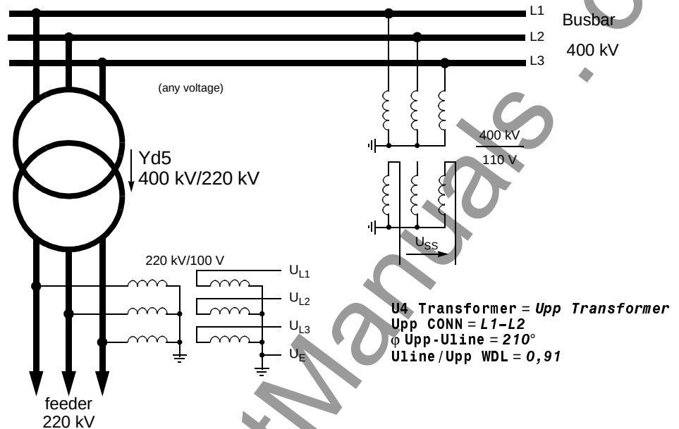
Figure 6-9 Busbar voltage, measured across a power transformer
