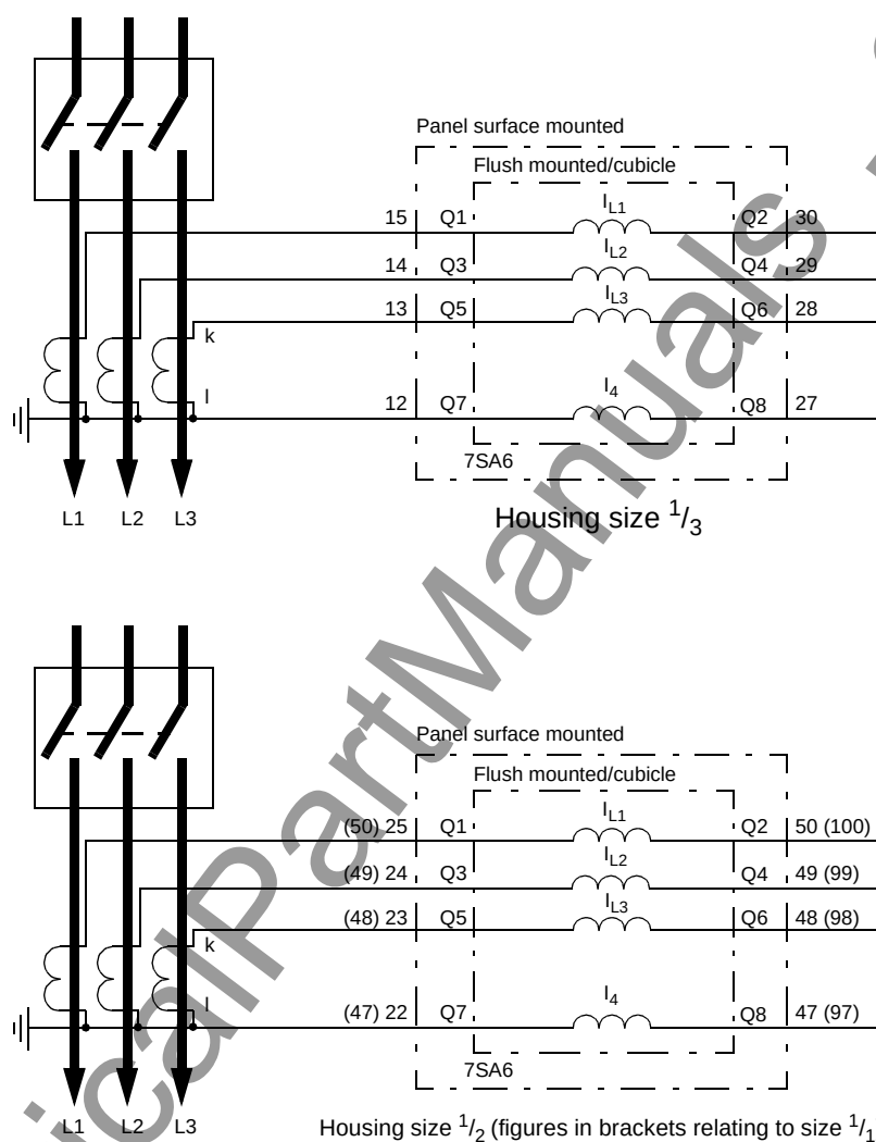
Figure A-20 Current connections to three current transformers with a star-point connection for earth current (residual 3I_0 neutral current), normal circuit layout — appropriate for all networks
