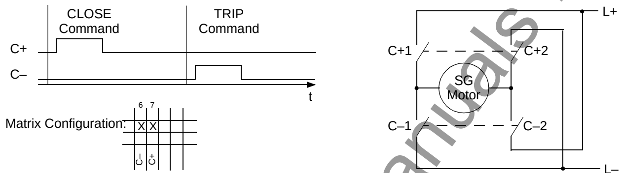
Figure 5-11 Double command motor control (anti-clockwise rotation / clockwise rotation) via two power relays with two contacts each
