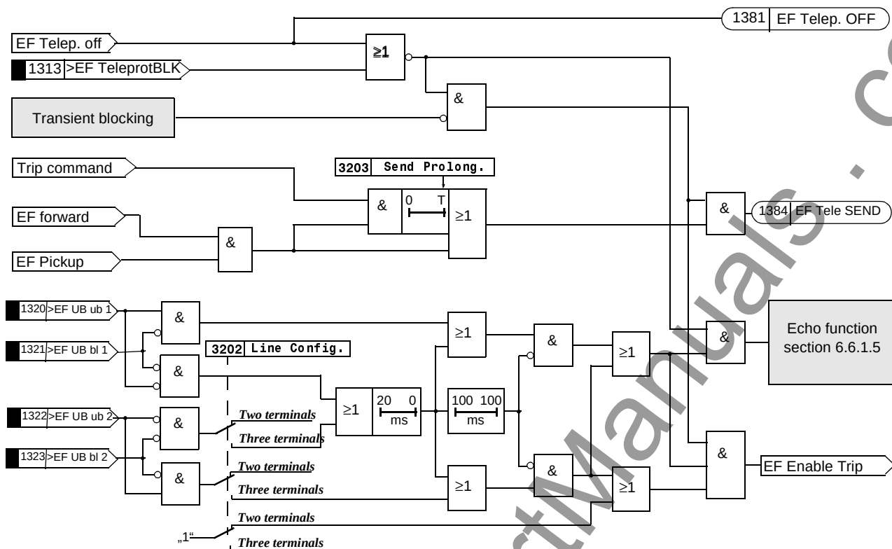
Figure 6-74 Logic diagram of the unblocking scheme (one line end)
