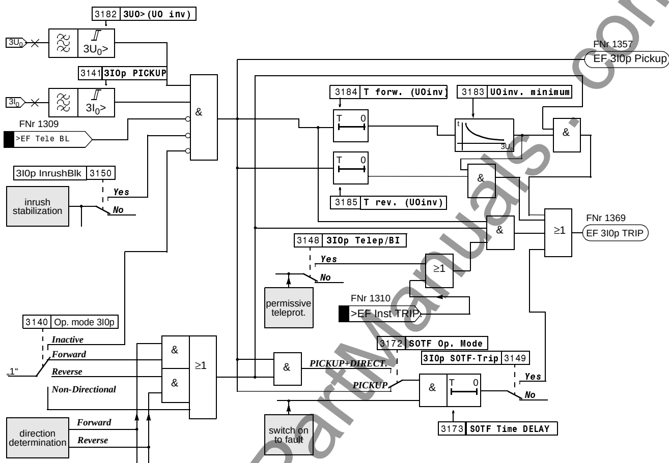
Figure 6-64 Directional zero voltage time protection with non-directional back-up stage
