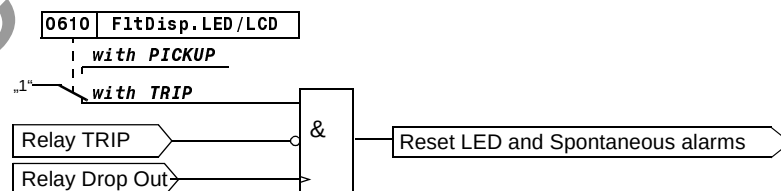
Figure 6-146 Logic diagram of the trip dependent messages
