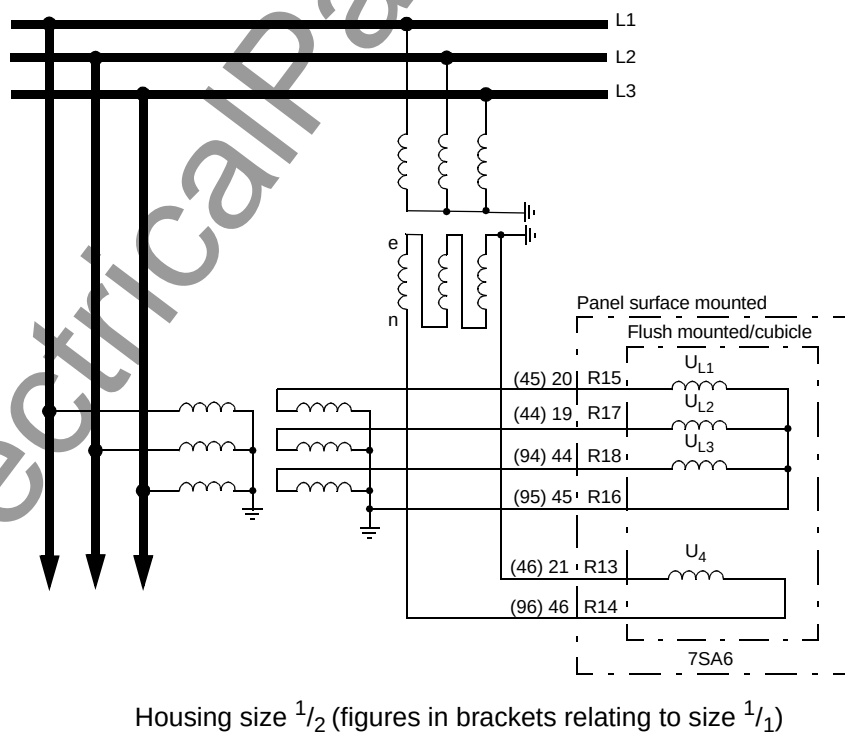
Figure A-26 Voltage connections to three Wye-connected voltage transformers with additional open-delta windings (e–n–winding) from the busbar
