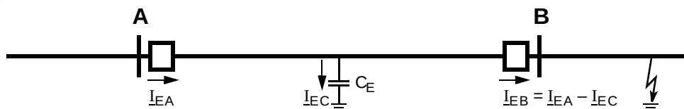
Figure 6-79 Possible current distribution during external earth fault
