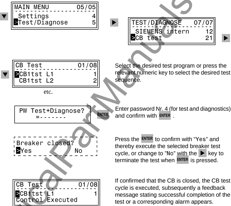
Figure 7-42 Circuit breaker trip test cycle from the front of the device
