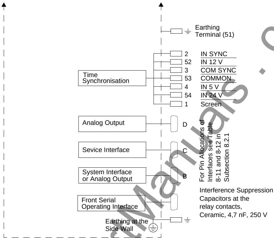
Figure A-13 General Diagram 7SA6*2*-*F (Panel Surface Mounting)
