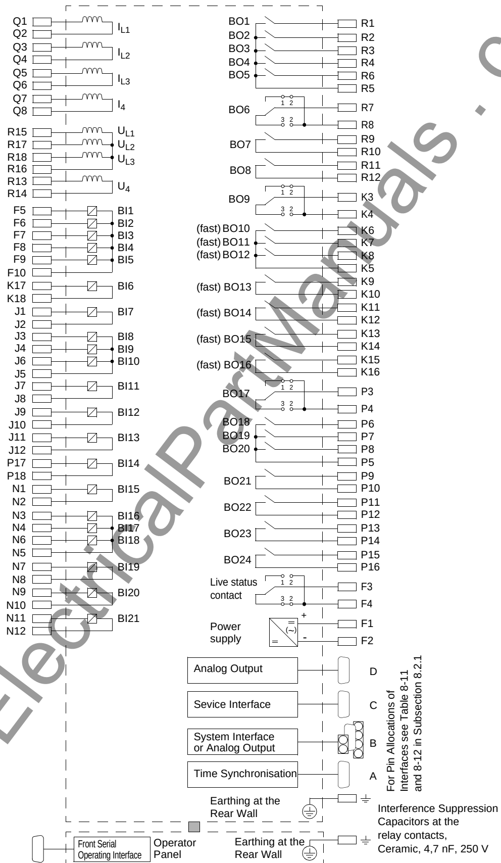
Figure A-17 General Diagram 7SA642*--*A/J (Mounting with detached operator panel)
