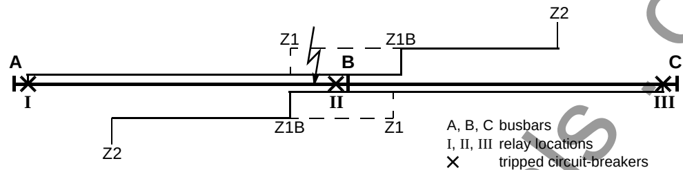
Figure 6-95 Example of a reduced dead time (RDT)
