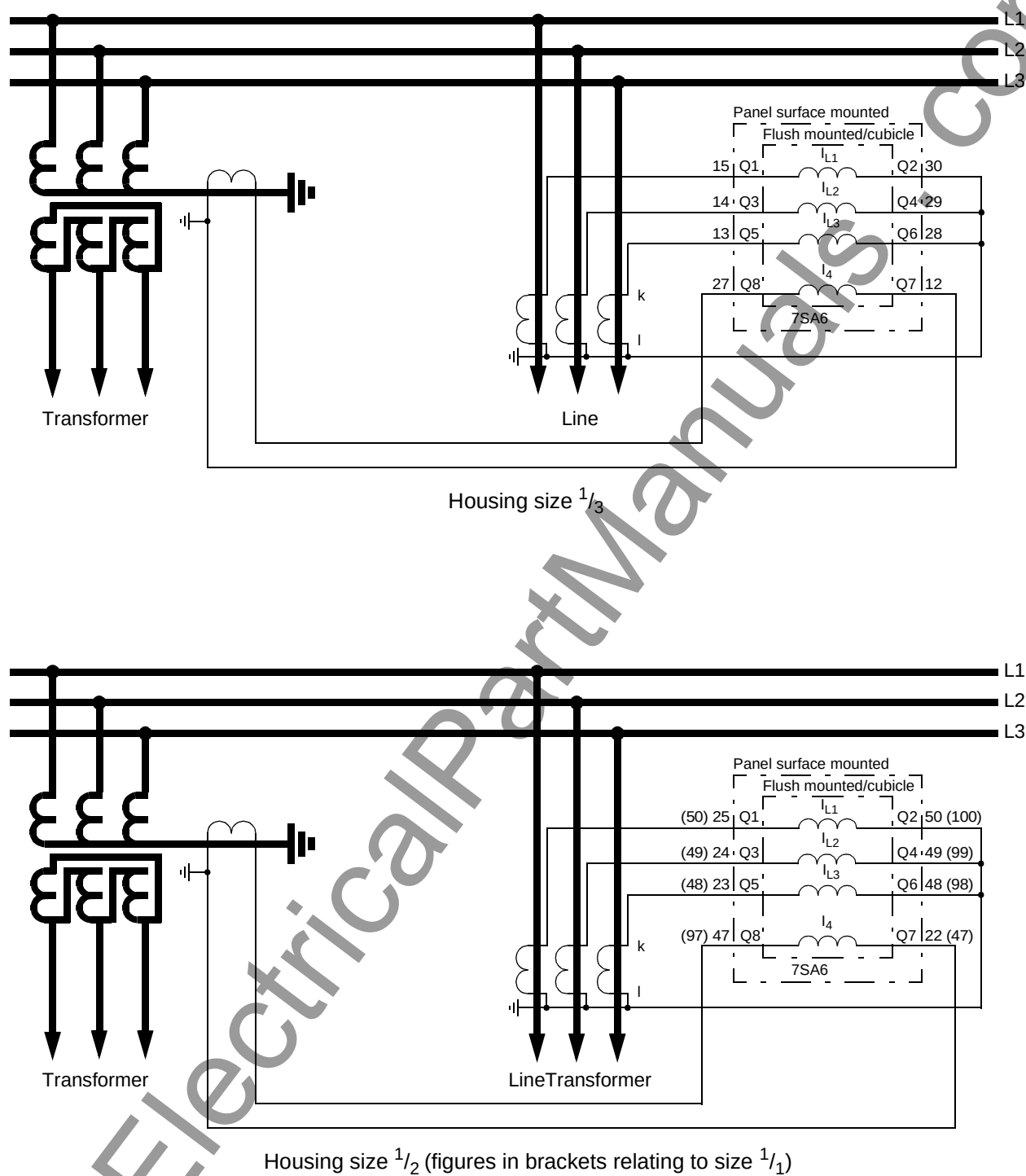
Figure A-23 Current connections to three current transformers and earth current from the star-point connection of an earthed power transformer (for directional-controlled earth fault protection)
