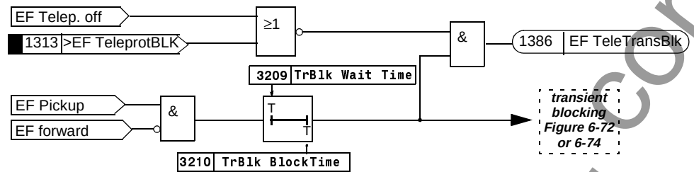
Figure 6-77 Transient blocking for a directional comparison and directional unblocking schemes
