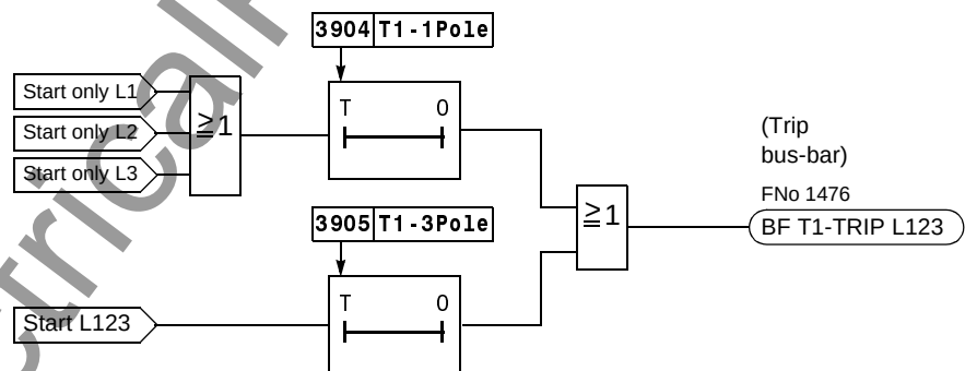
Figure 6-121 Single-stage breaker failure protection with different delay timers
