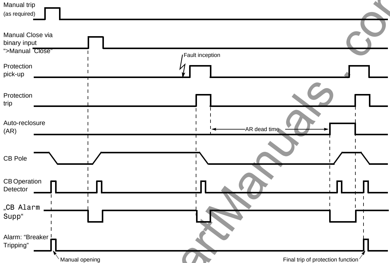
Figure 6-145 Breaker tripping alarm suppression — sequence examples
