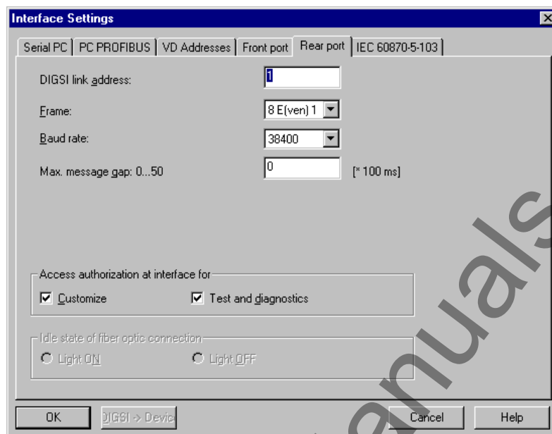
Figure 5-52 DIGSI® 4, Settings for the rear port — example
