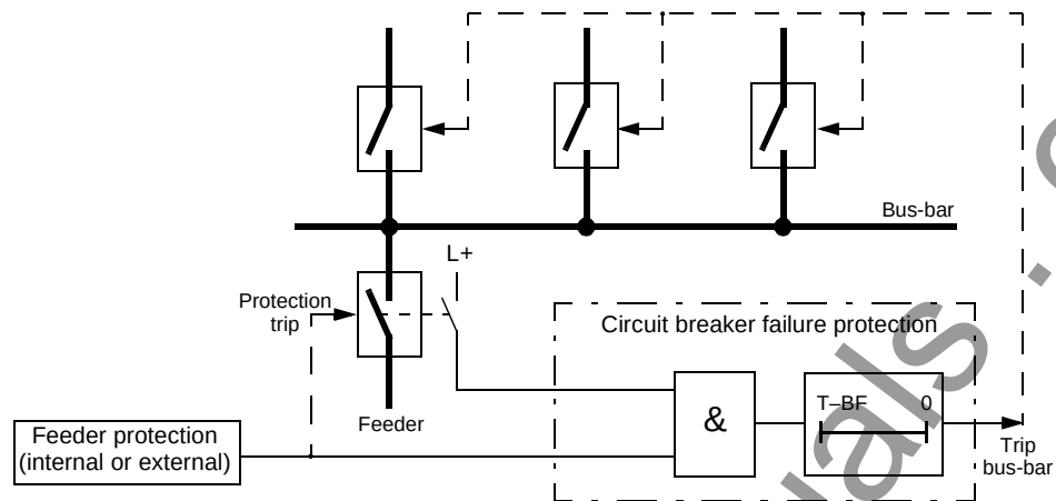
Figure 6-112 Simplified function diagram of circuit breaker failure protection controlled by circuit breaker auxiliary contact
