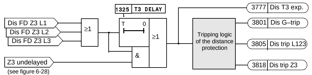
Figure 6-36 Tripping logic for the 3rd Zone
