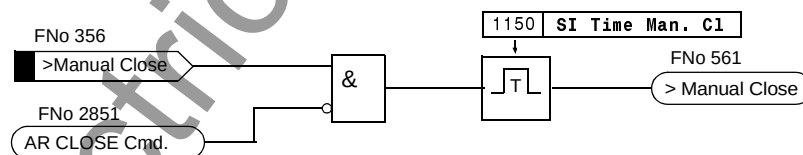
Figure 6-138 Logic diagram of the manual closure handling
