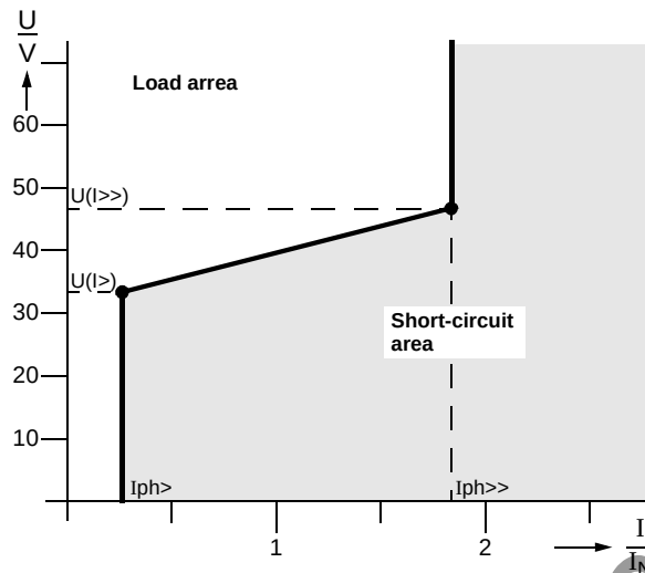
Figure 6-19 U/I characteristic
