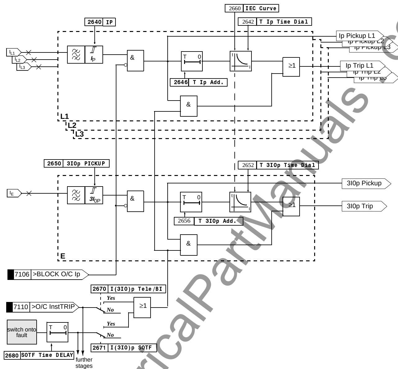
Figure 6-84 Logic diagram of the I_p -stage (inverse time overcurrent protection IDMT) — illustration for IEC-curves
