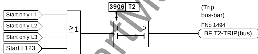
Figure 6-120 Single-stage breaker failure protection with common phase initiation
