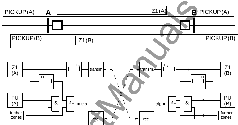
Figure 6-42 Operation scheme of the permissive underreach transfer trip method via pickup
