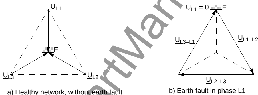
Figure 6-88 Earth fault in non-earthed neutral network
