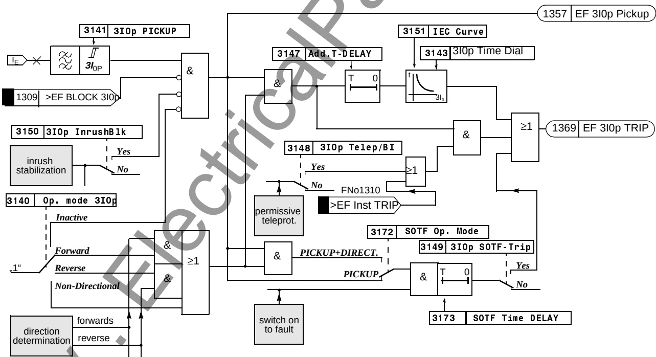
Figure 6-62 Logic diagram of the 3I_{0p} -stage (inverse time overcurrent protection), for example IEC curves
