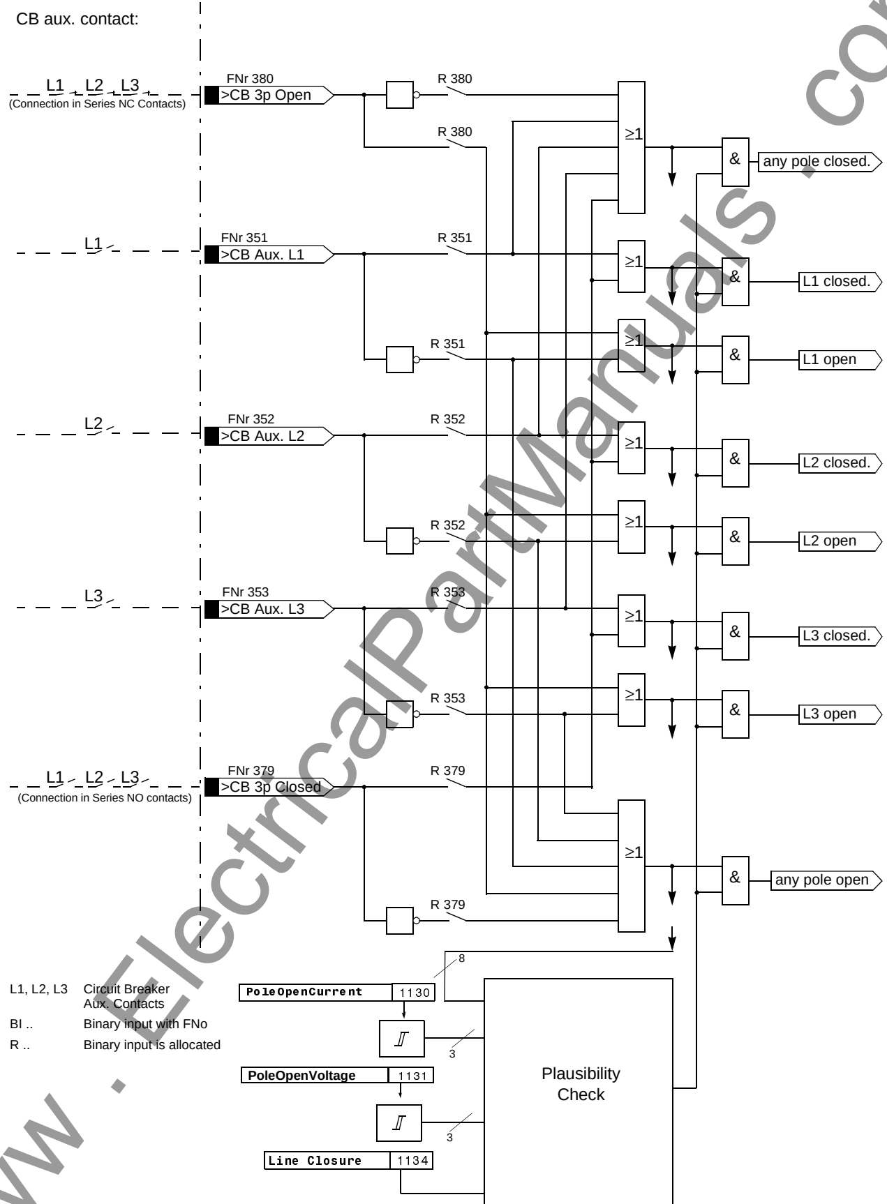
Figure 6-141 Circuit breaker position logic
