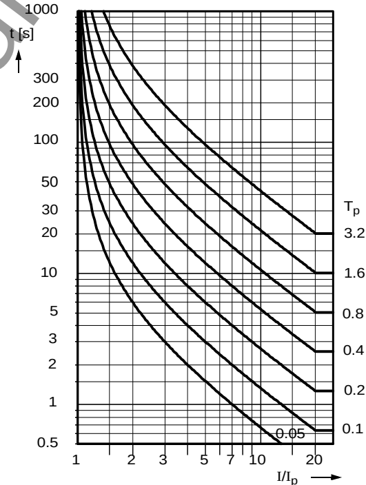
Longtime inverse:
