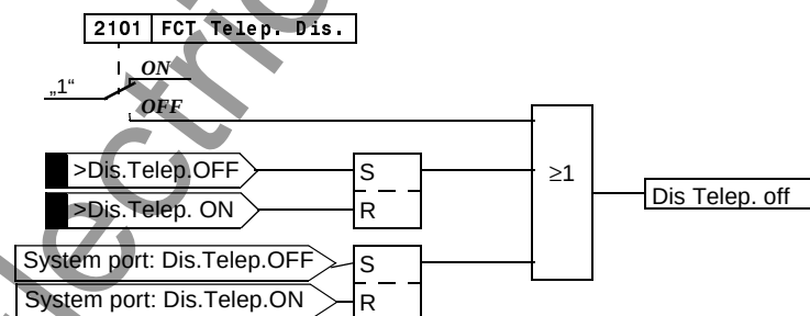
Figure 6-41 Switching on and off of the teleprotection
