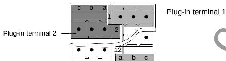
Figure 2-39 Correlation between plug-in terminals and connection numbers/letters
