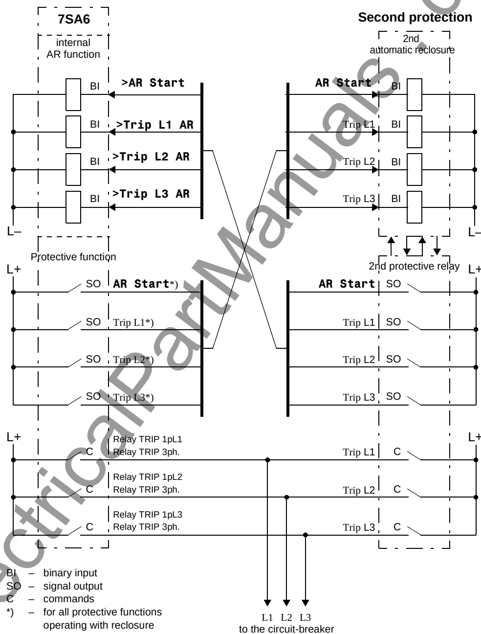
Figure 6-102 Connection example for 2 protection devices with 2 automatic reclosure functions
