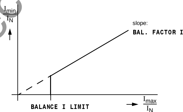
Figure 6-131 Current symmetry monitoring
