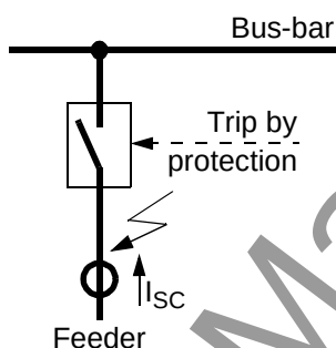
Figure 6-124 End fault between circuit breaker and current transformers
