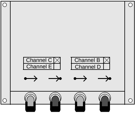
Figure 2-27 Inclined housing with optical communication interfaces (example: channel B and C fitted)
