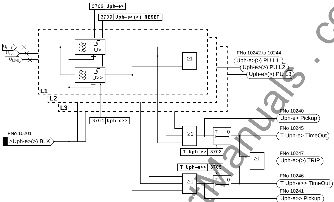
Figure 6-105 Logic diagram of the overvoltage protection for phase voltages
