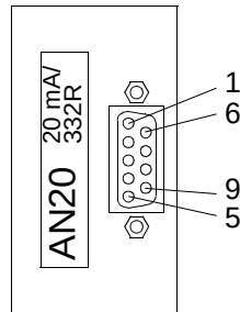
Figure 2-20 9 pin D-subminiature connectors
