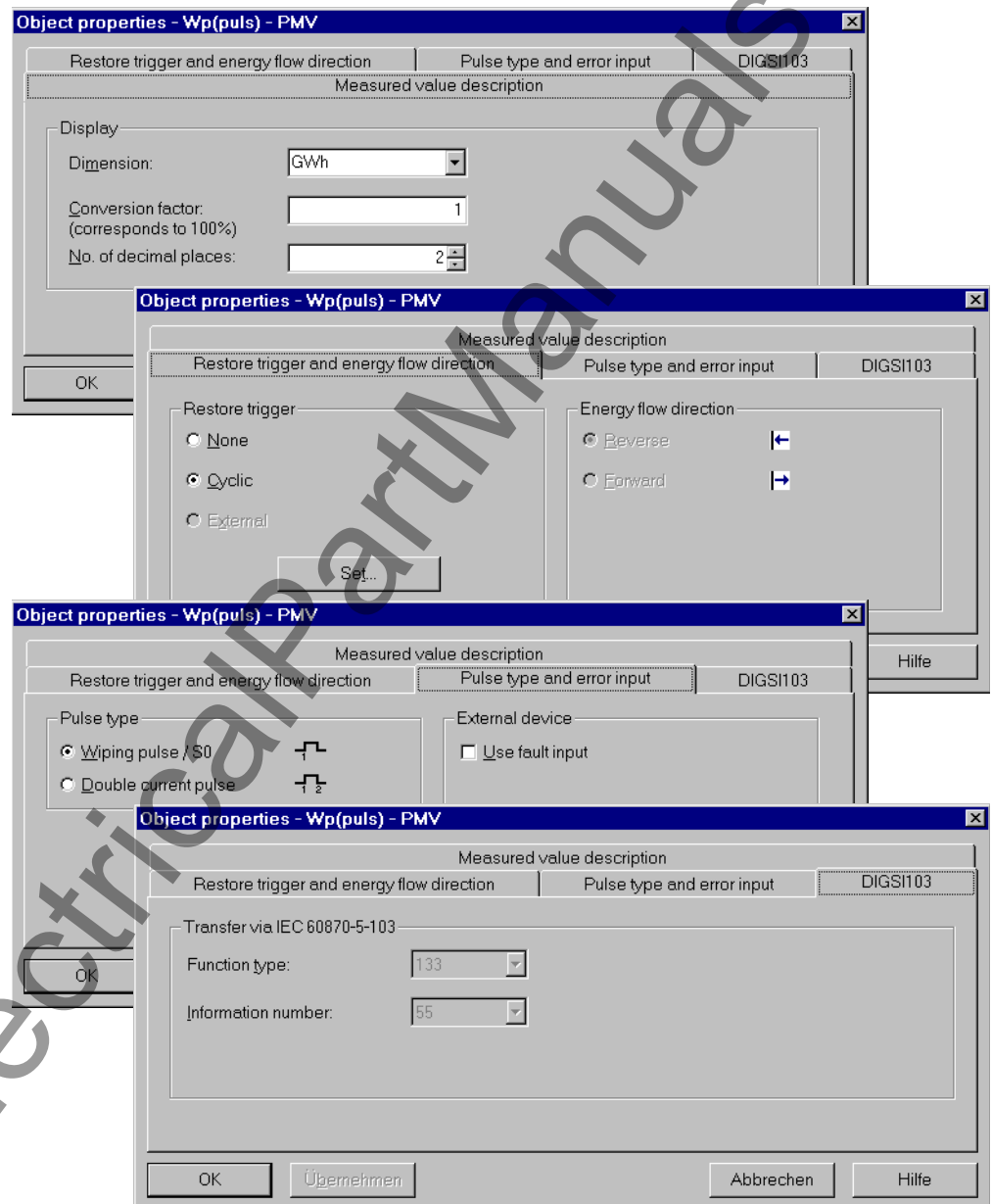
Figure 5-20 Information Properties, Example for Information Type "Pulse Measured Value" (PMV)
