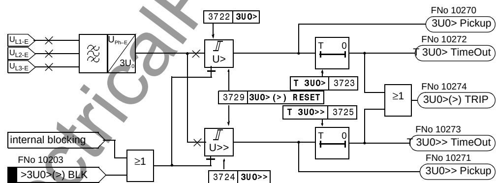
Figure 6-107 Logic diagram of the overvoltage protection for zero sequence voltage
