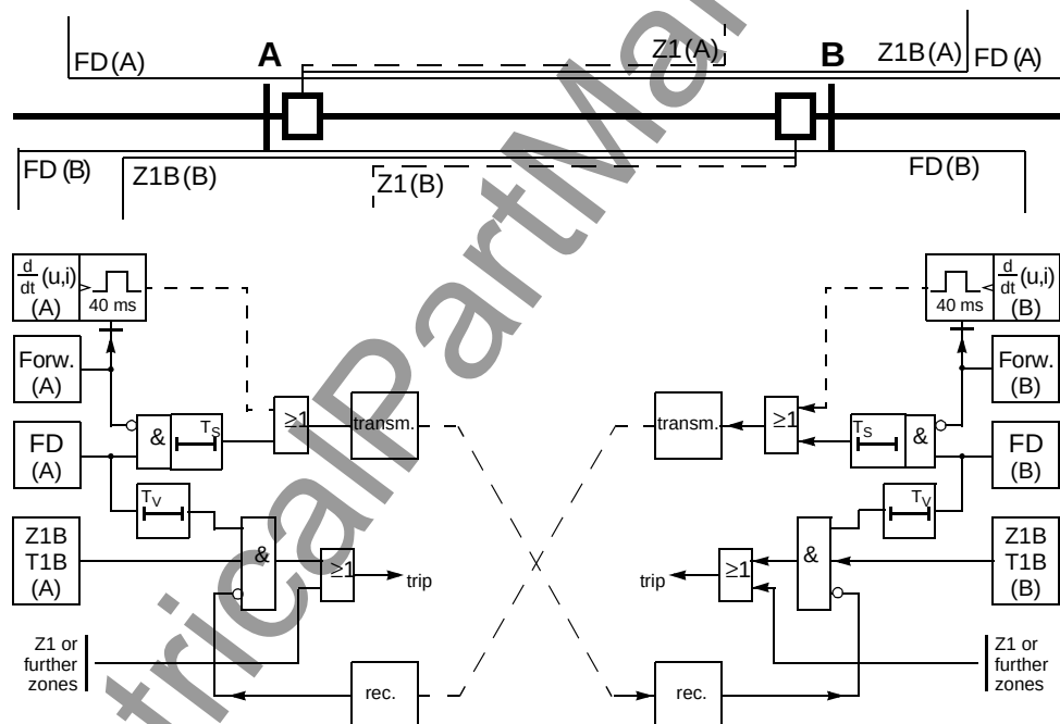
Figure 6-54 Operation scheme of the blocking method
