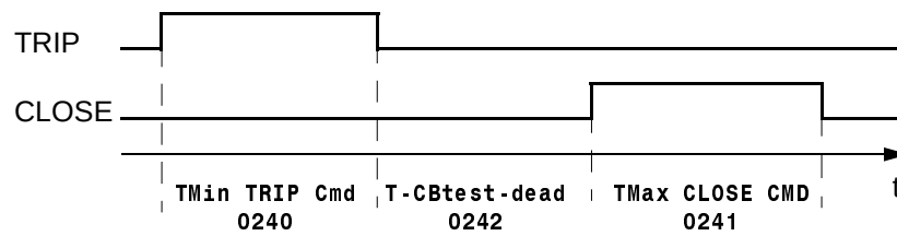
Figure 6-147 Trip/Close test cycle
