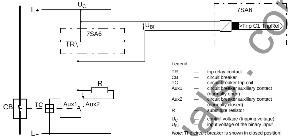
Figure 6-136 Operating principle of the trip circuit supervision with one binary input
