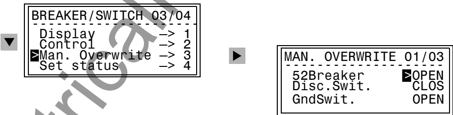
Figure 7-50 Manual Overwriting for Switching Devices from the Front Panel
