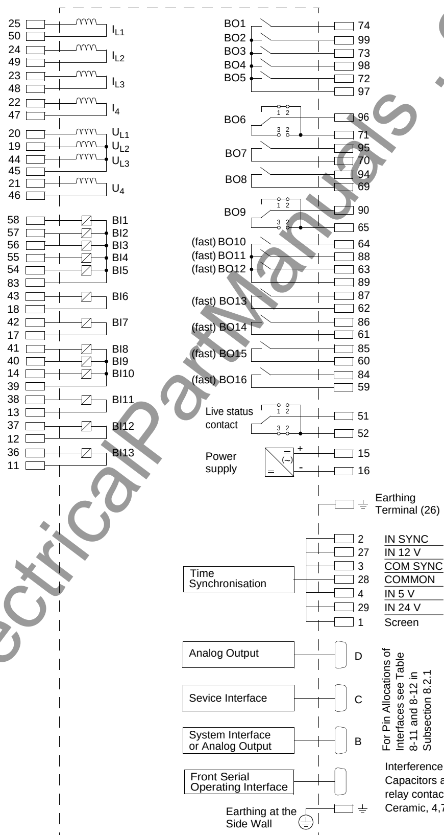
Figure A-10 General Diagram 7SA6*1*-*E (Panel Surface Mounting)
