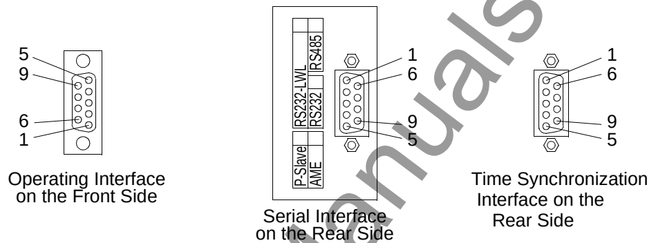
Figure 2-19 9 pin D-subminiature connectors
