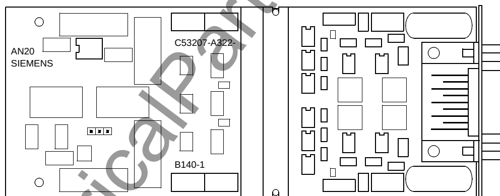
Figure 8-20 Interface module with the analog output AN20
