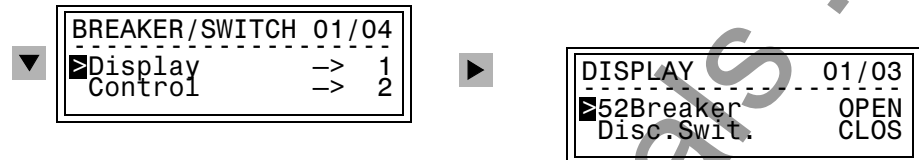
Figure 7-45 Display of Switch Positions in the HMI (example)
