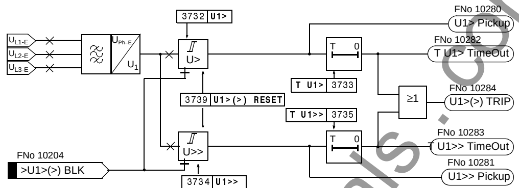
Figure 6-106 Logic diagram of the overvoltage protection for the positive sequence voltage system
