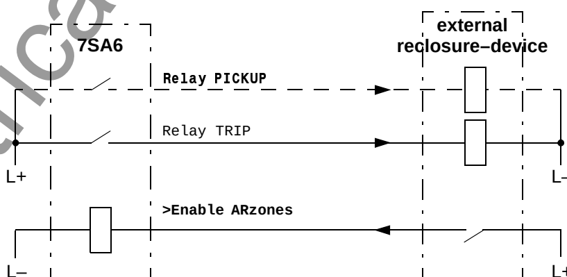
Figure 6-98 Connection example with external reclosure device for 3-pole reclosure
