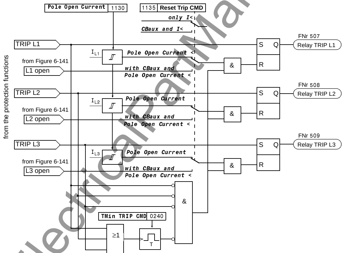
Figure 6-142 Latching and reset of the trip command
