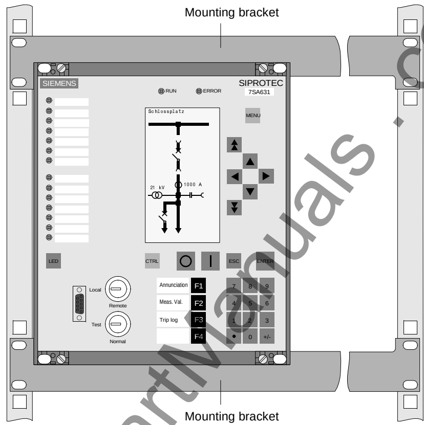
Figure 8-5 Installing a 7SA631 with graphic display in a rack or cubicle (housing width 1\frac{1}{2} of 19 inch rack) as an example
