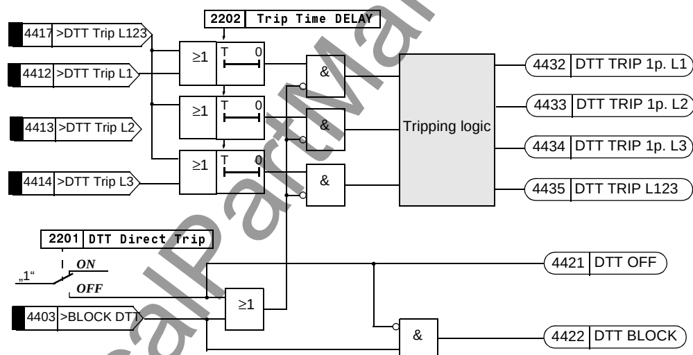
Figure 6-82 Logic diagram of the local external tripping
