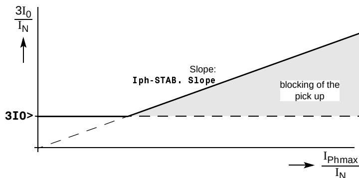
Figure 6-65 Phase current stabilization
