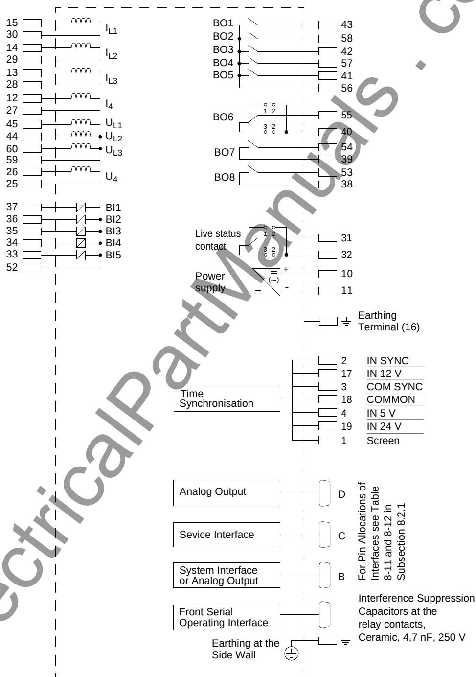
Figure A-8 General Diagram 7SA610*—*E (Panel Surface Mounting)
