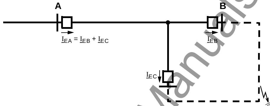
Figure 6-80 Possible unfavourable current distribution on a three terminal line during an external earth fault.
