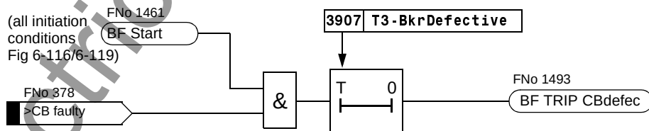
Figure 6-123 Circuit breaker not operational
