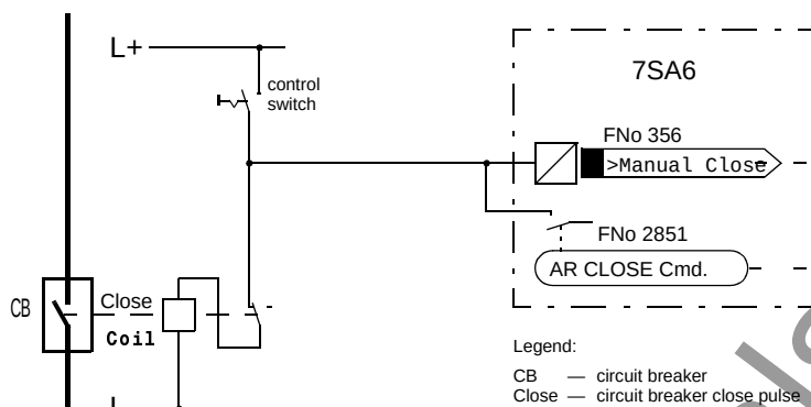
Figure 6-139 Manual closure with internal automatic reclosure
