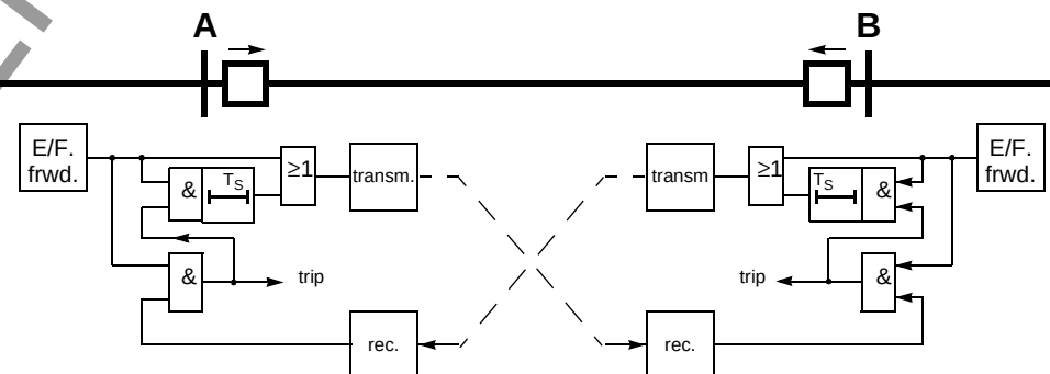
Figure 6-71 Operation scheme of the directional comparison method
