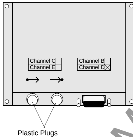
Figure 2-30 Inclined housing with 9 pin D-subminiature connectors
