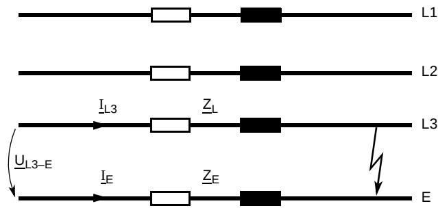
Figure 6-24 Short circuit of a phase-earth loop
