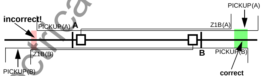
Figure 6-60 Distance protection setting with permissive overreach schemes
