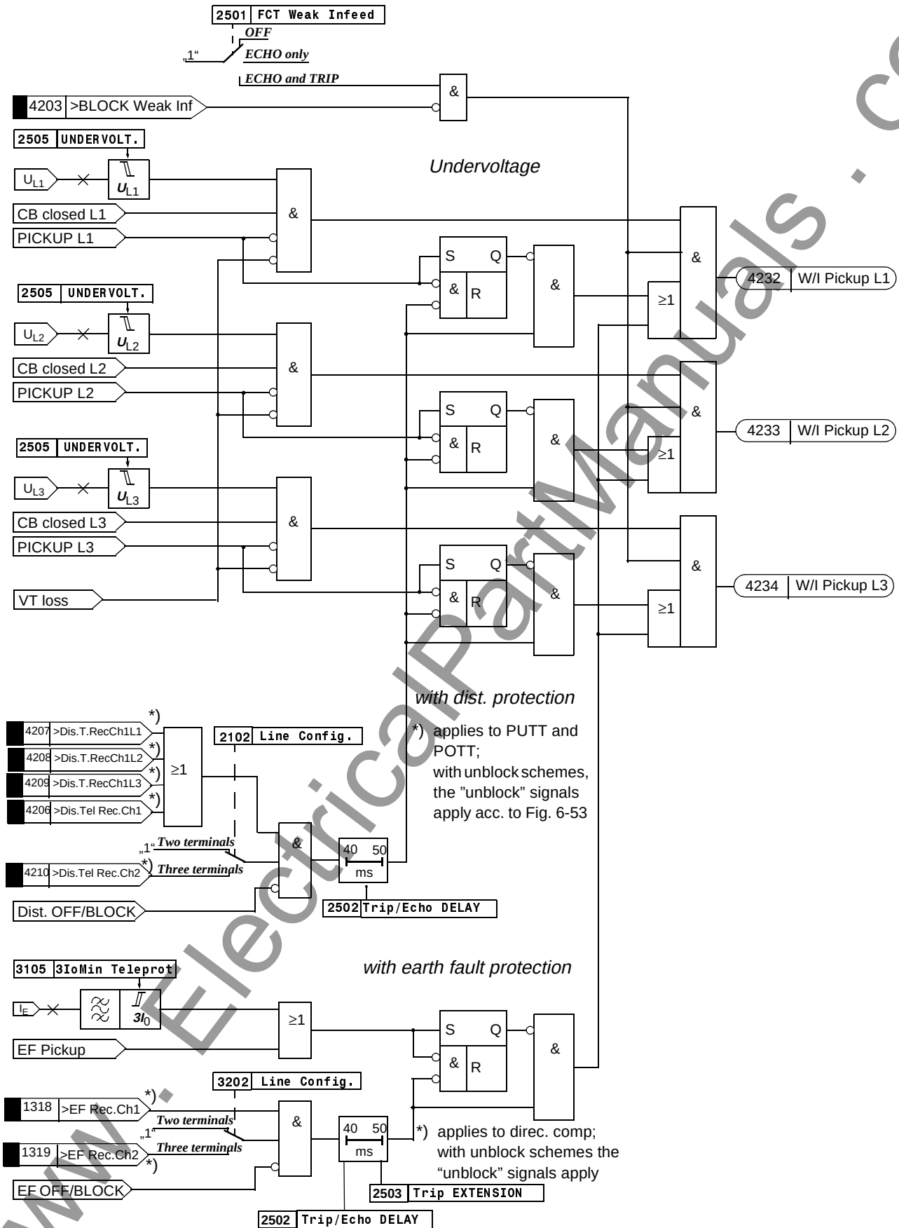
Figure 6-81 Logic diagram of the weak infeed tripping
