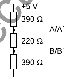
Figure 8-12 Termination of the RS 485 interface (external)
