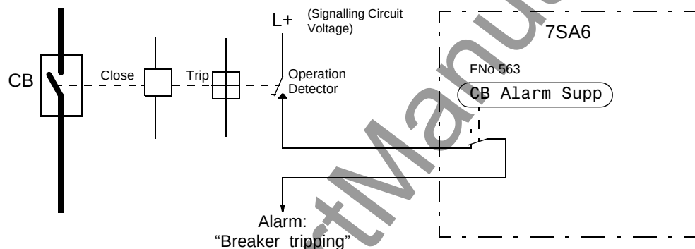
Figure 6-144 Breaker tripping alarm suppression
