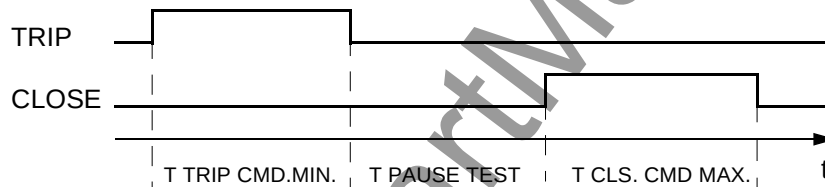
Figure 7-41 TRIP-CLOSE test cycle
