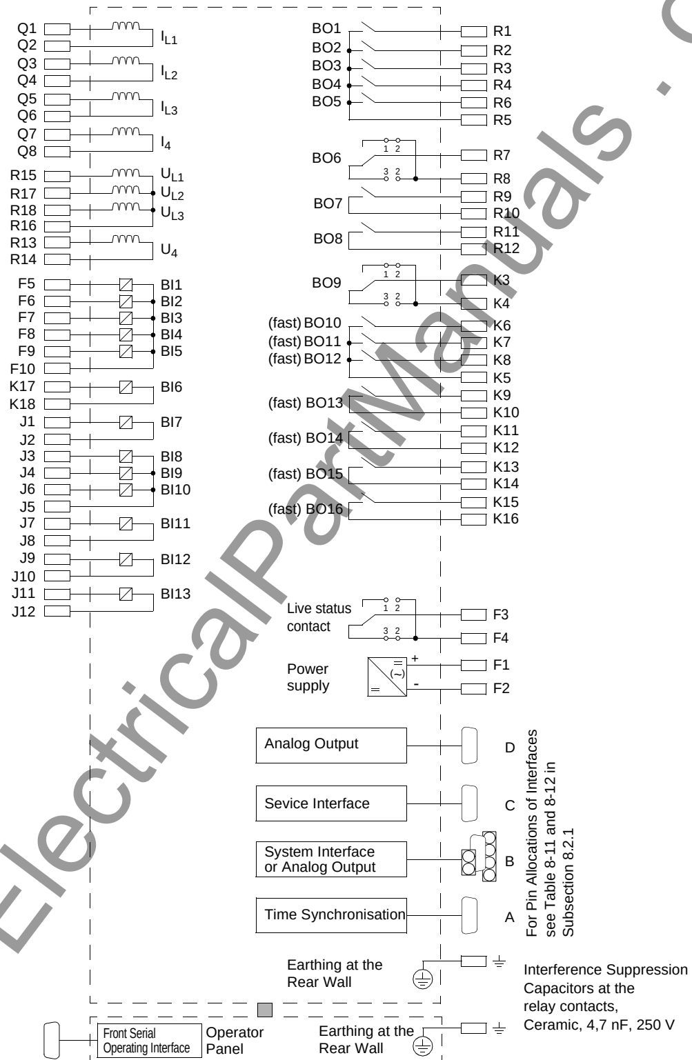
Figure A-15 General Diagram 7SA641*--*A/J (Mounting with detached operator panel)
