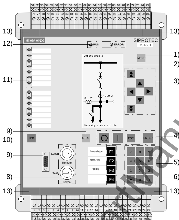
Figure 2-24 Front view of a 7SA63, housing size 1 / 2 , for panel surface mounting without optical communication interfaces
