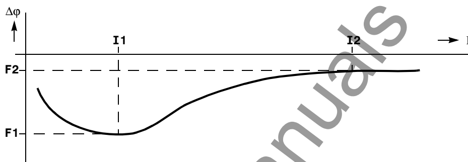
Figure 6-92 Settings for the phase angle correction
