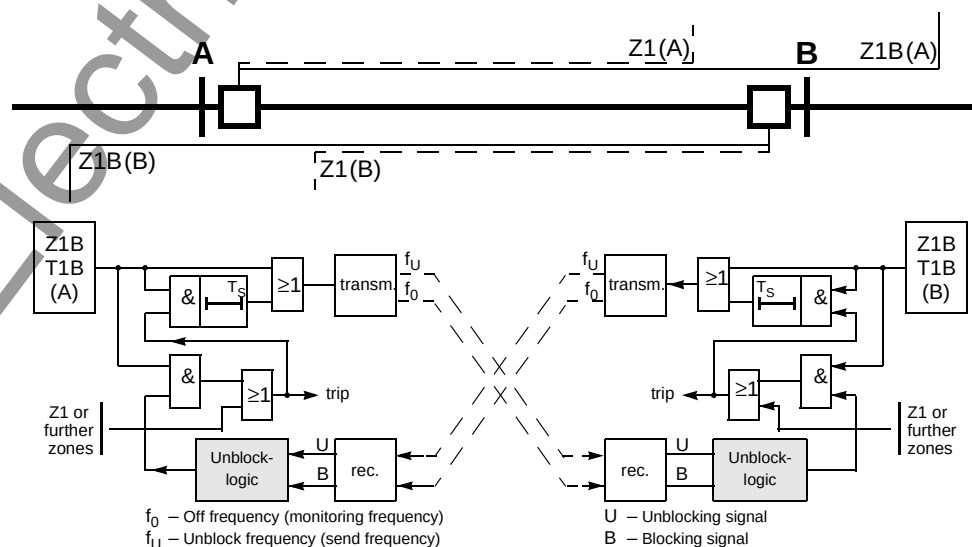
Figure 6-51 Operation scheme of the unblocking method with Z1B
