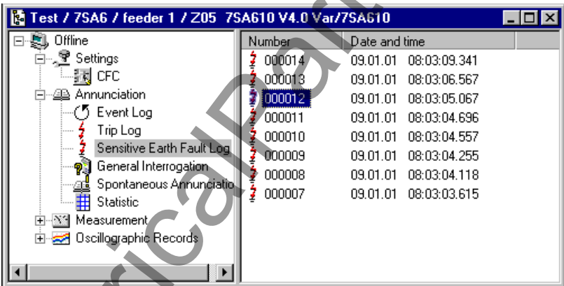
Figure 7-11 DIGSI® 4 Selection of Earth Fault Log with a Fault Indicated in the Data Window
