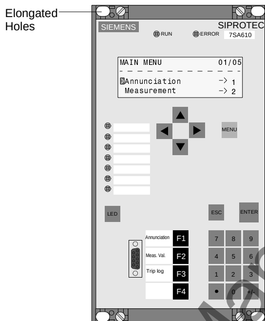
Figure 8-1 Panel mounting of a 7SA610 with a four-line display (housing width 1\frac{1}{3} ) as an example
