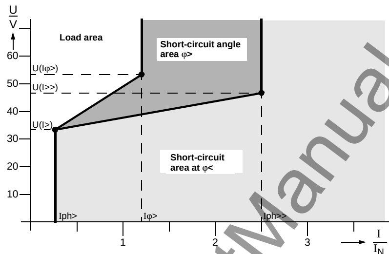
Figure 6-20 U/I/φ characteristic
