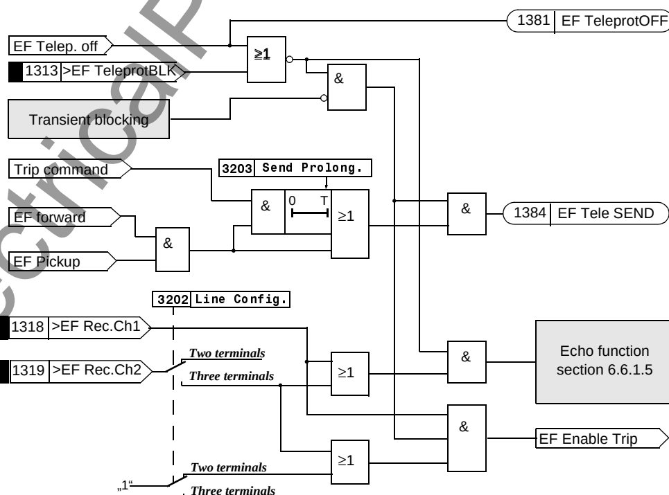
Figure 6-72 Logic diagram of the directional comparison scheme (one line end)
