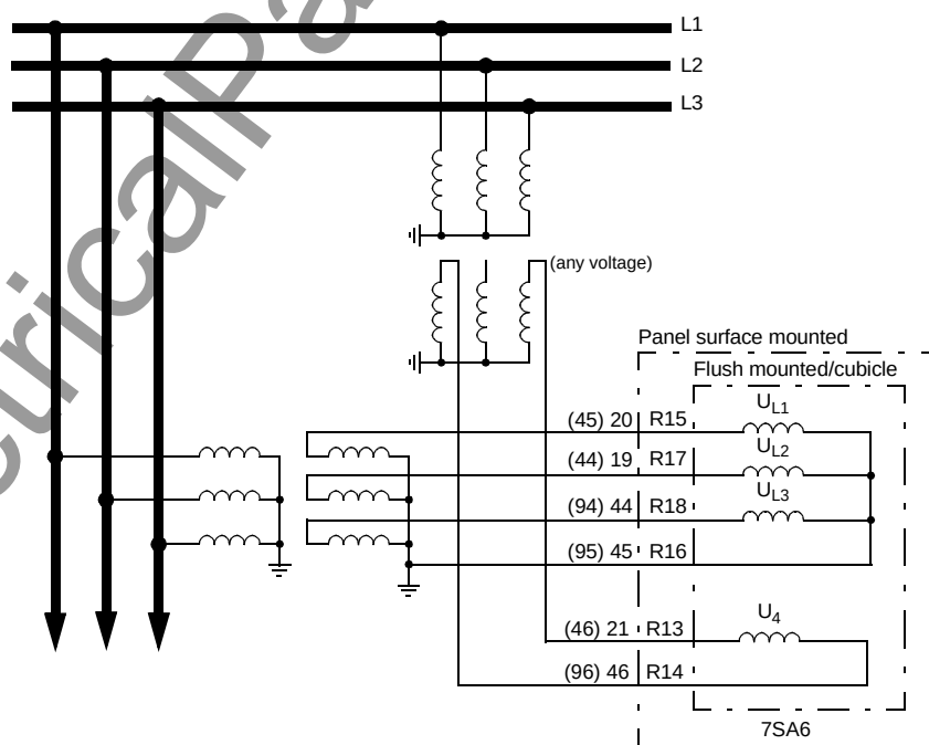
Figure A-27 Voltage connections to three Wye-connected voltage transformers and additionally to any phase-to-phase voltage (for overvoltage protection and/or synchronism check)
