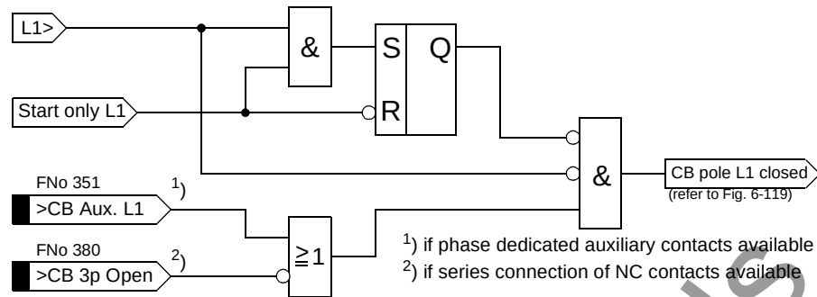
Figure 6-114 Interlock of the auxiliary contact criterion — example for phase L1
