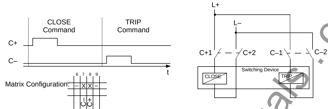
Figure 5-13 Single command with 2 outputs via 2 power relays with 2 contacts each (setting: "Double Command with Single Output") - example
