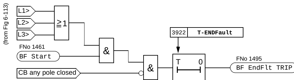
Figure 6-125 Function block diagram of end fault protection
