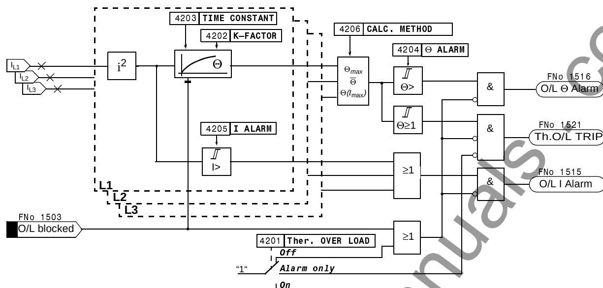
Figure 6-129 Logic diagram of the thermal overload protection
