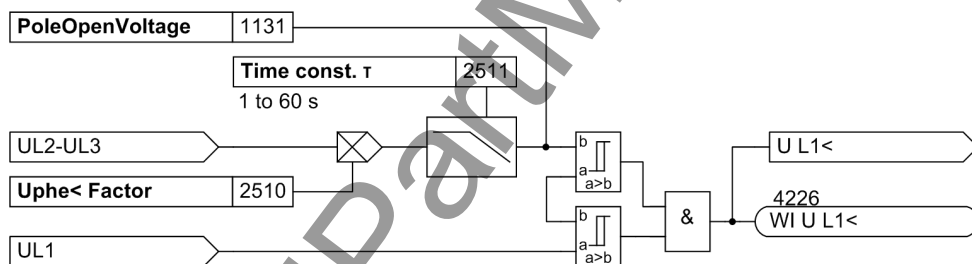
Figure 2-114 Undervoltage detection for U_{L1-E}
