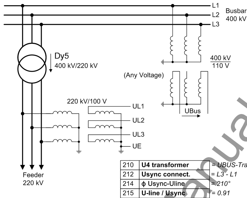
Figure 2-3 Busbar voltage measured via transformer
