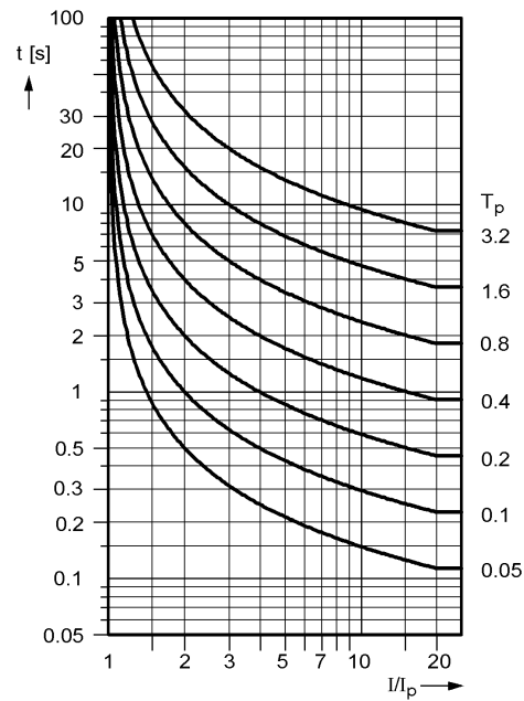
Normal inverse: (Type A)
