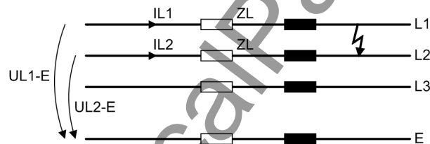
Figure 2-33 Short-circuit of a phase-phase loop
