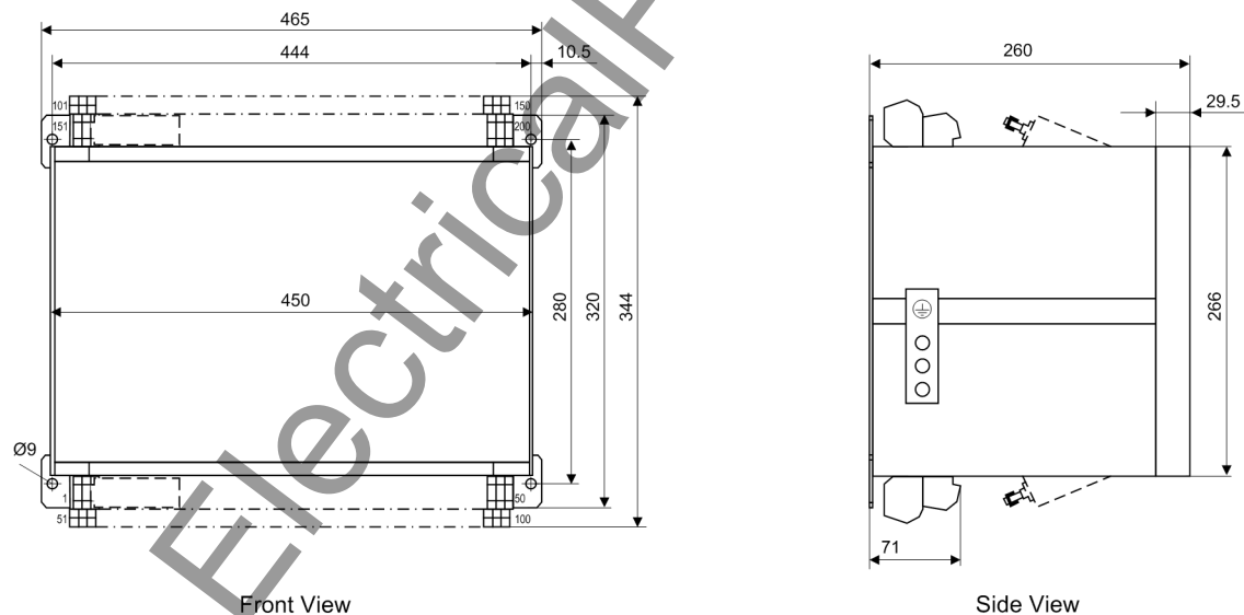
Figure 4-11 Dimensions of a device for panel surface mounting (size 1/1 )
