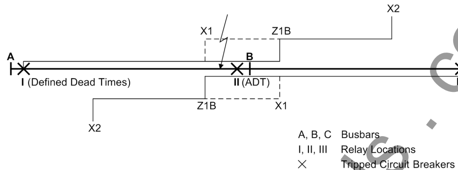
Figure 2-123 Example of adaptive dead time (ADT)
