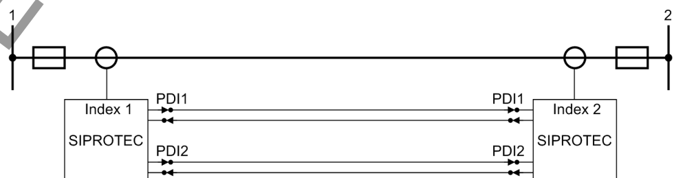
Figure 2-8 Differential protection for two ends with two 7SD5 each of them having two protection data interfaces (transmitter/receiver)
