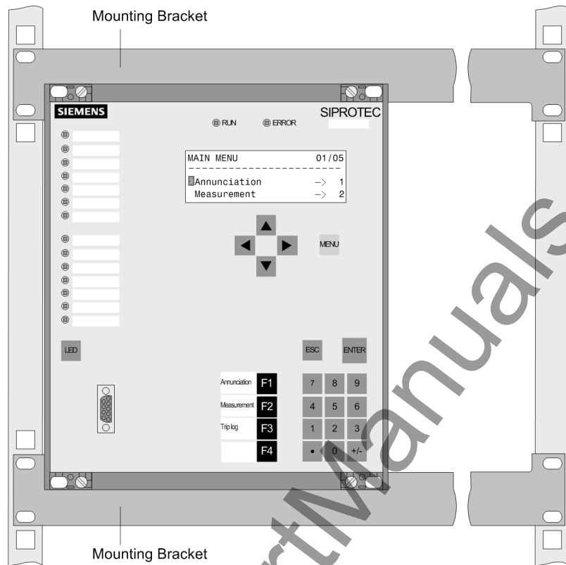
Figure 3-15 Example of rack or cubicle mounting of a device (housing size 1/2 )
