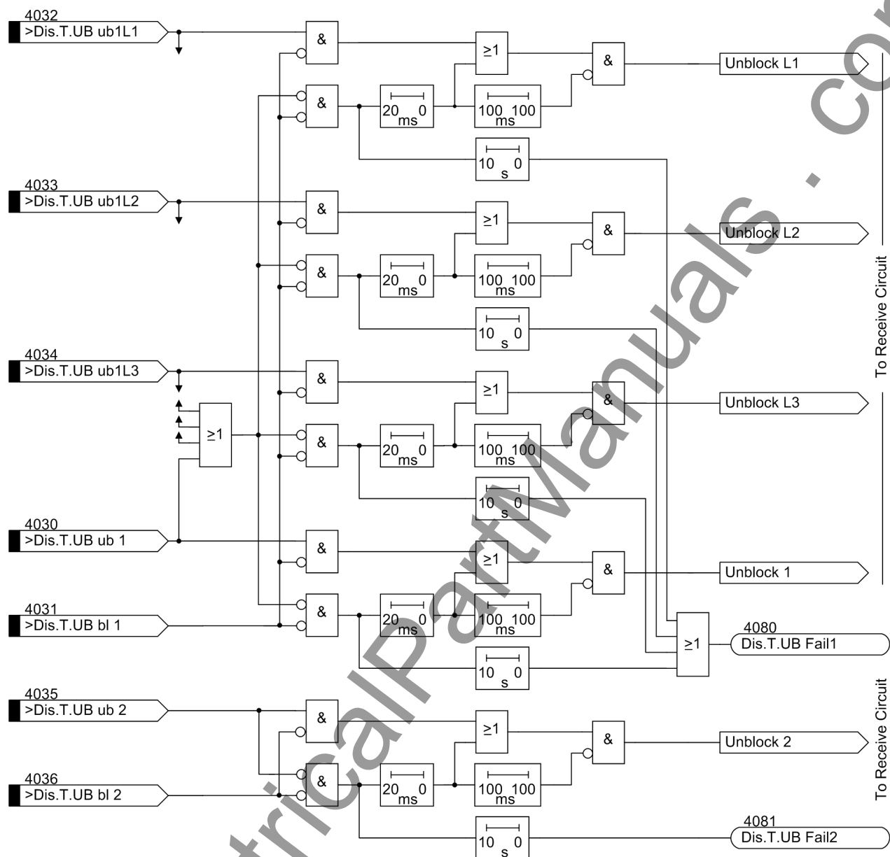
Figure 2-78 Unblock logic
