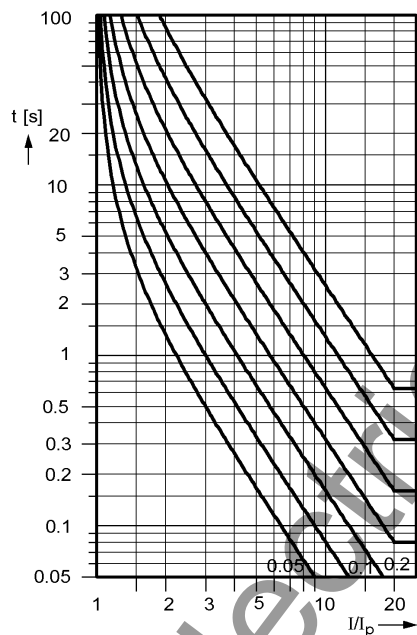
Extremely inverse: (Type C)
