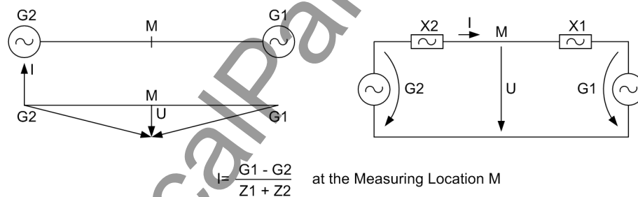
Figure 2-60 Power swing
