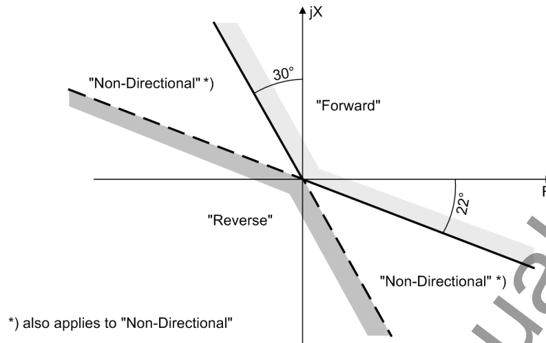
Figure 2-43 Directional characteristic in the R-X-diagram
