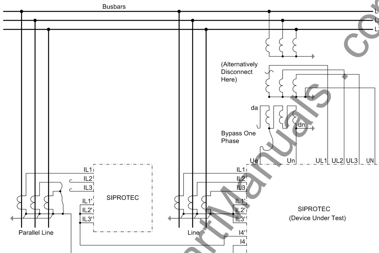
Figure 3-31 Polarity check of I_4 , example with earth current of a parallel line
