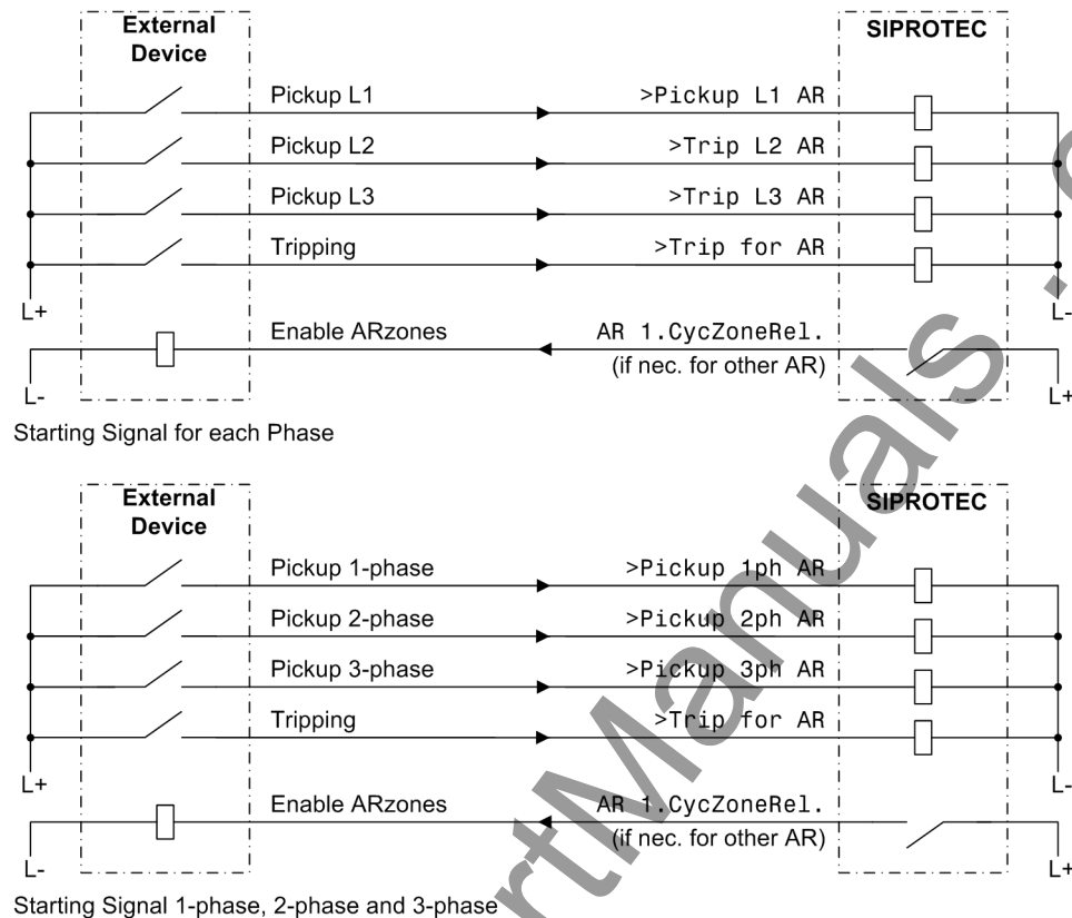
Figure 2-128 Connection example with external protection device for fault detection dependent dead time — dead time control by pickup signals of the protection device; AR control mode = with PICKUP
