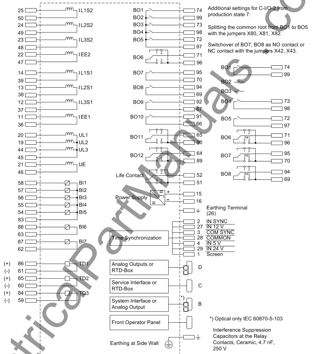
Figure A-3 General Diagram for 7UM621/623*-*B (panel surface mounting)
