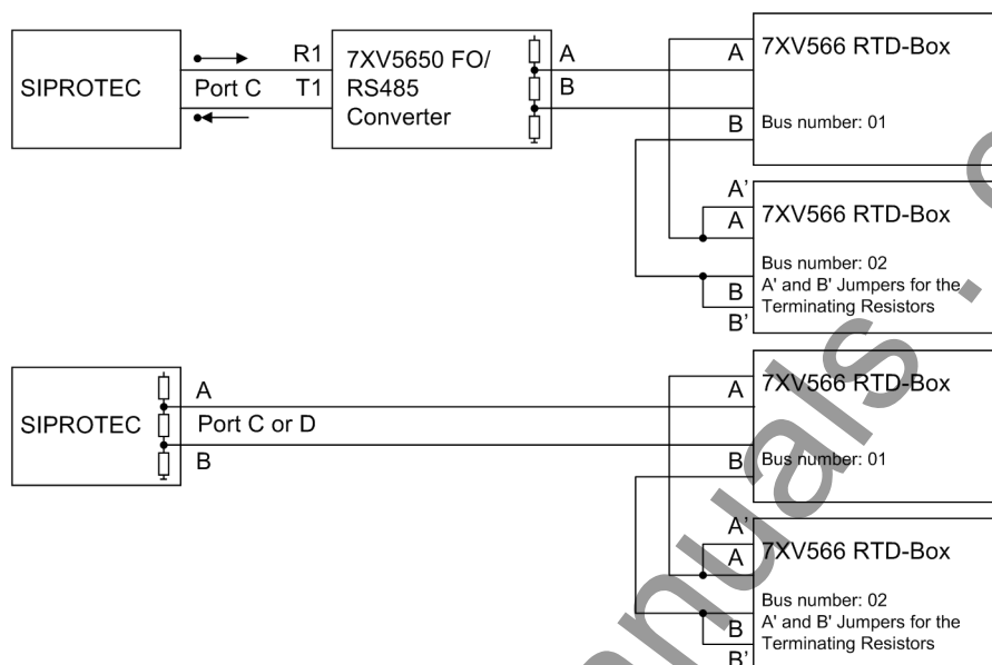
Figure A-21 Semiduplex operation with two thermoboxes above: optical design (2 FOs) below: design with RS485
