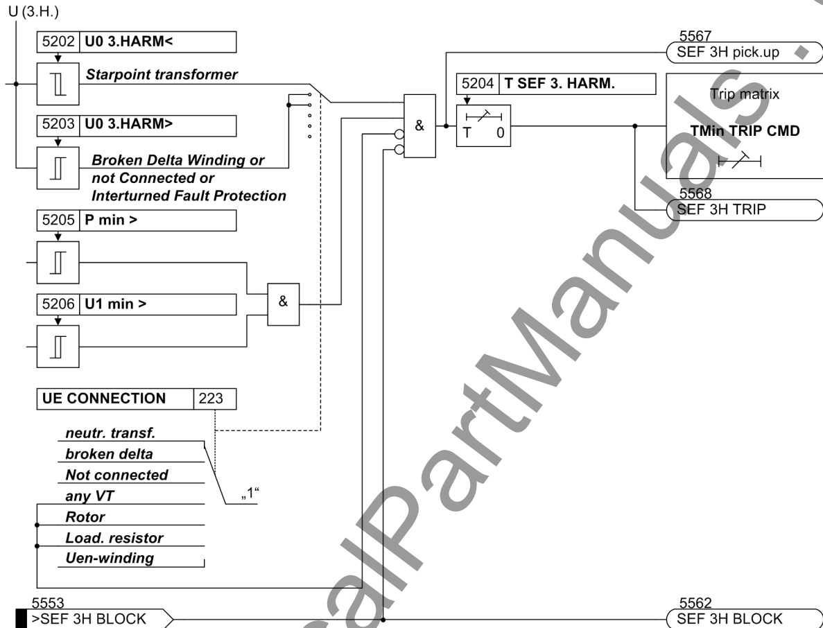
Figure 2-92 Logic Diagram of 100% Stator Earth Fault Protection
