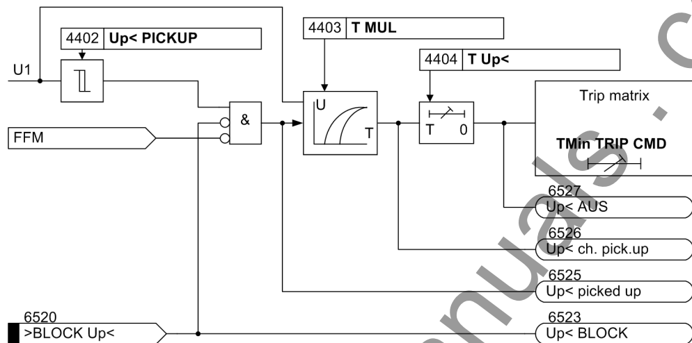
Figure 2-77 Logic Diagram of the Inverse-Time Undervoltage Protection
