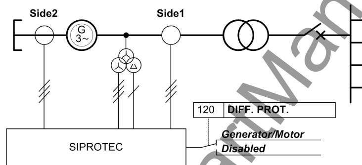
Figure 2-2 Use as Generator Differential Protection
