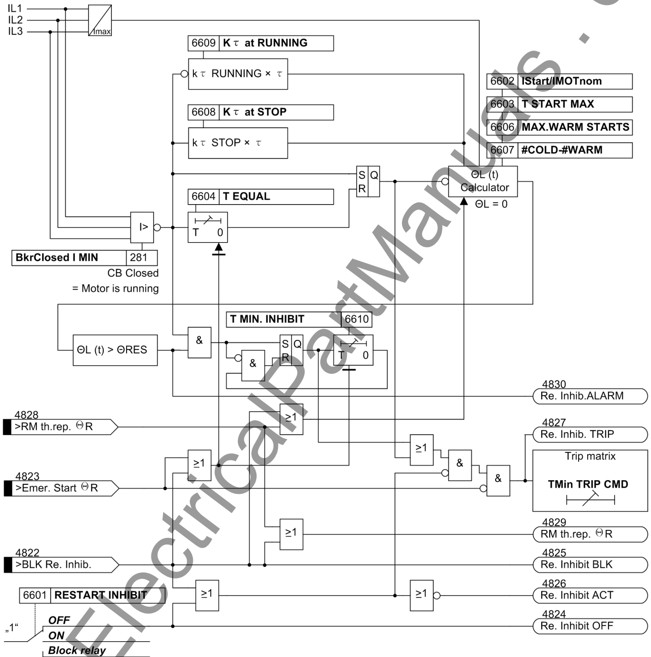
Figure 2-115 Logic diagram of the Restart Inhibit
