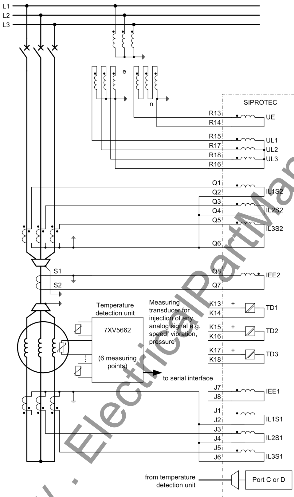
Figure A-12 Synchronous motor: Connection to three voltage transformers (phase-to-earth voltages, usually from the busbar); Displacement voltage detection at broken delta winding, and three current transformers on each side; Earth fault direction detection using toroidal CTs
