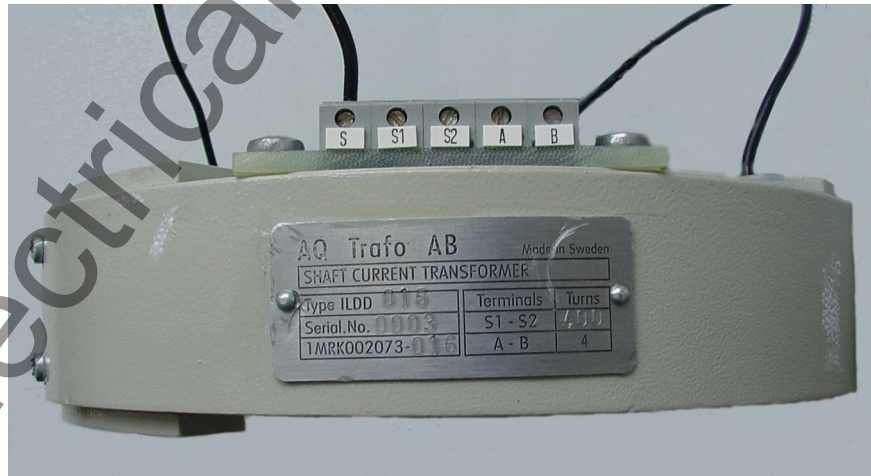
Figure 2-100 Terminals of the shaft current transformer
