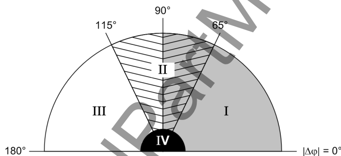
Figure 2-49 Operating ranges of the direction criterion
