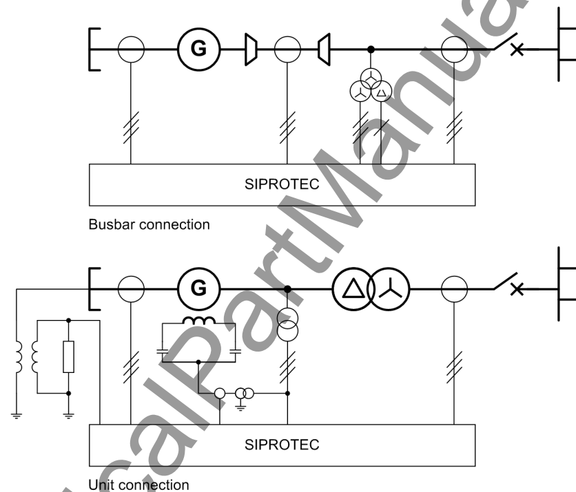
Figure 1-2 Typical Connections
