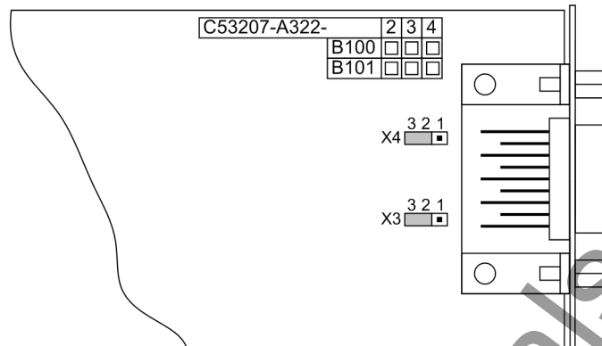
Figure 3-11 Position of the Plug-in Jumpers for the Configuration of the Terminating Resistors at the Profibus (FMS and DP), DNP 3.0 and Modbus Interfaces
