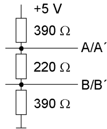
Figure 3-4 Termination of the RS485 interface (external)
