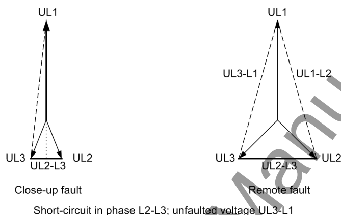
Figure 2-12 Cross-Polarized Voltages for Direction Determination
