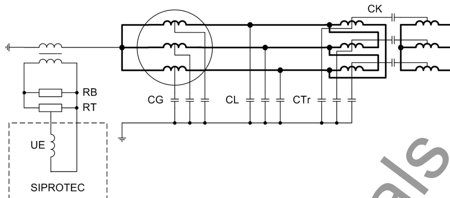
Figure 2-82 Unit Connection with Earthing Transformer
