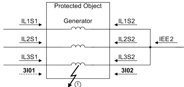
Figure 2-46 Connection scheme and definition of current vectors
