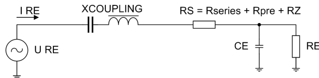
Figure 2-107 Equivalent Measuring Circuit for Rotor Earth Fault Protection where:
