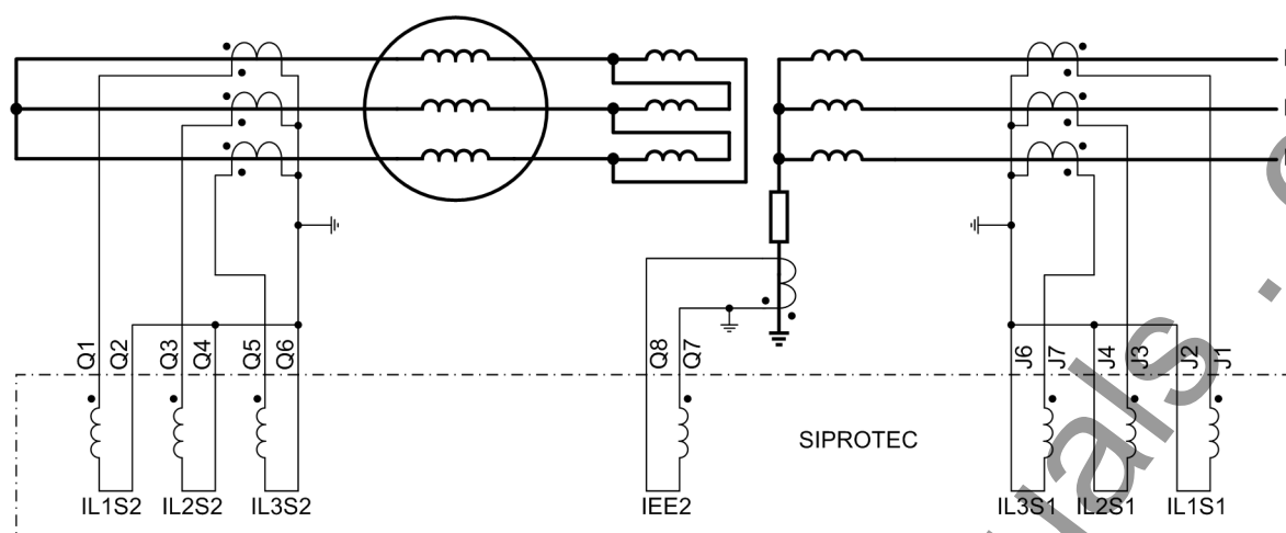
Figure A-18 Earth current differential protection (generator)
