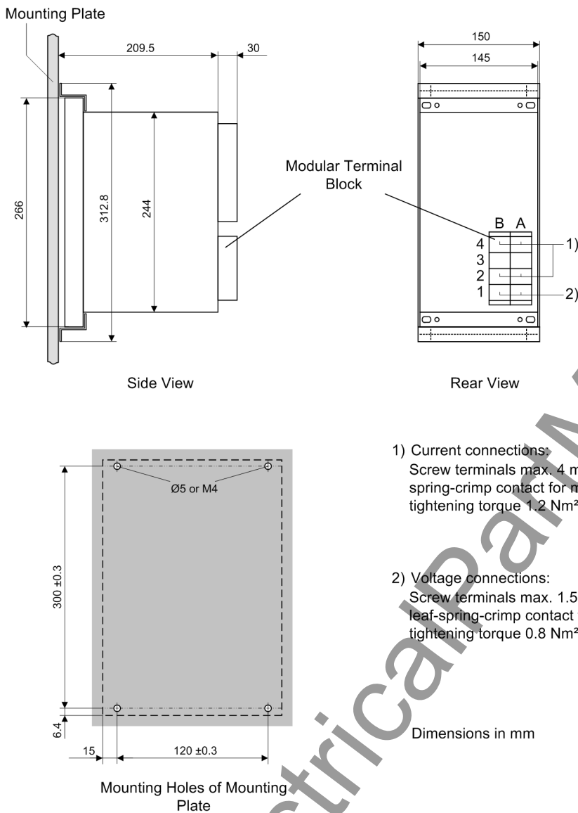
Figure 4-19 Dimensions of Coupling Unit 7XR6100-0BA0 for Panel Surface Mounting
