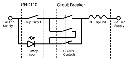
Figure 2 - Trip Circuit Supervision Scheme
