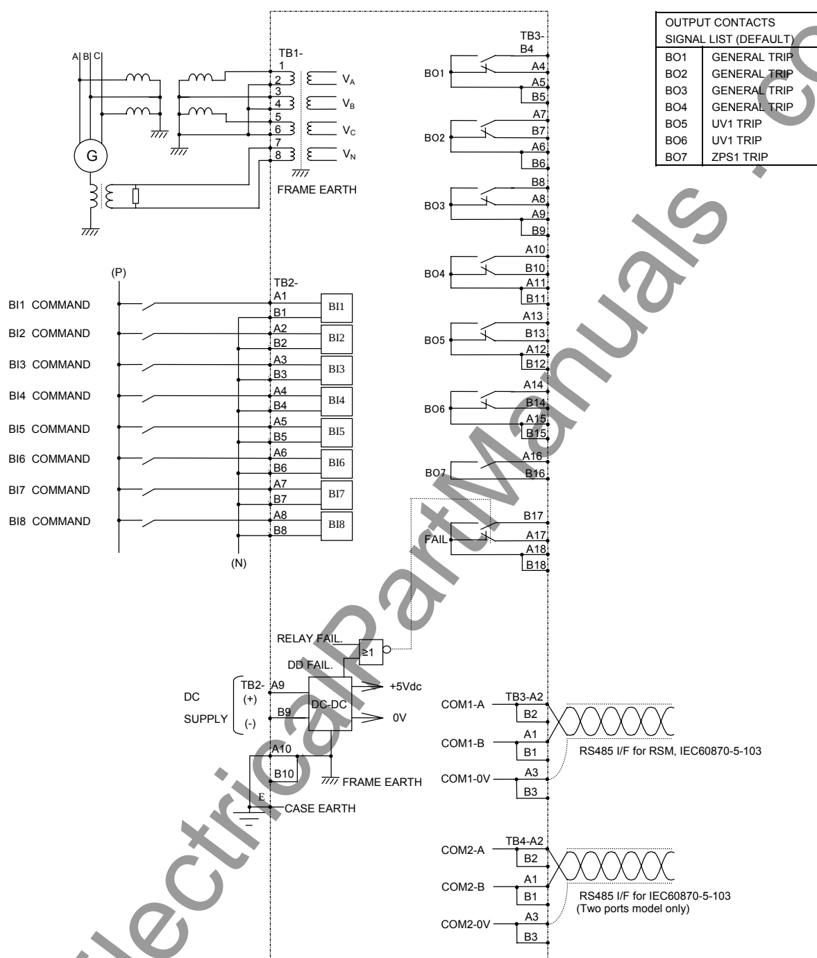
Figure 8 - GRD130-410 Typical Application Diagram for Two Phase VT Connection with Residual Voltage Measured by Earthing Transformer
