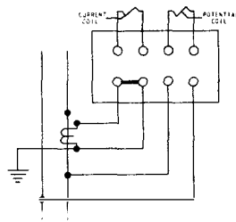
Fig. 10 Back-View Connection of Test Block for One Current and One Potential Coil
