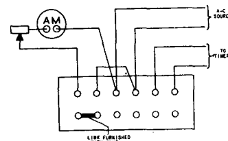
Fig. 16 Plug Connection for Fig. 11 for Separate Test of Relay With Separate Source
