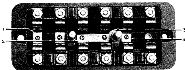
Fig. 3 Six-Pole Test Block With Jumper and Auxiliary Contacts
