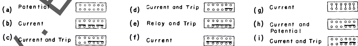
Fig. 8 Internal Connections of Four-Pole Block
