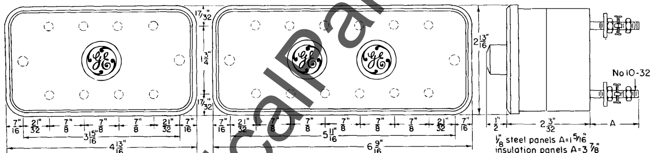
Fig. 4 Outline Dimensions of Four-Pole and Six-Pole Test Blocks
