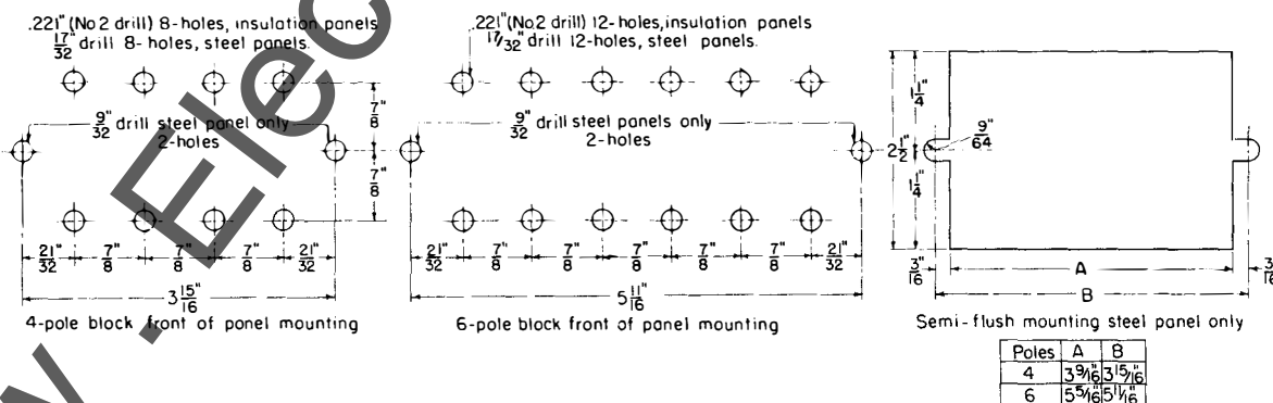
Fig. 5 Panel-Drilling Dimensions of Four-Pole and Six-Pole Test Blocks
