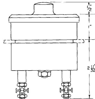
Fig. 2 Semi-Flush Mounting on 1/8-inch Steel Panel
