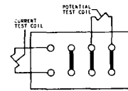
Fig. 13 Back-View Connection of Plug for Testing One Current and One Potential Coil In Circuit
