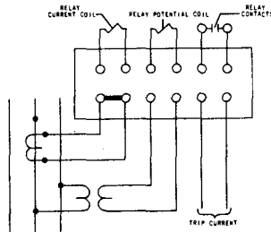
Fig. 11 Test-Block for One Current and One Potential Coil With Connections for Trip Circuit
