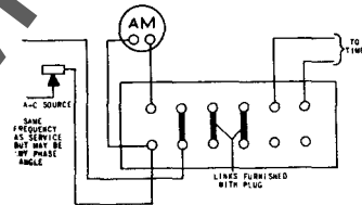
Fig. 15 Plug Connections for Fig. 11 for Testing Relay With Same or Separate Source
