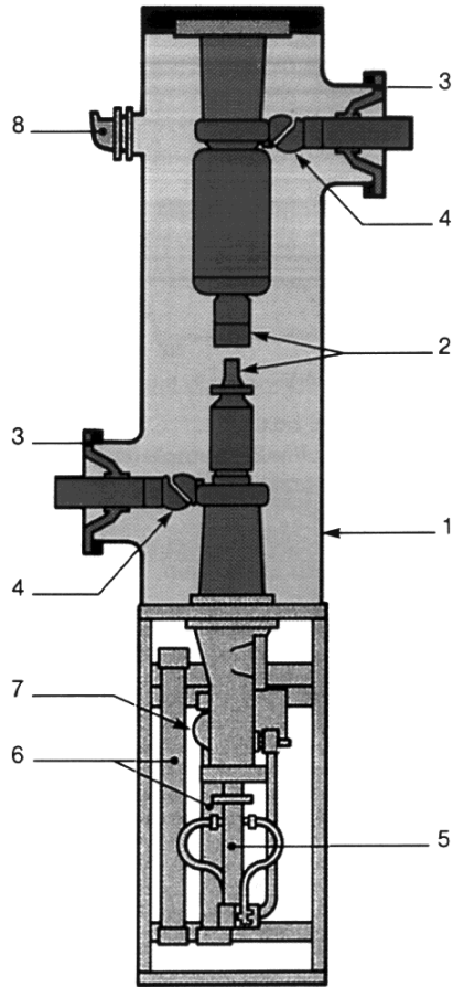
Circuit breaker hydraulic operating mechanism - Schematic diagram
