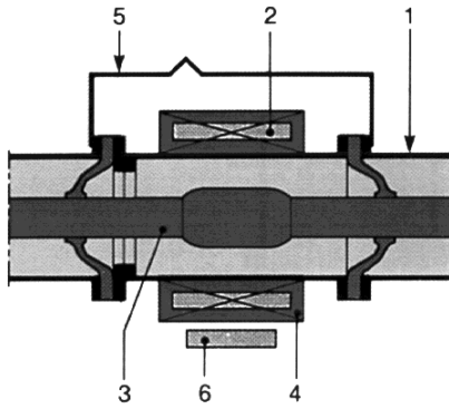
Angular shaft disconnector
