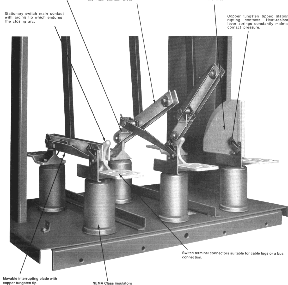
HVL SWITCH AS VIEWED LESS INTER-PHASE BARRIERS & COMPLETED ARC CHUTE ASSEMBLIES
