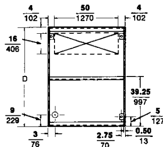
Floor Plan
