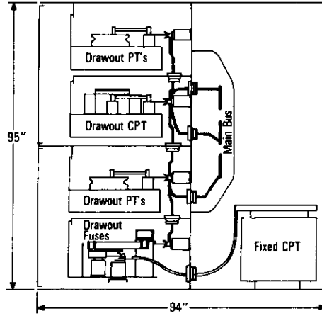
36" Wide Typical Auxiliary/Auxiliary Vertical Section
