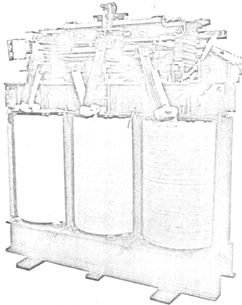
Core and Coils—Liquid-Immersed Type
