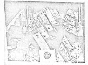
Cutaway of 3-pole selector switch shows blade positions for connection of one incoming line.
