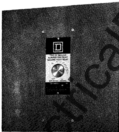
ALTERNATE RELAY MOUNTING WITH NAMEPLATE AND CURRENT ADJUSTMENT ON FRONT OF EQUIPMENT ENCLOSURE
