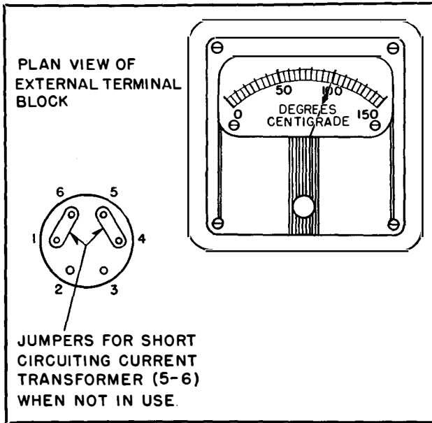
FIG. 4. Dial and Jumper for Short Circuiting Current Transformer When Not in Use.
