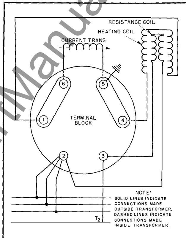
FIG. 2. Front and Rear Connections on Terminal Block.
