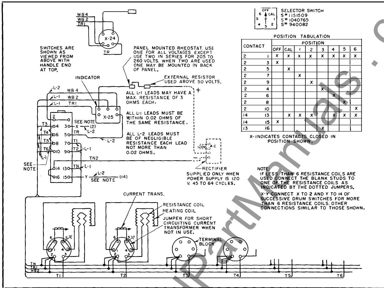
FIG. 3. Wiring Diagram for Temperature Indicator.
